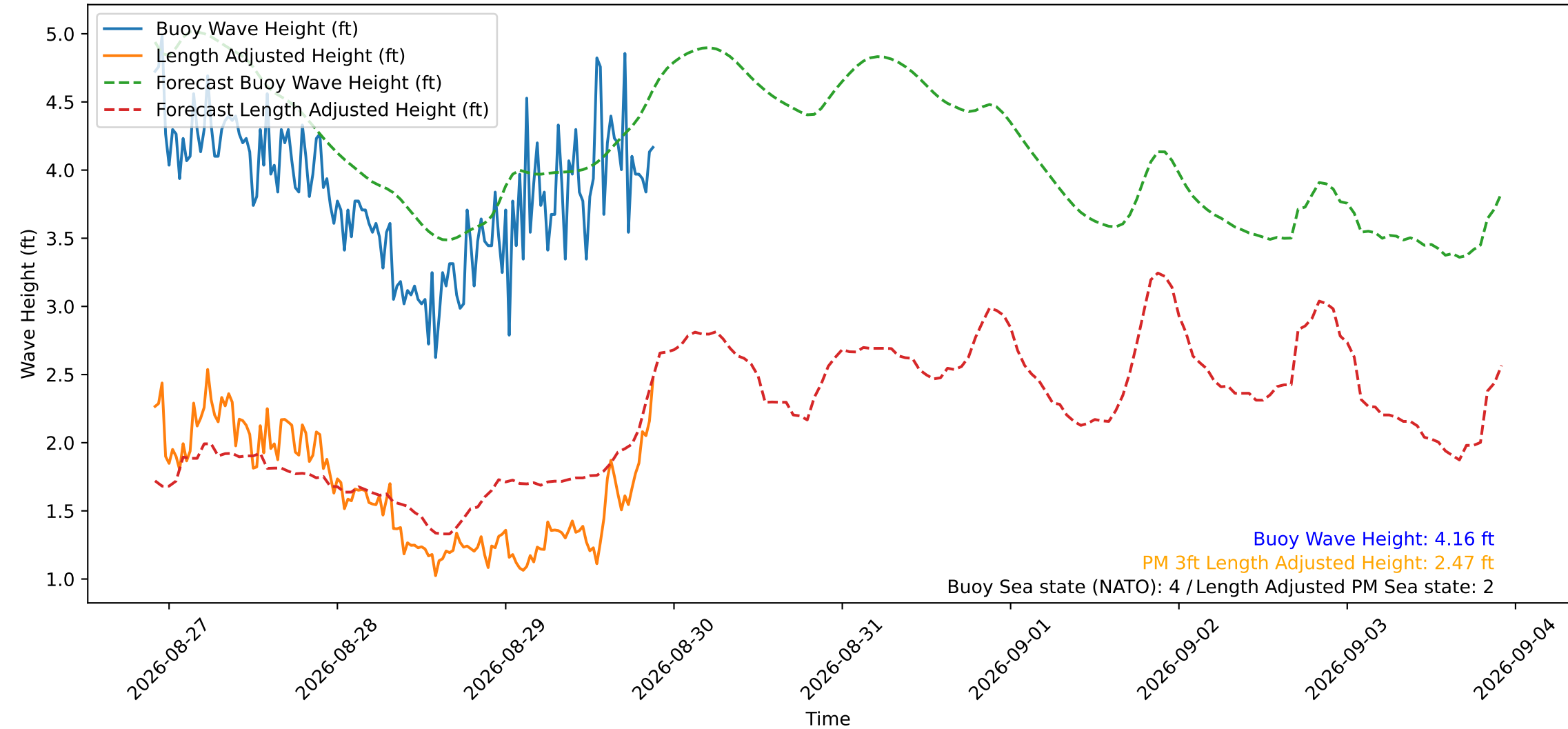
Wave Heights over Time for Green Beach at 2026-08-29 21:51:14
