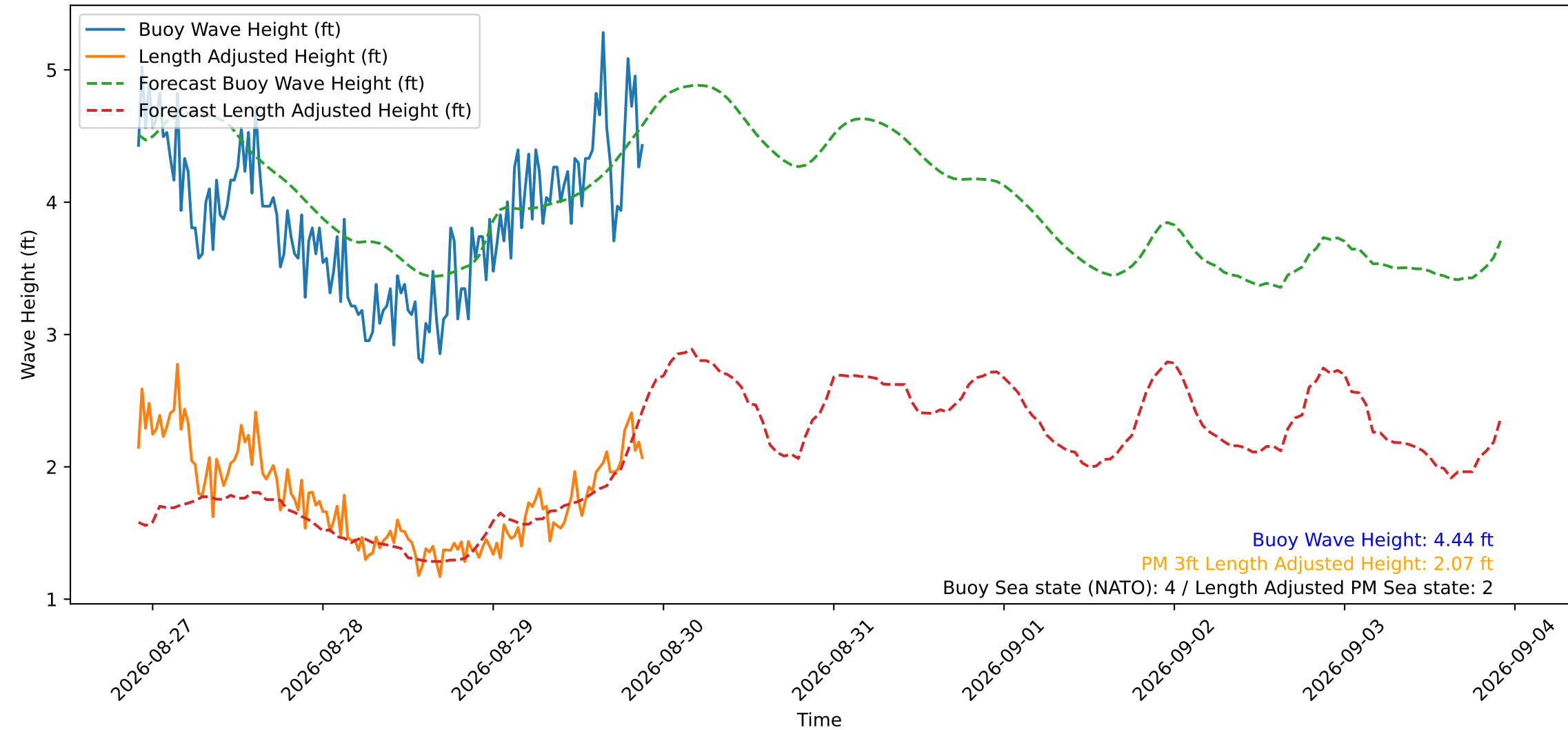
Wave Heights over Time for Oceanside Harbor at 2026-08-29 21:50:29
