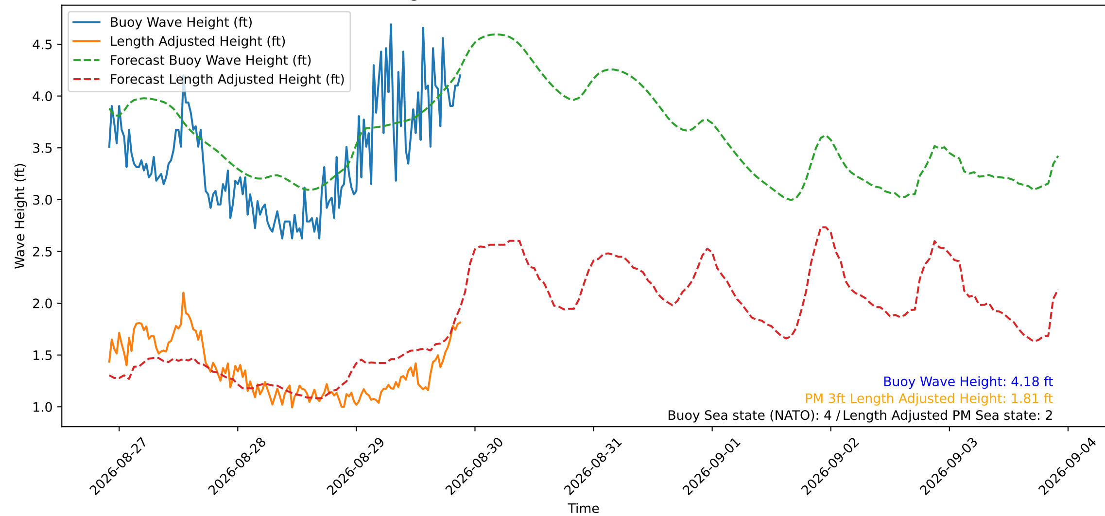
Wave Heights over Time for Red Beach at 2026-08-29 21:50:50
