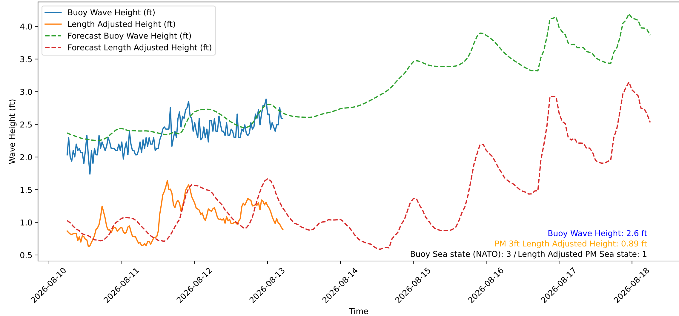
Wave Heights over Time for Red Beach at 2026-08-13 05:50:47
