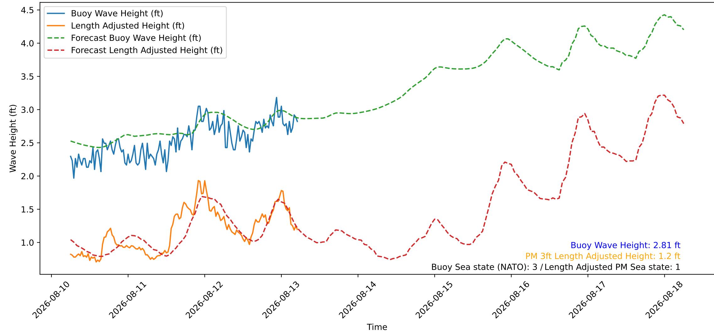
Wave Heights over Time for Oceanside Harbor at 2026-08-13 05:50:26
