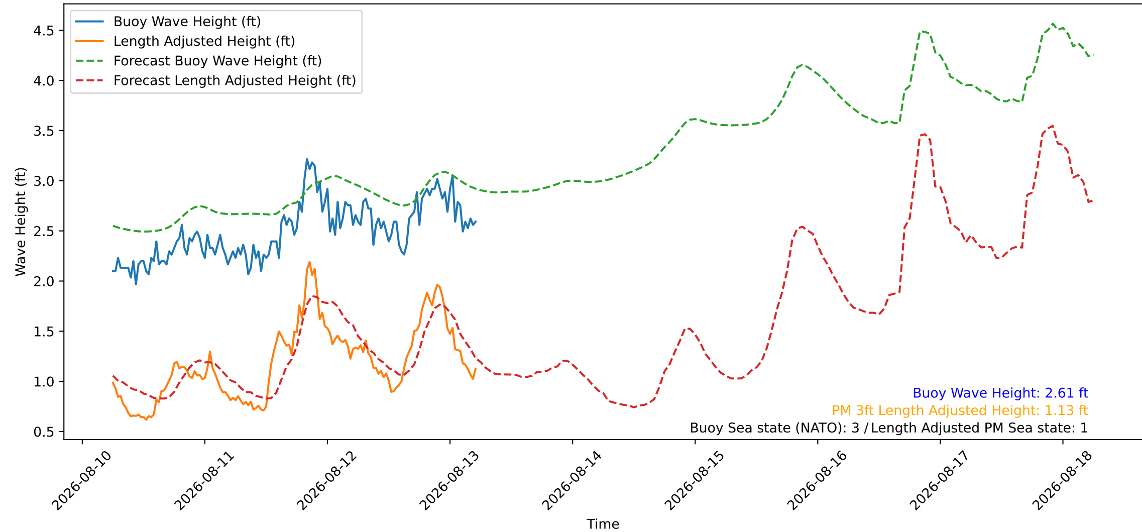
Wave Heights over Time for Green Beach at 2026-08-13 05:51:10
