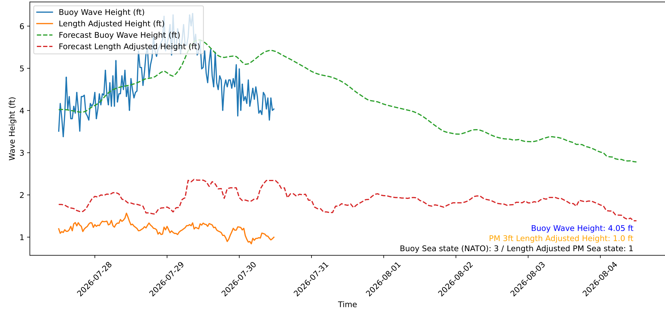
Wave Heights over Time for Green Beach at 2026-07-30 12:11:08
