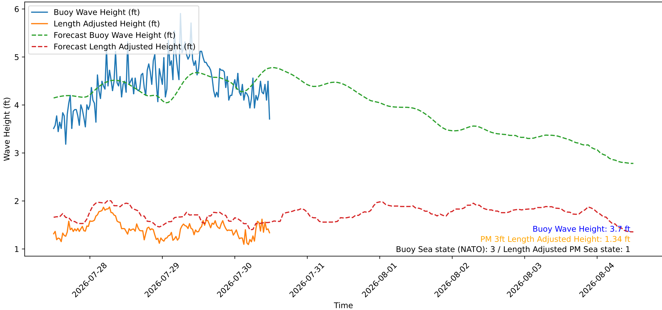
Wave Heights over Time for Oceanside Harbor at 2026-07-30 12:10:26
