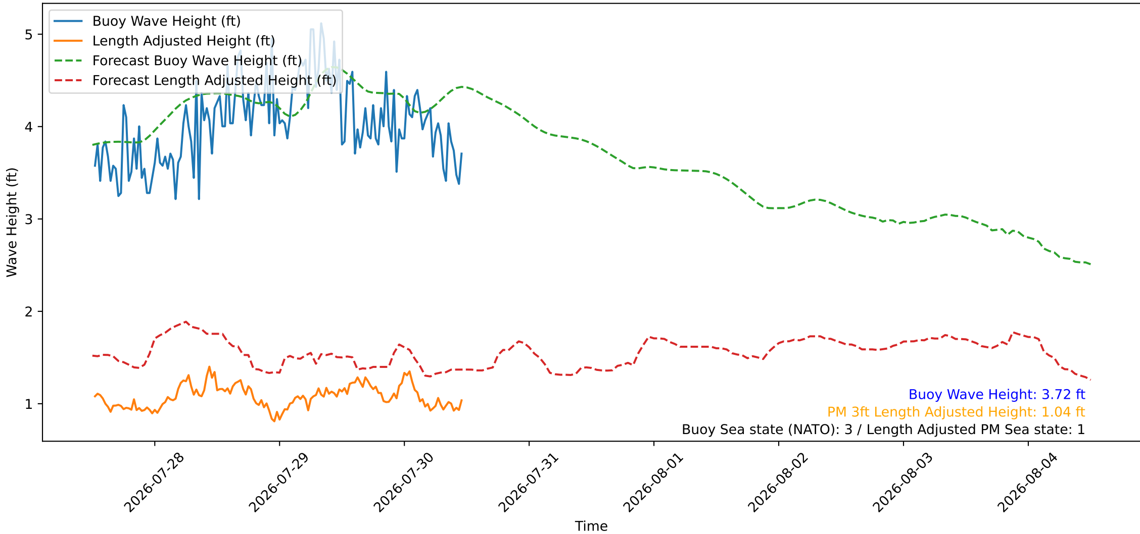
Wave Heights over Time for Red Beach at 2026-07-30 12:10:45
