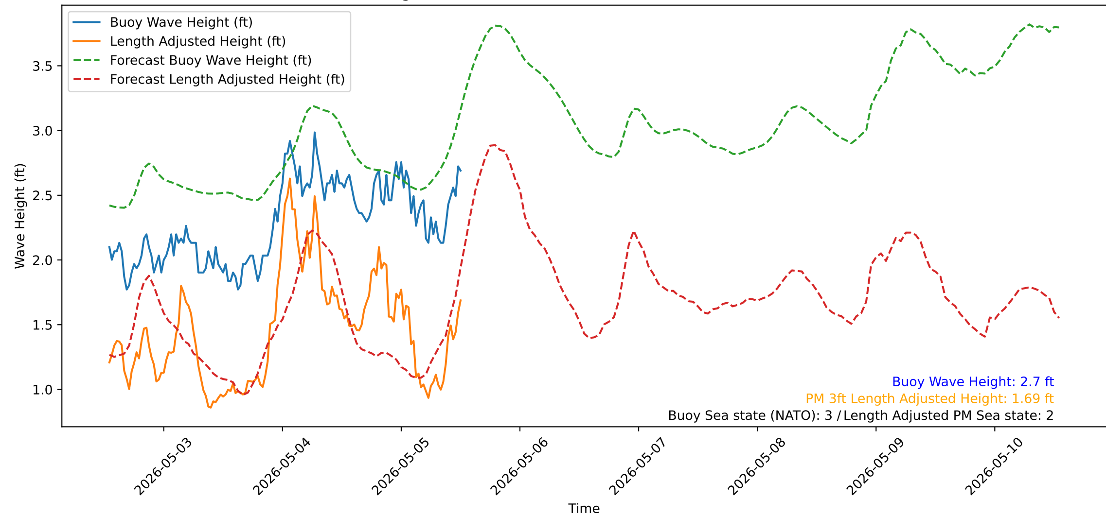
Wave Heights over Time for Green Beach at 2026-05-05 13:01:12
