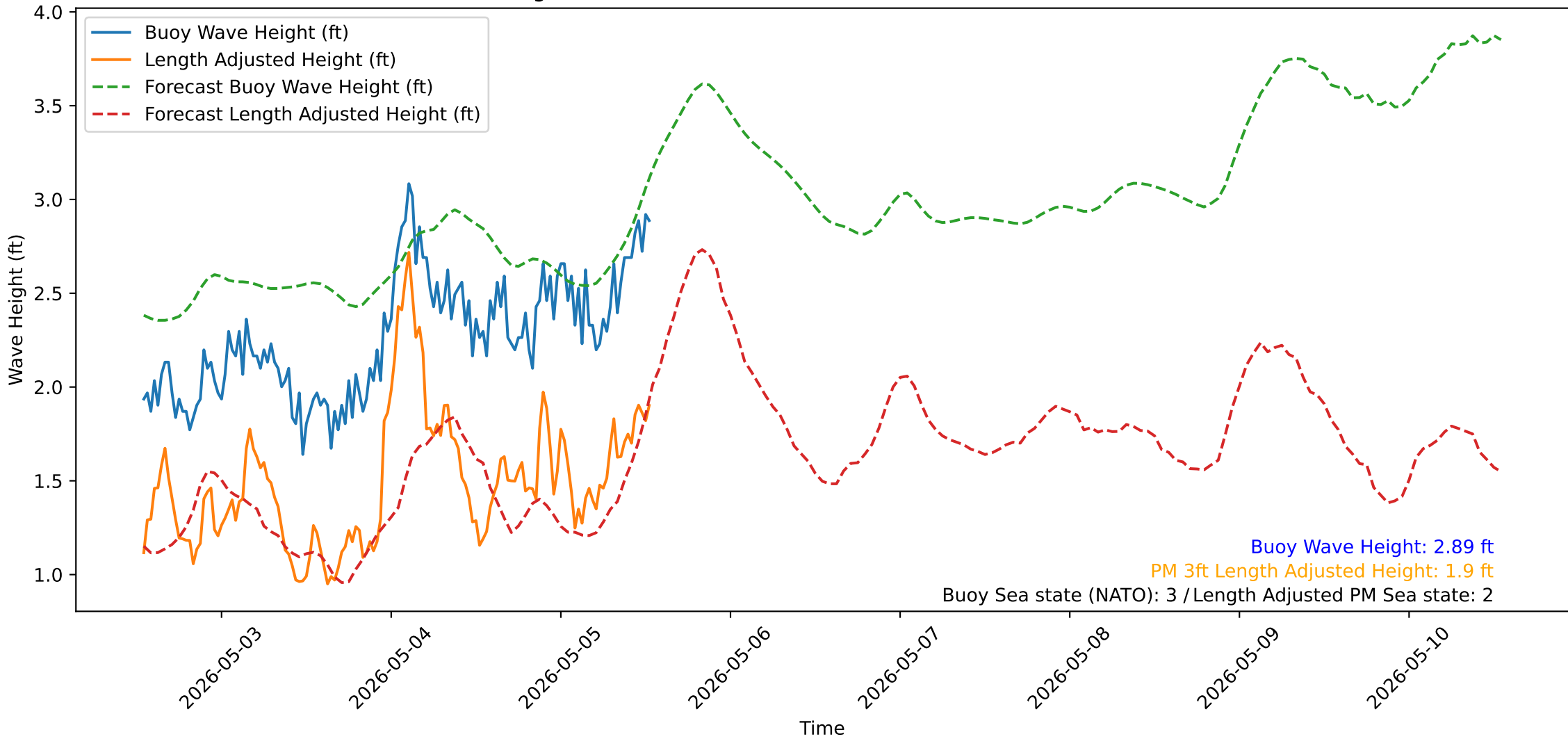
Wave Heights over Time for Oceanside Harbor at 2026-05-05 13:00:31
