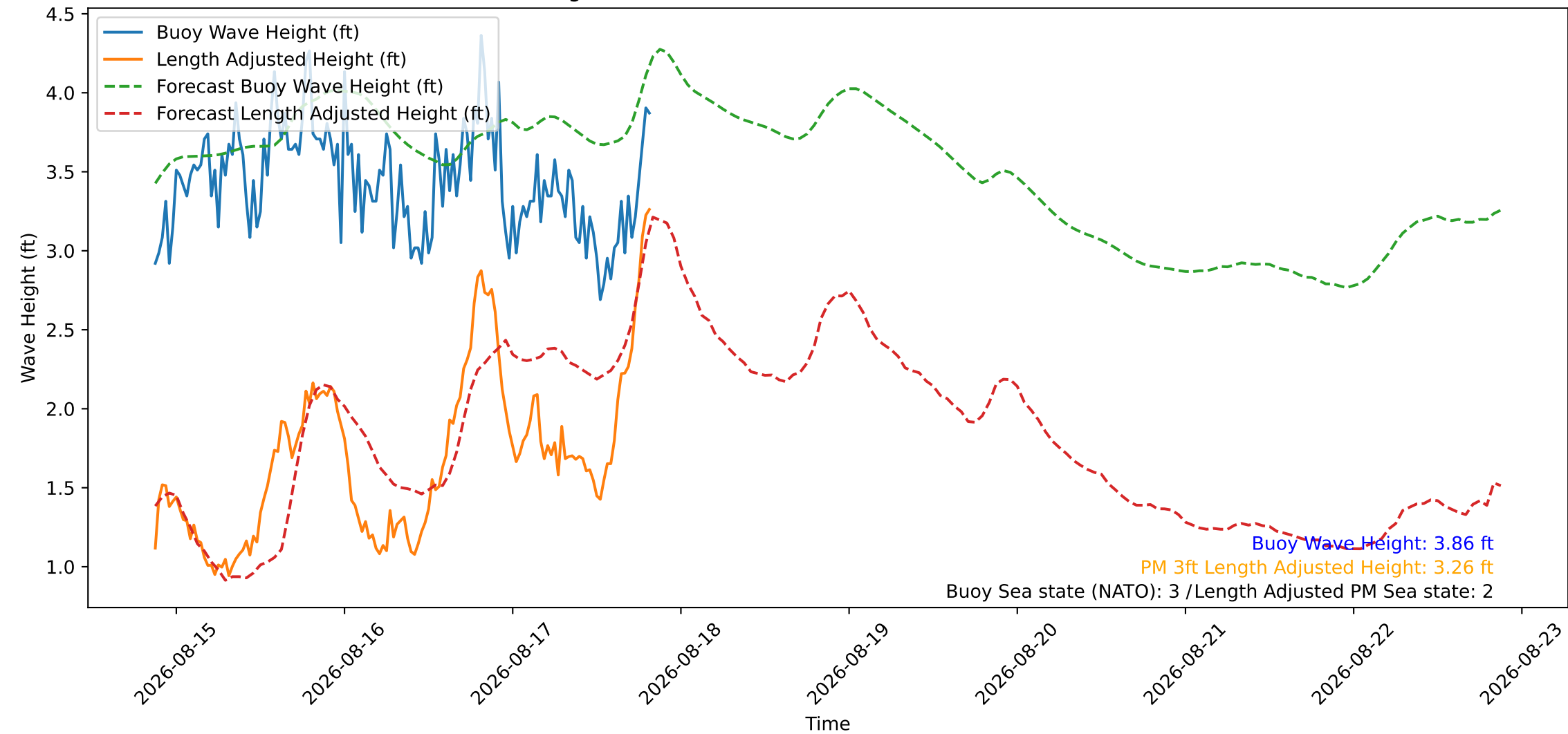
Wave Heights over Time for Green Beach at 2026-08-17 20:31:08
