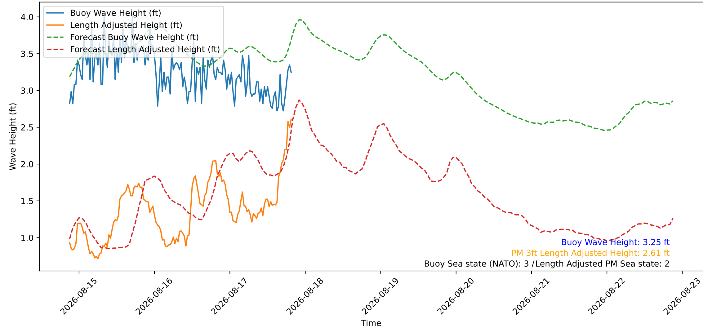
Wave Heights over Time for Red Beach at 2026-08-17 20:30:46
