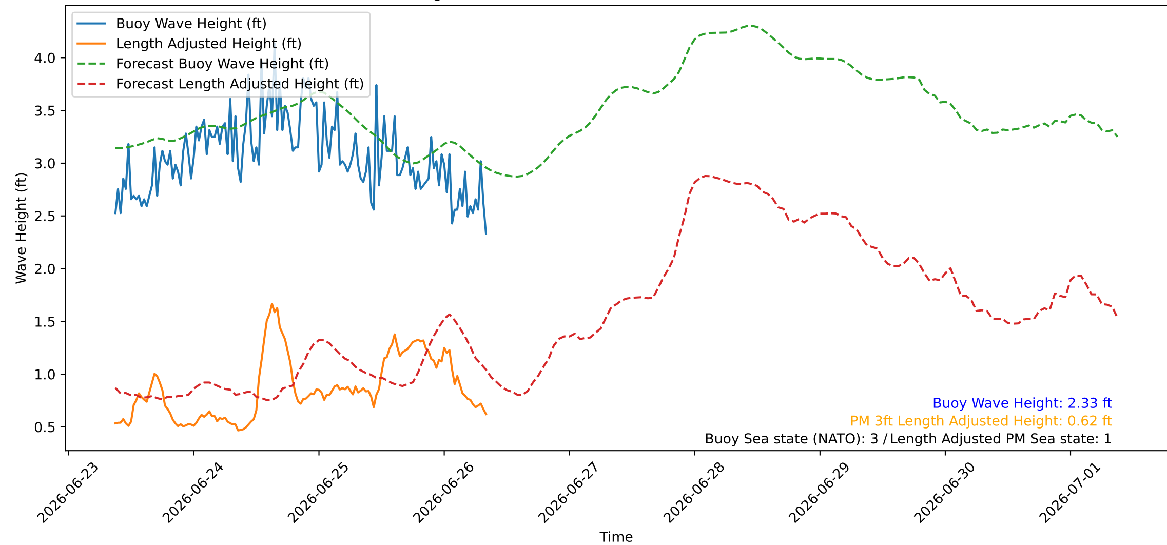
Wave Heights over Time for Red Beach at 2026-06-26 08:40:46
