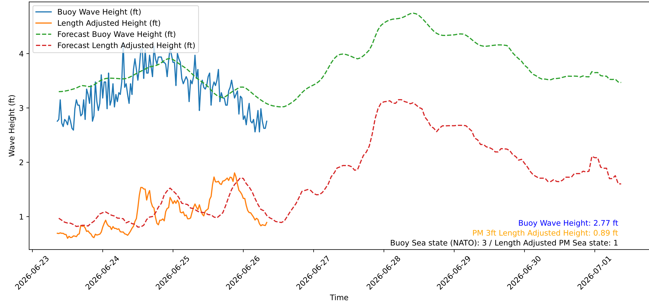
Wave Heights over Time for Green Beach at 2026-06-26 08:41:09
