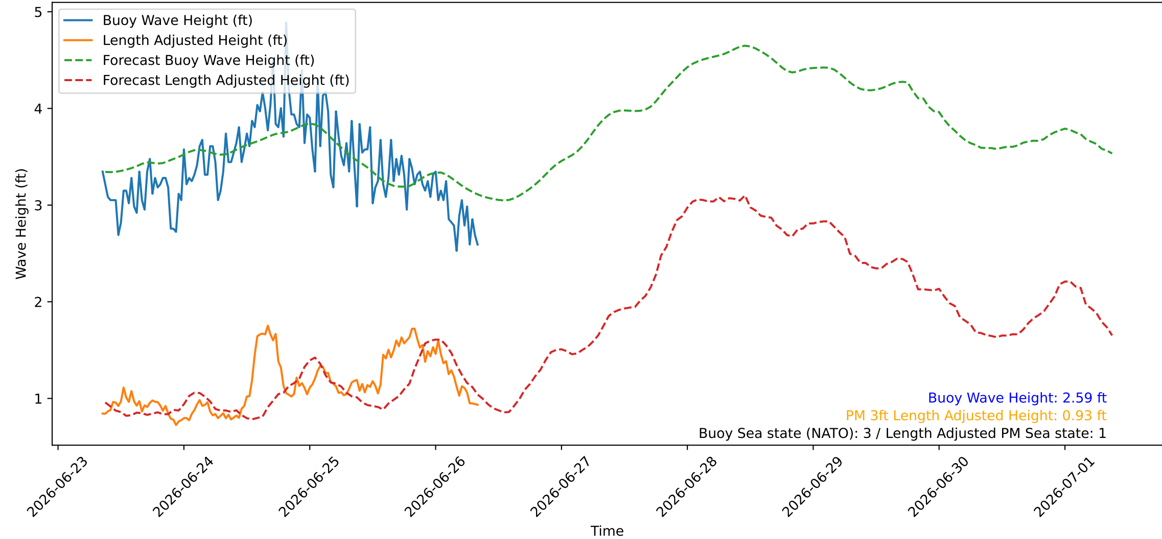
Wave Heights over Time for Oceanside Harbor at 2026-06-26 08:40:26
