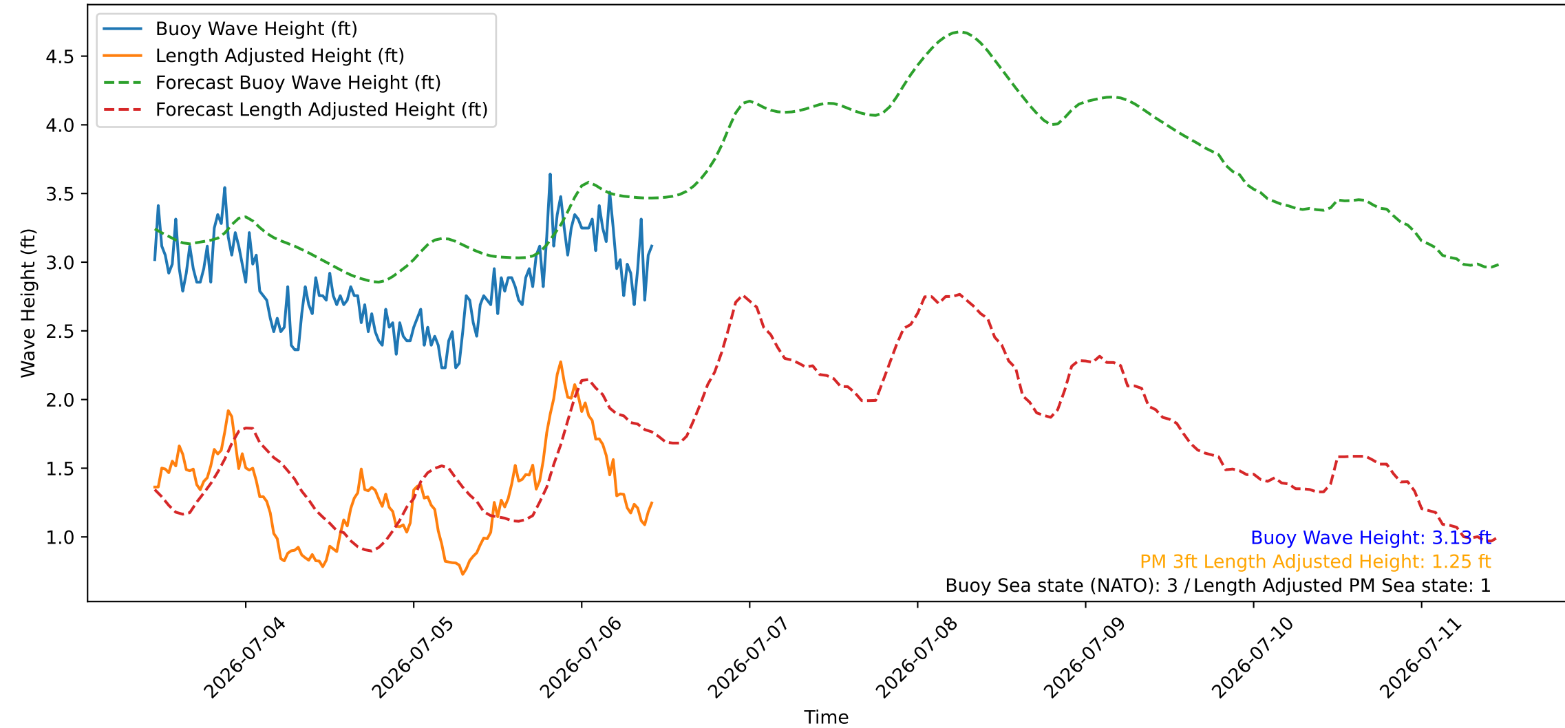
Wave Heights over Time for Red Beach at 2026-07-06 10:50:47
