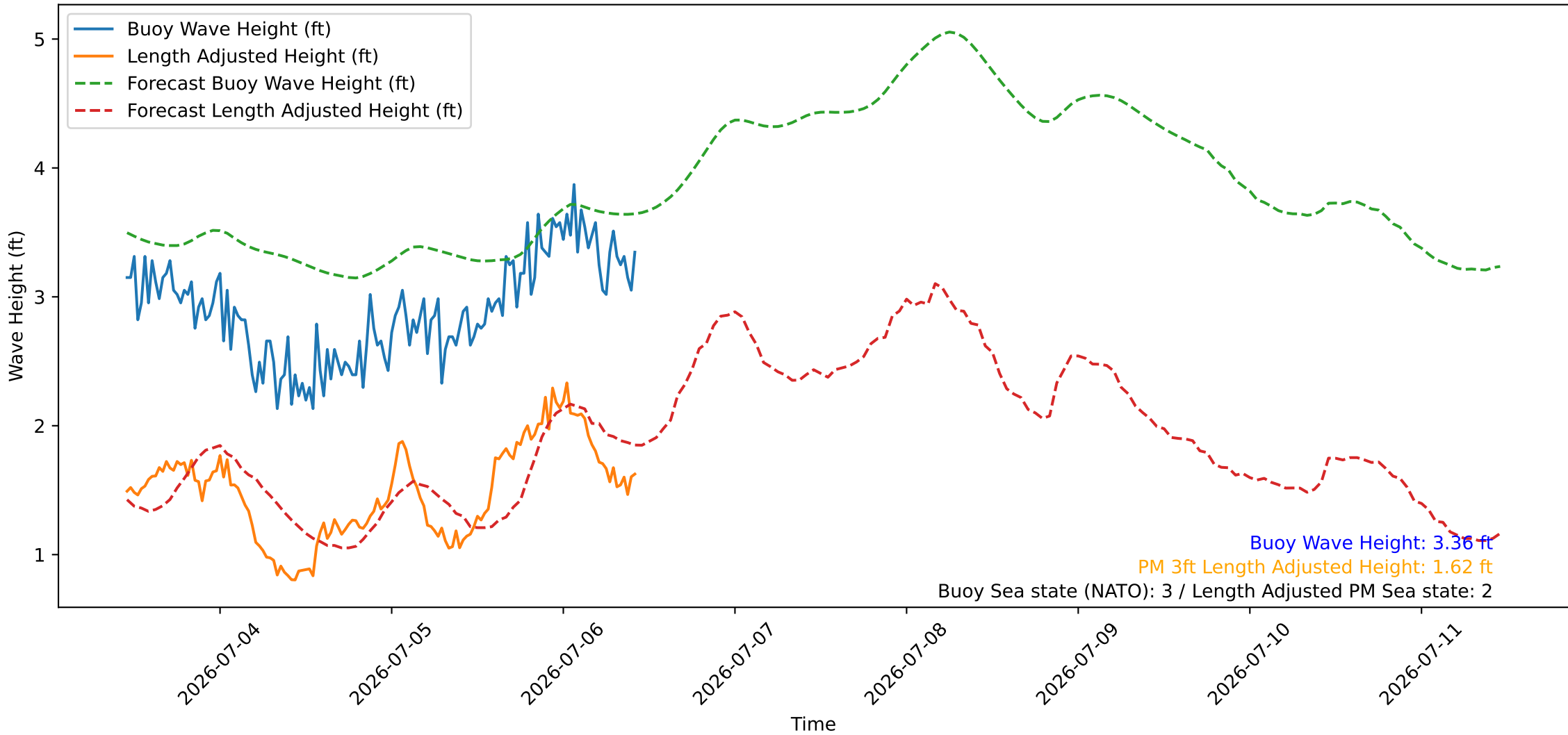
Wave Heights over Time for Oceanside Harbor at 2026-07-06 10:50:26
