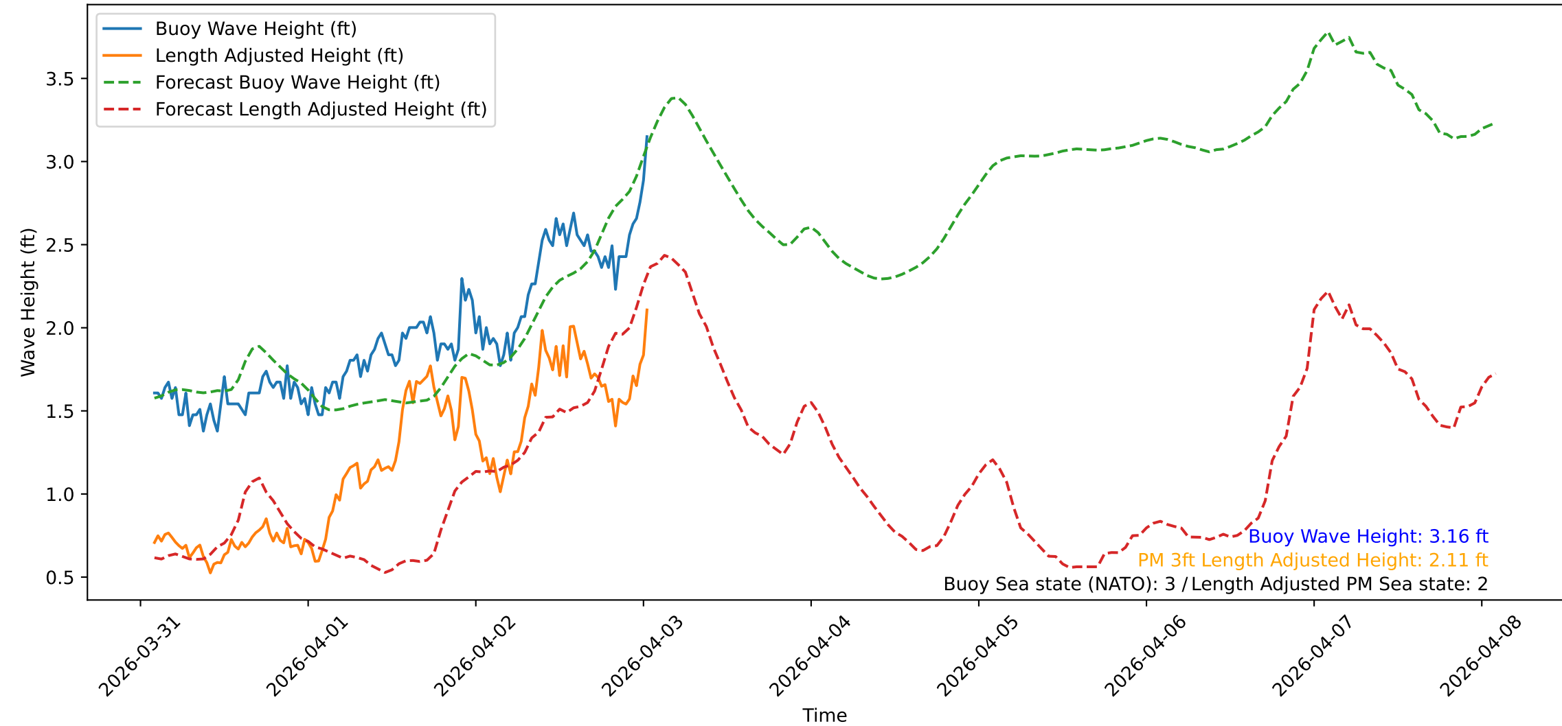
Wave Heights over Time for Red Beach at 2026-04-03 01:40:47
