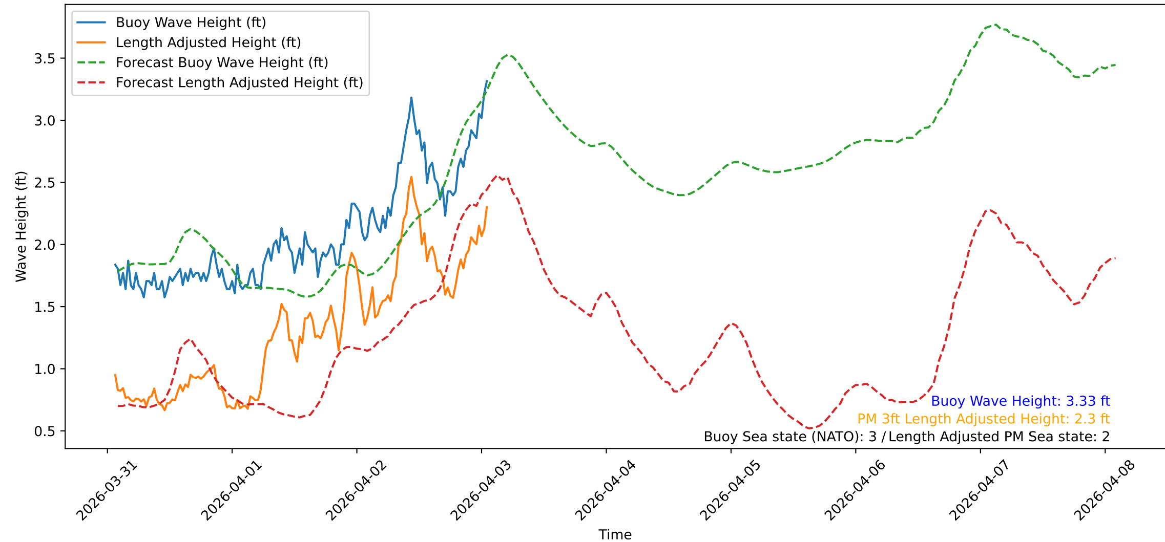
Wave Heights over Time for Oceanside Harbor at 2026-04-03 01:40:31
