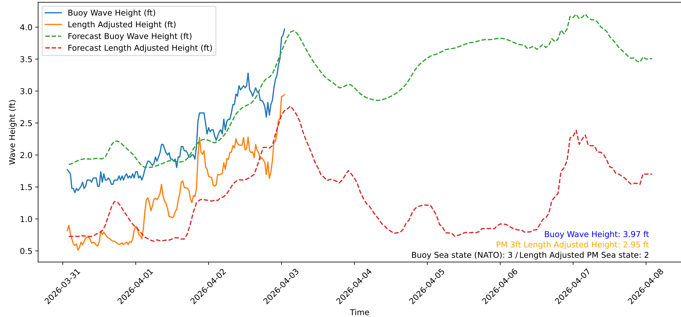
Wave Heights over Time for Green Beach at 2026-04-03 01:41:10
