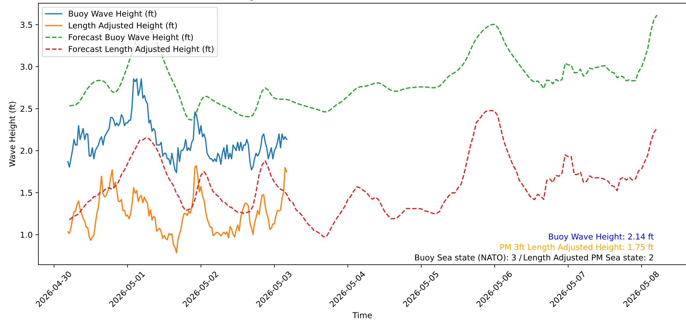
Wave Heights over Time for Green Beach at 2026-05-03 04:41:13
