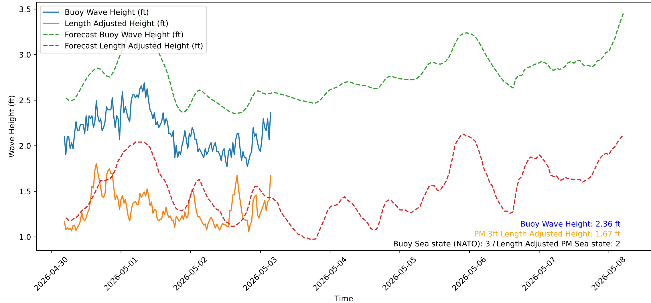
Wave Heights over Time for Oceanside Harbor at 2026-05-03 04:40:31
