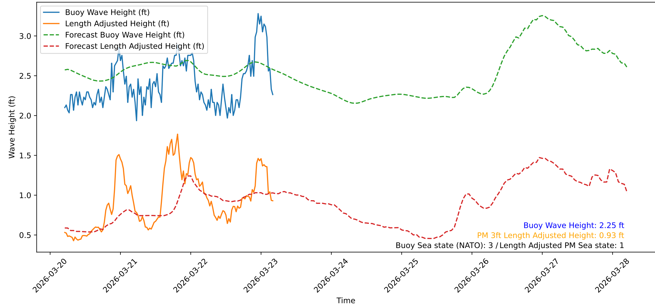
Wave Heights over Time for Green Beach at 2026-03-23 05:01:10
