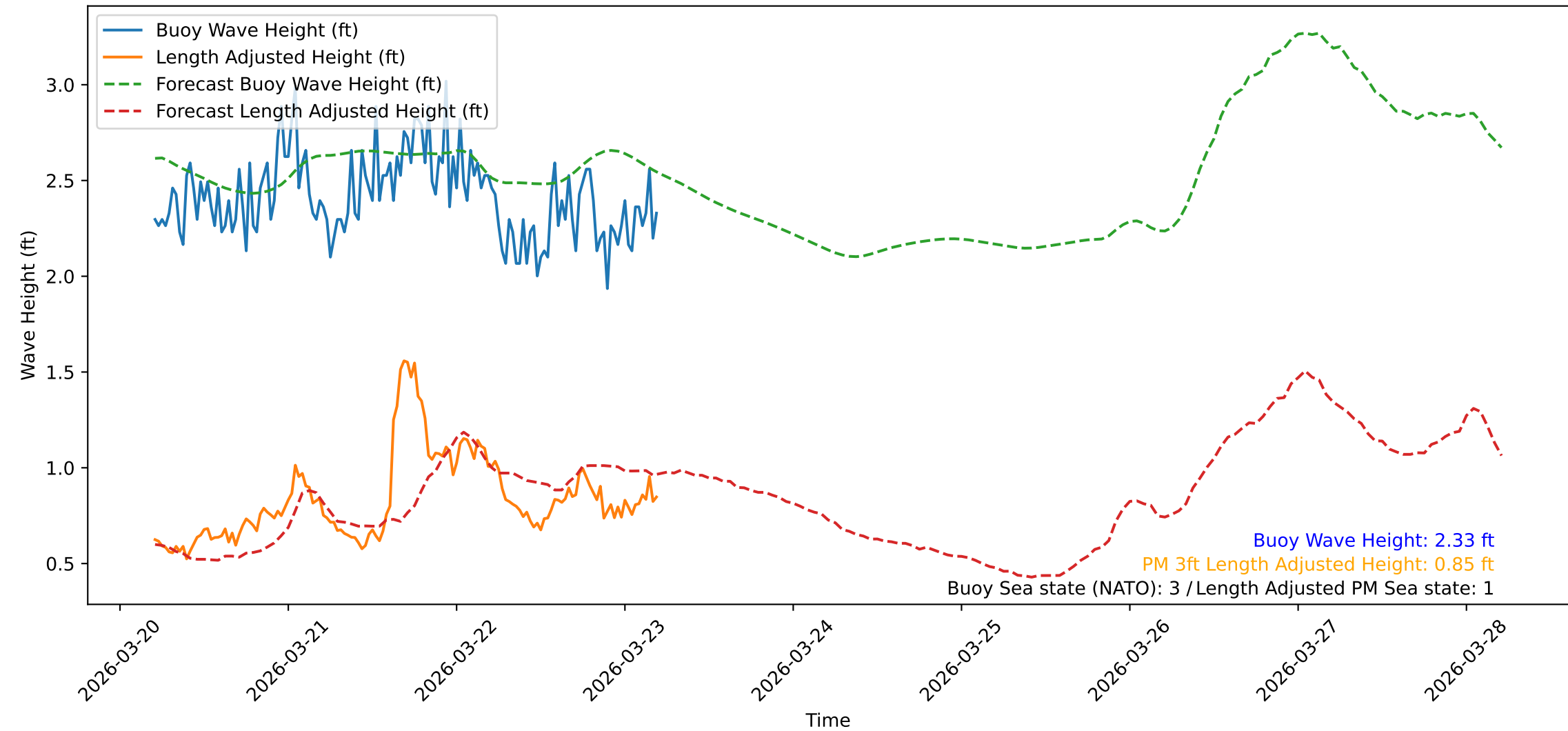
Wave Heights over Time for Oceanside Harbor at 2026-03-23 05:00:31
