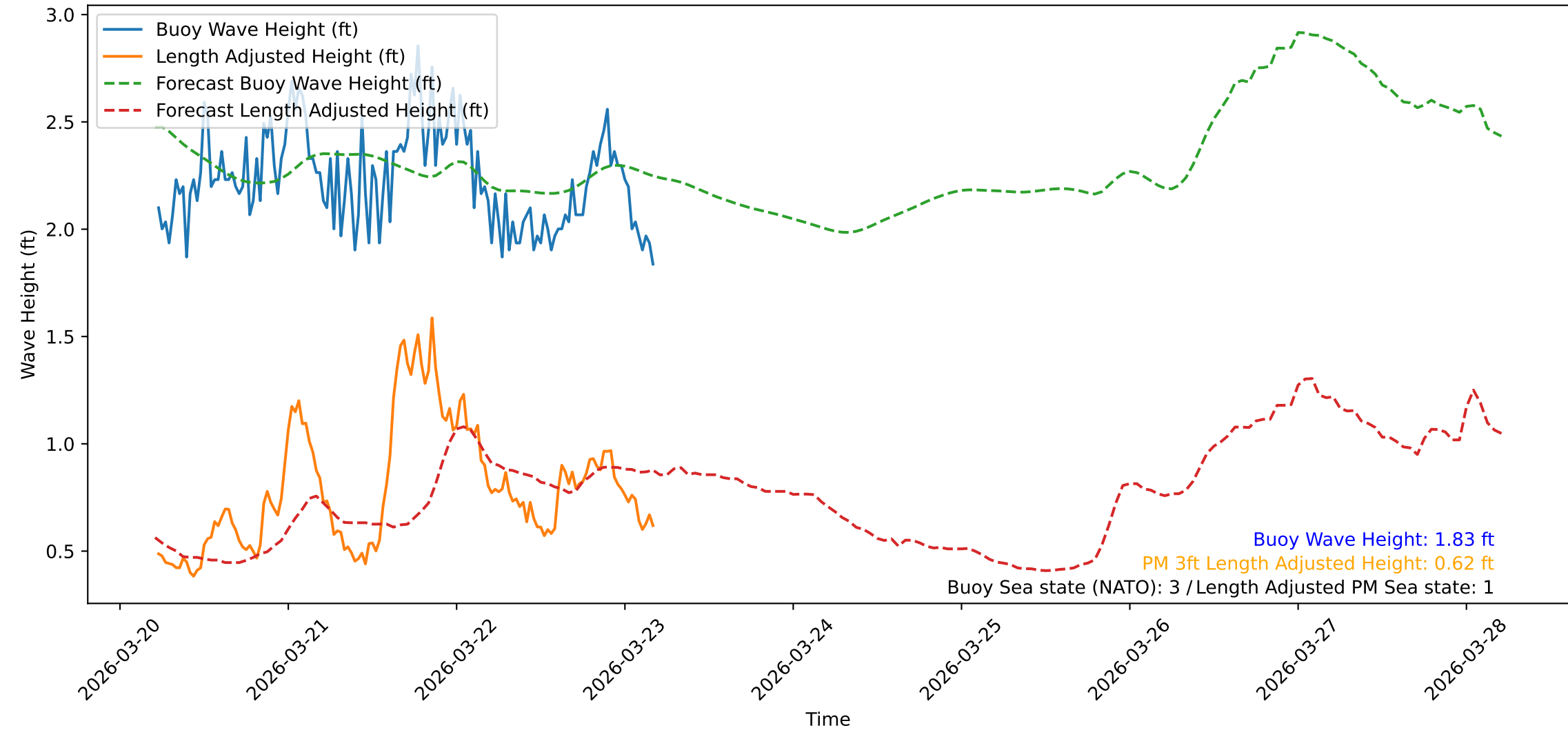
Wave Heights over Time for Red Beach at 2026-03-23 05:00:48
