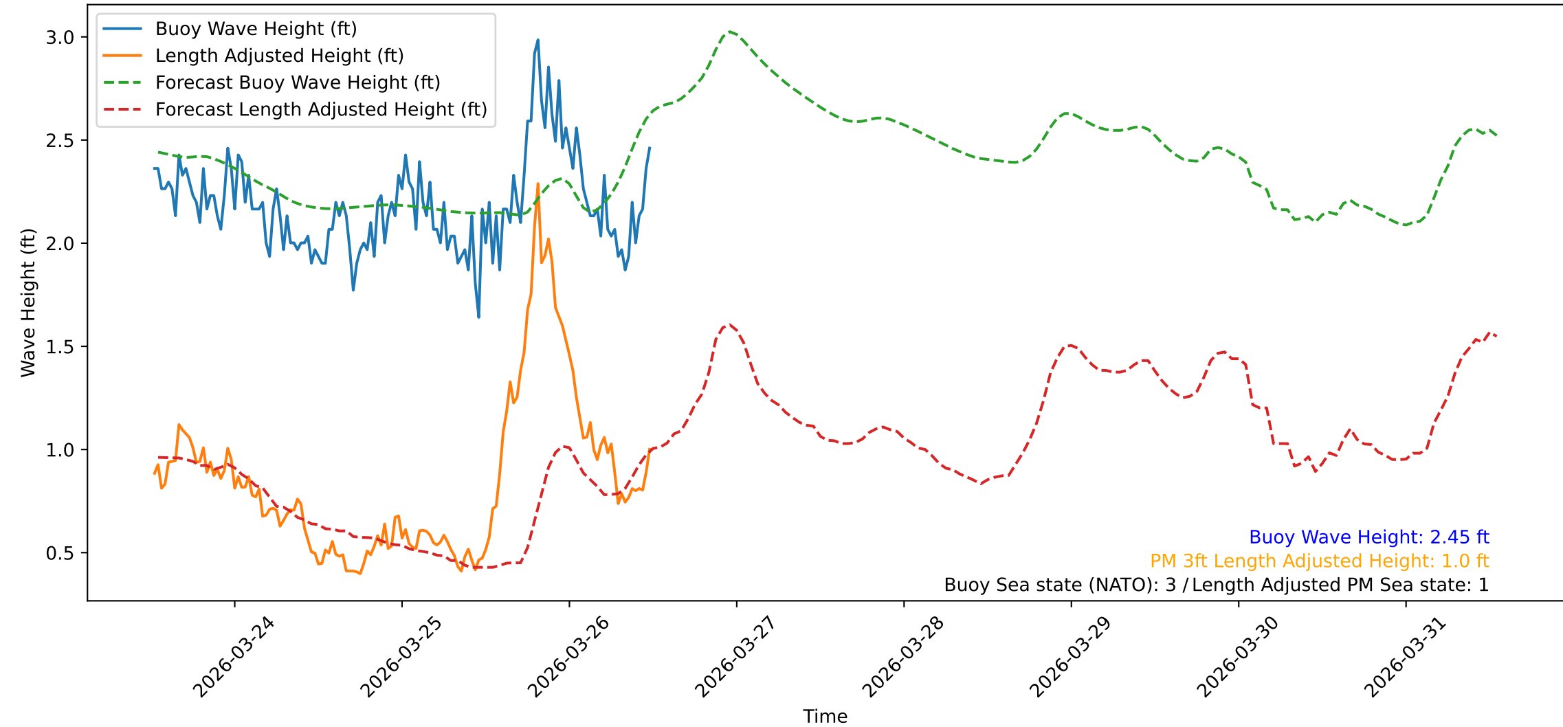
Wave Heights over Time for Green Beach at 2026-03-26 12:31:08
