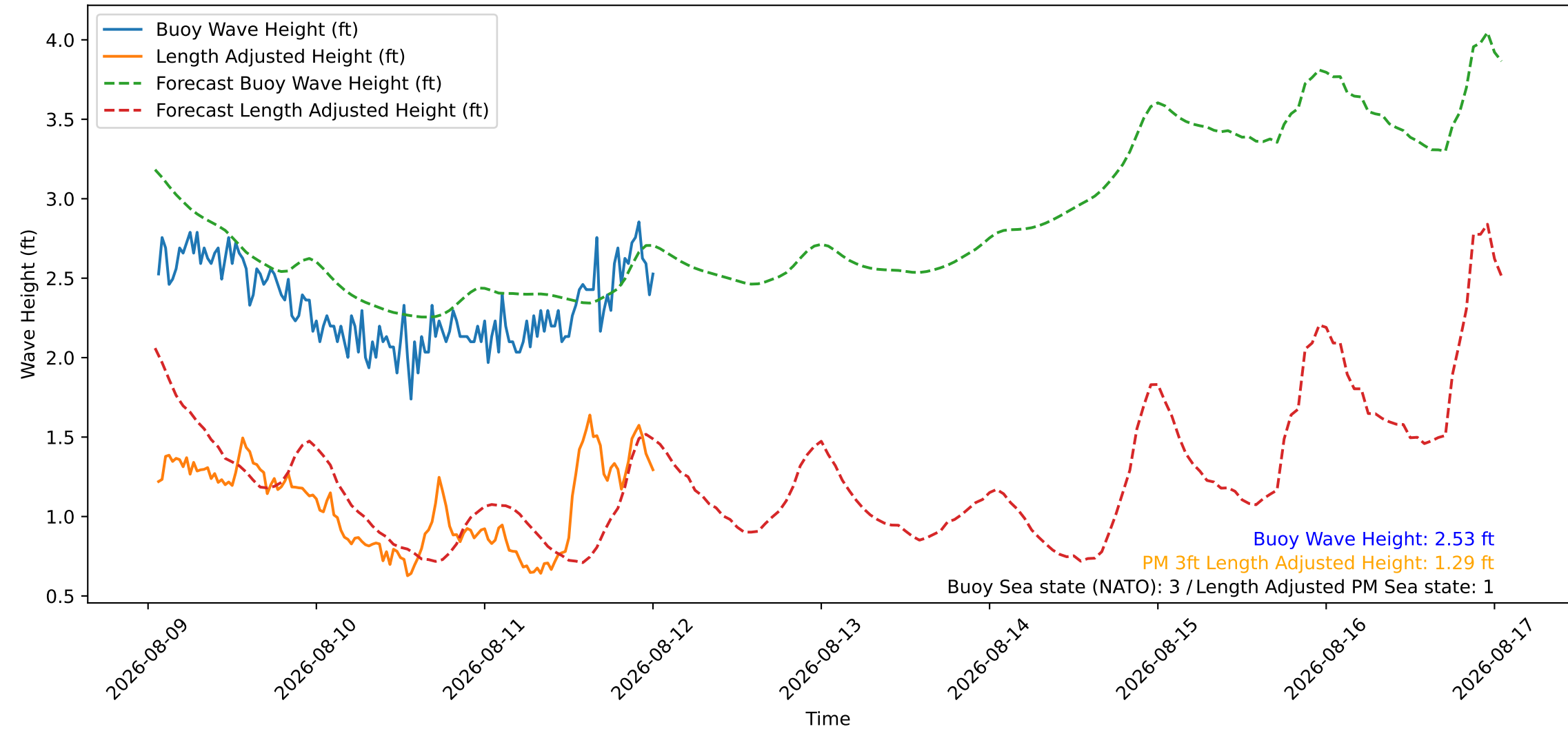
Wave Heights over Time for Red Beach at 2026-08-12 01:00:46
