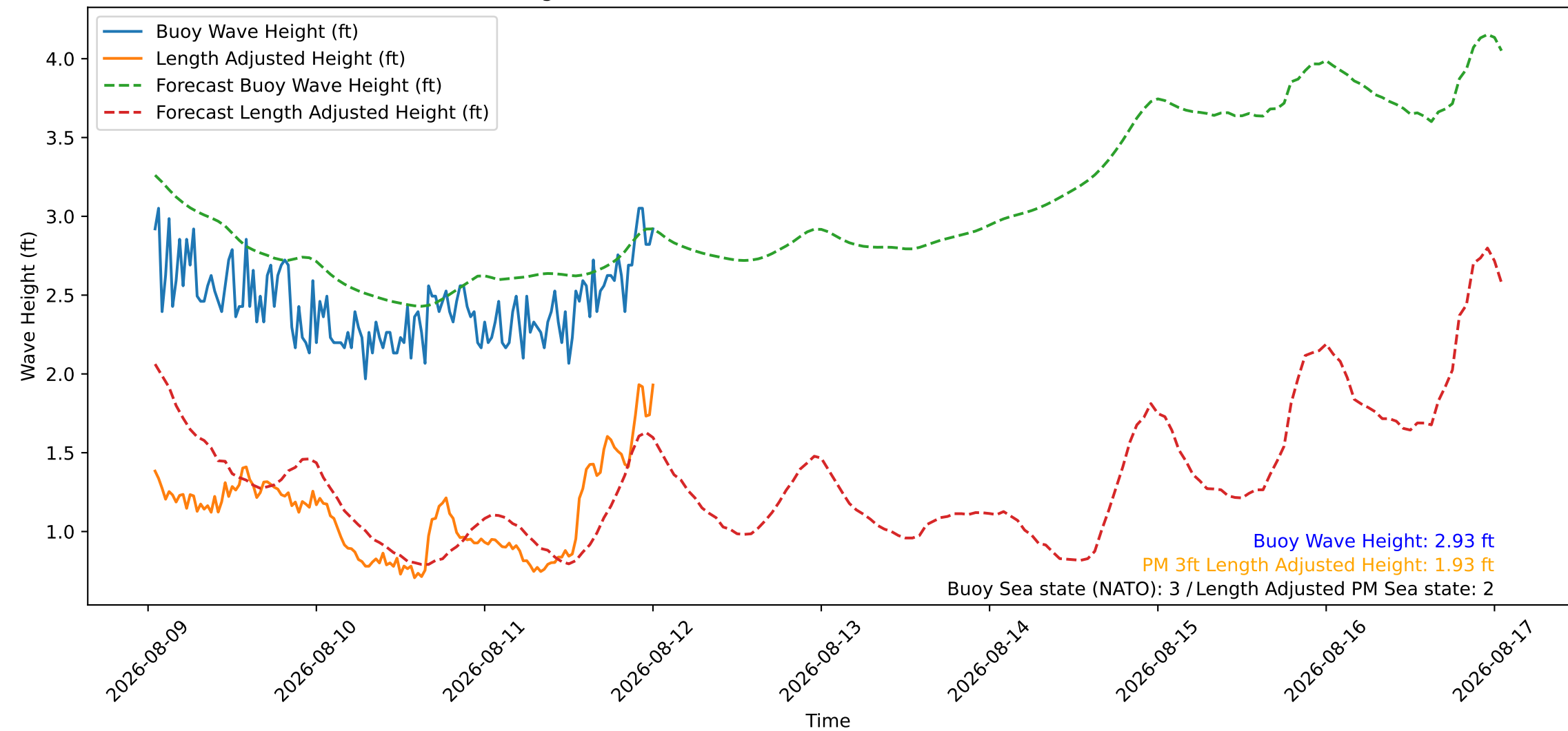
Wave Heights over Time for Oceanside Harbor at 2026-08-12 01:00:27
