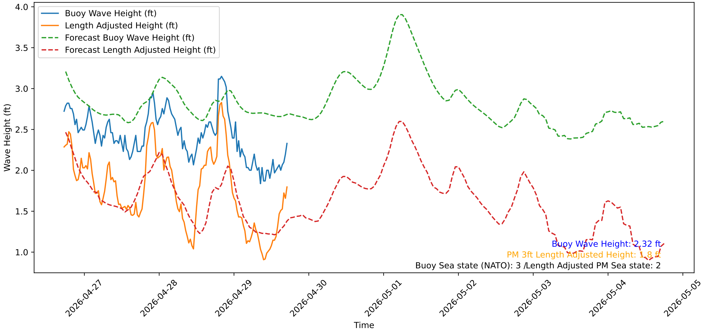
Wave Heights over Time for Green Beach at 2026-04-29 17:41:13
