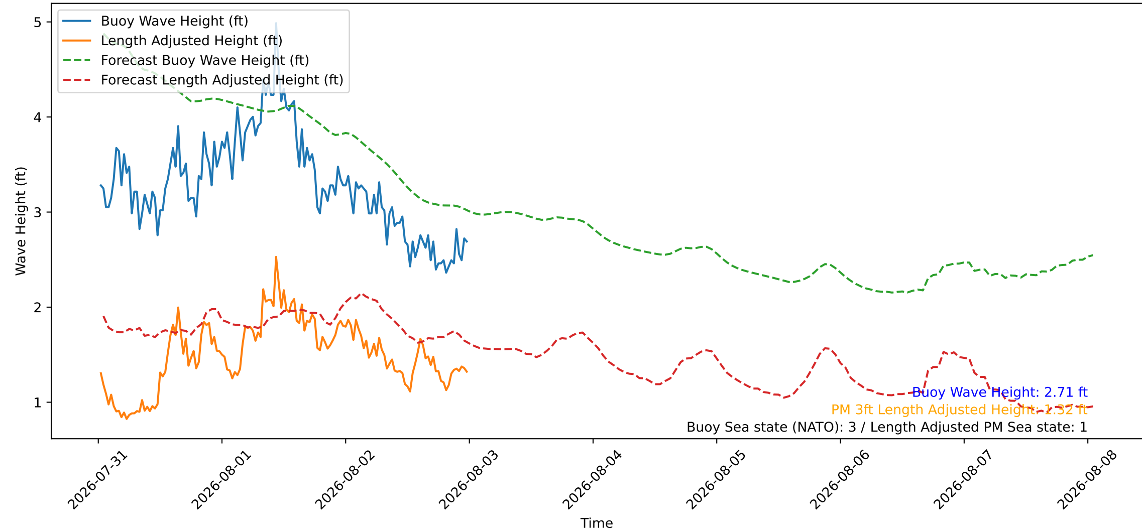
Wave Heights over Time for Green Beach at 2026-08-03 00:31:08
