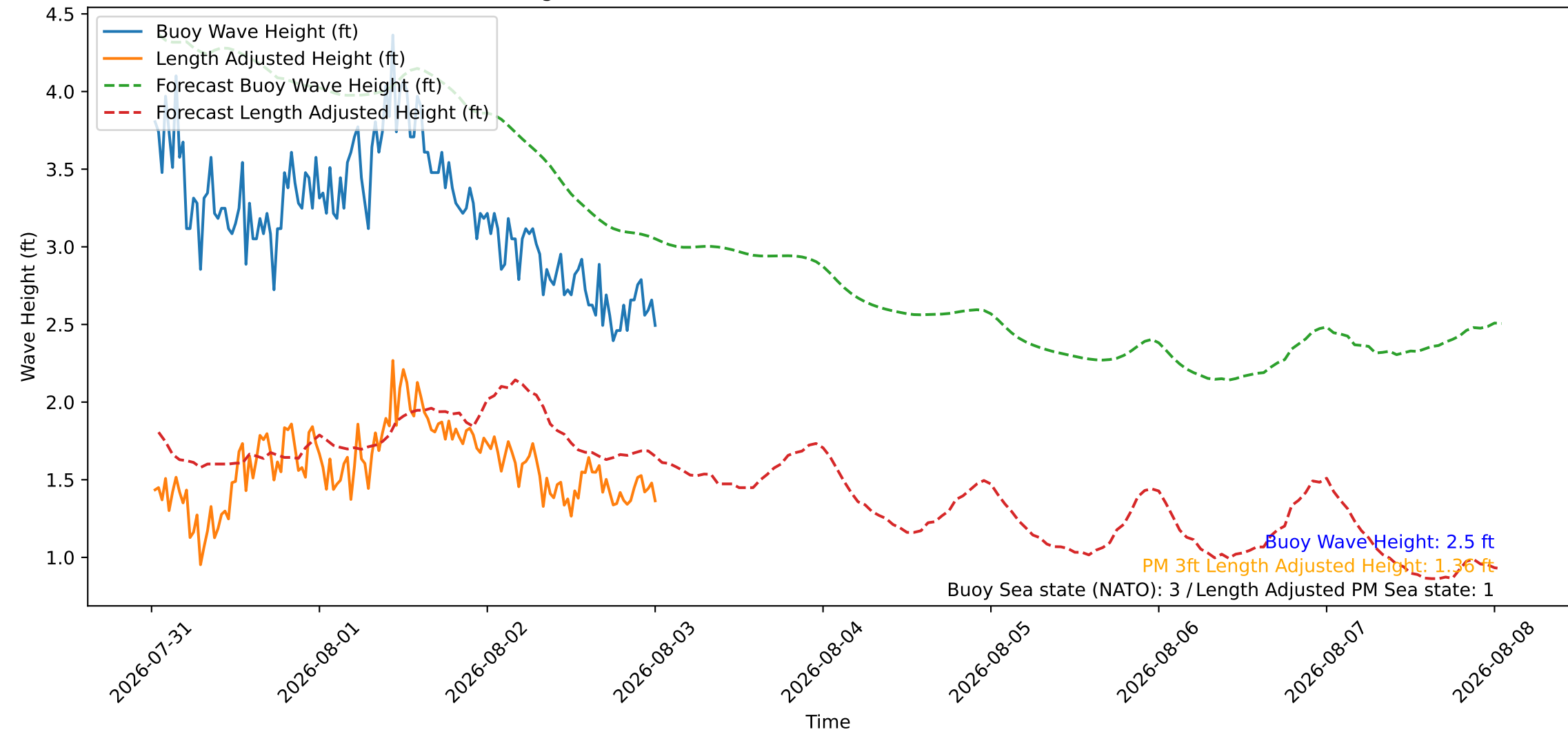
Wave Heights over Time for Oceanside Harbor at 2026-08-03 00:30:26
