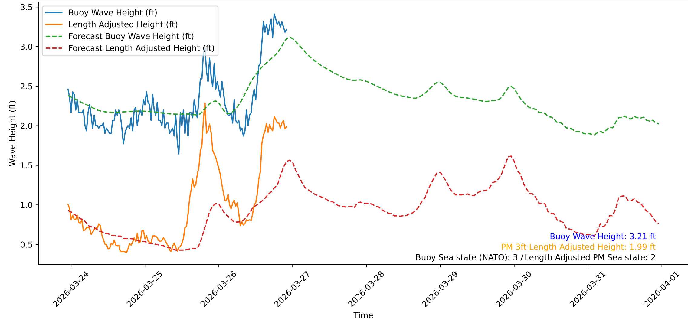
Wave Heights over Time for Green Beach at 2026-03-26 22:51:08
