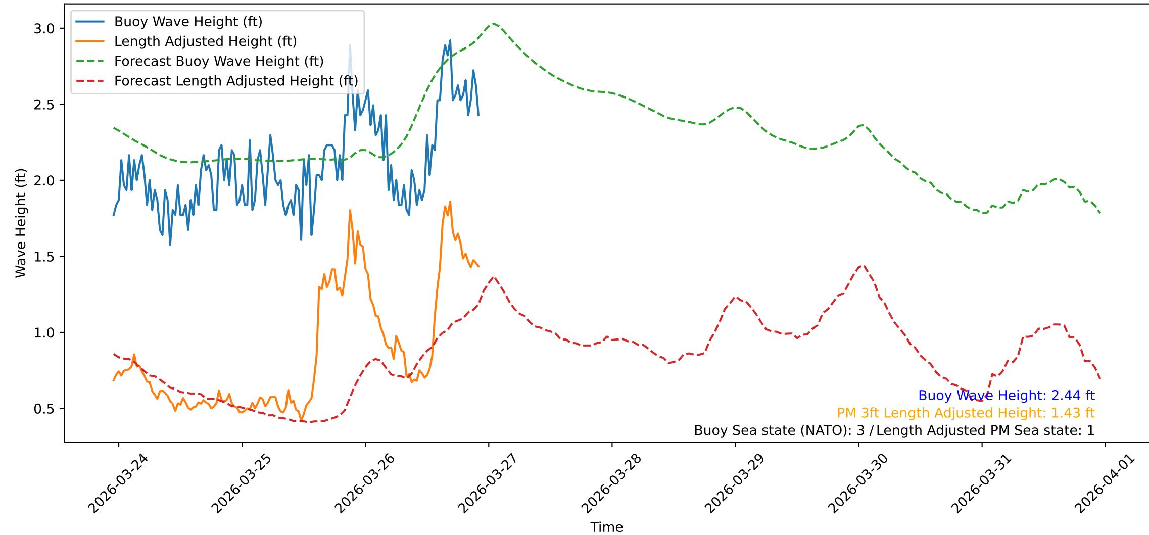
Wave Heights over Time for Oceanside Harbor at 2026-03-26 22:50:30
