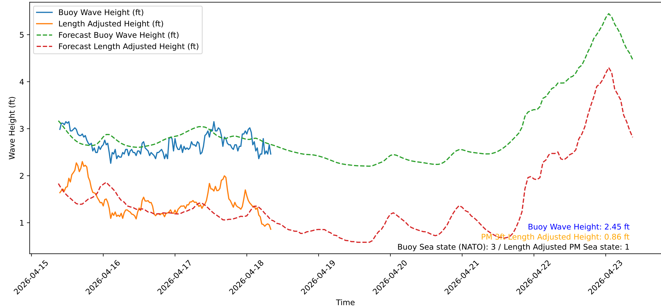
Wave Heights over Time for Red Beach at 2026-04-18 09:10:50
