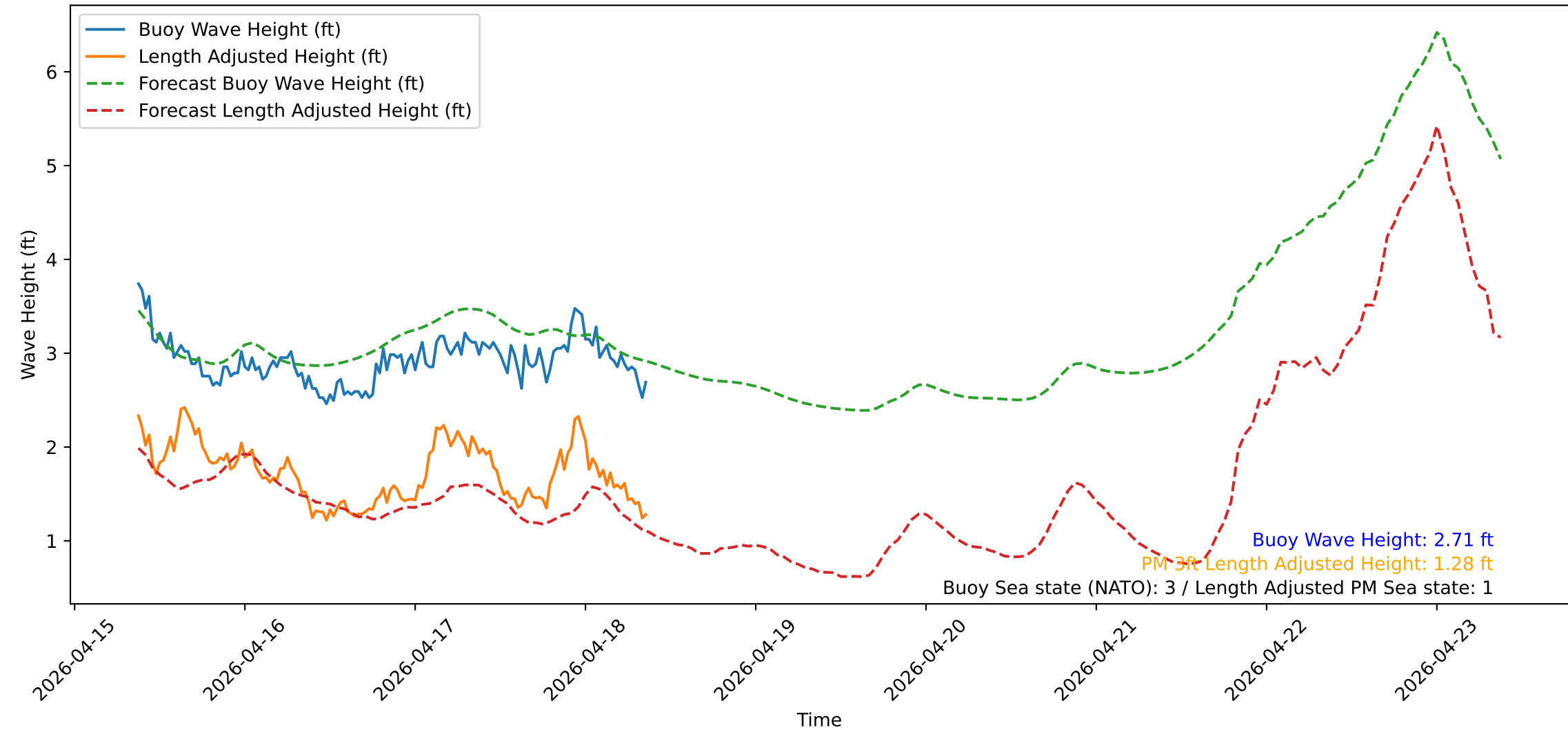
Wave Heights over Time for Green Beach at 2026-04-18 09:11:12
