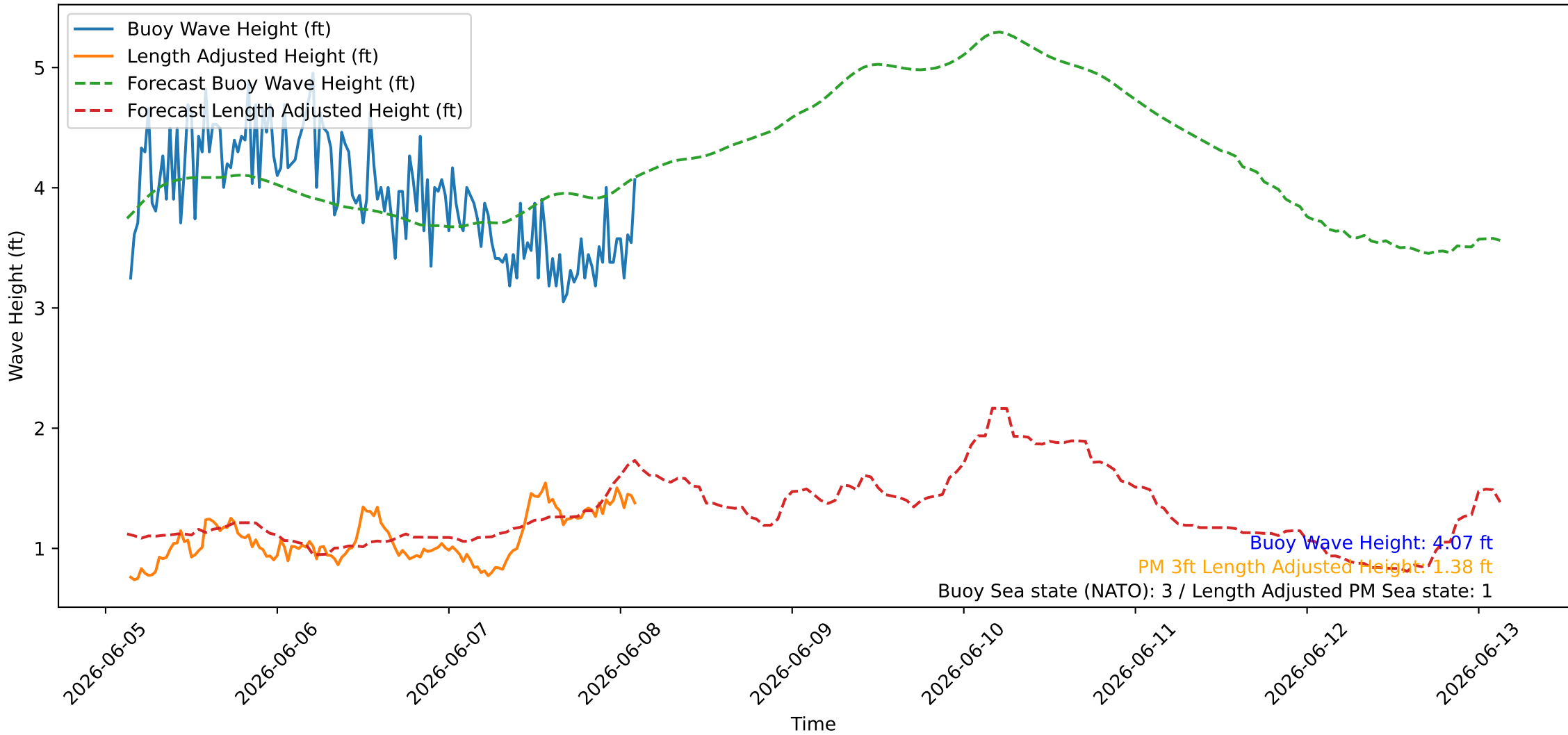
Wave Heights over Time for Red Beach at 2026-06-08 03:00:45
