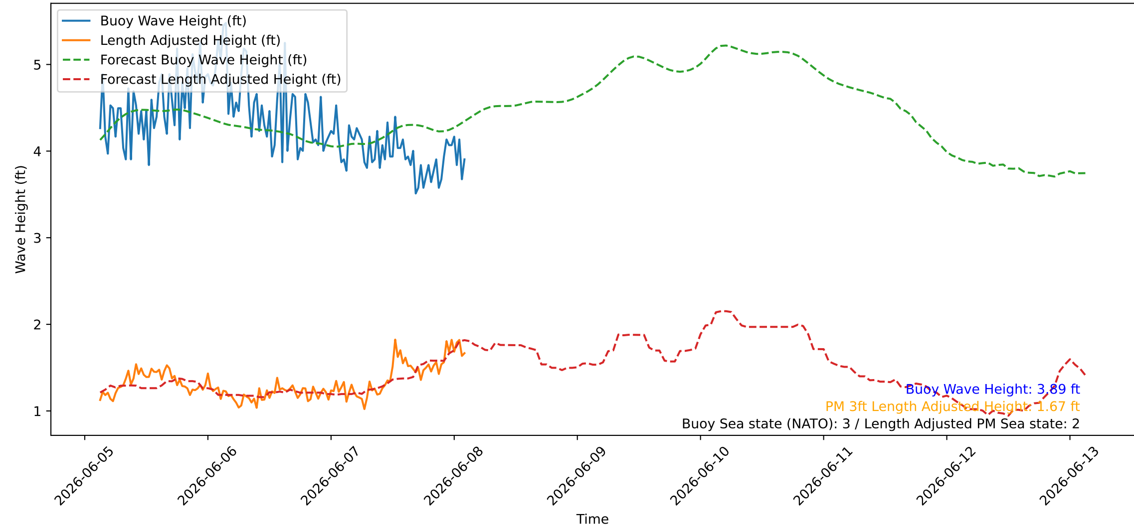
Wave Heights over Time for Oceanside Harbor at 2026-06-08 03:00:26
