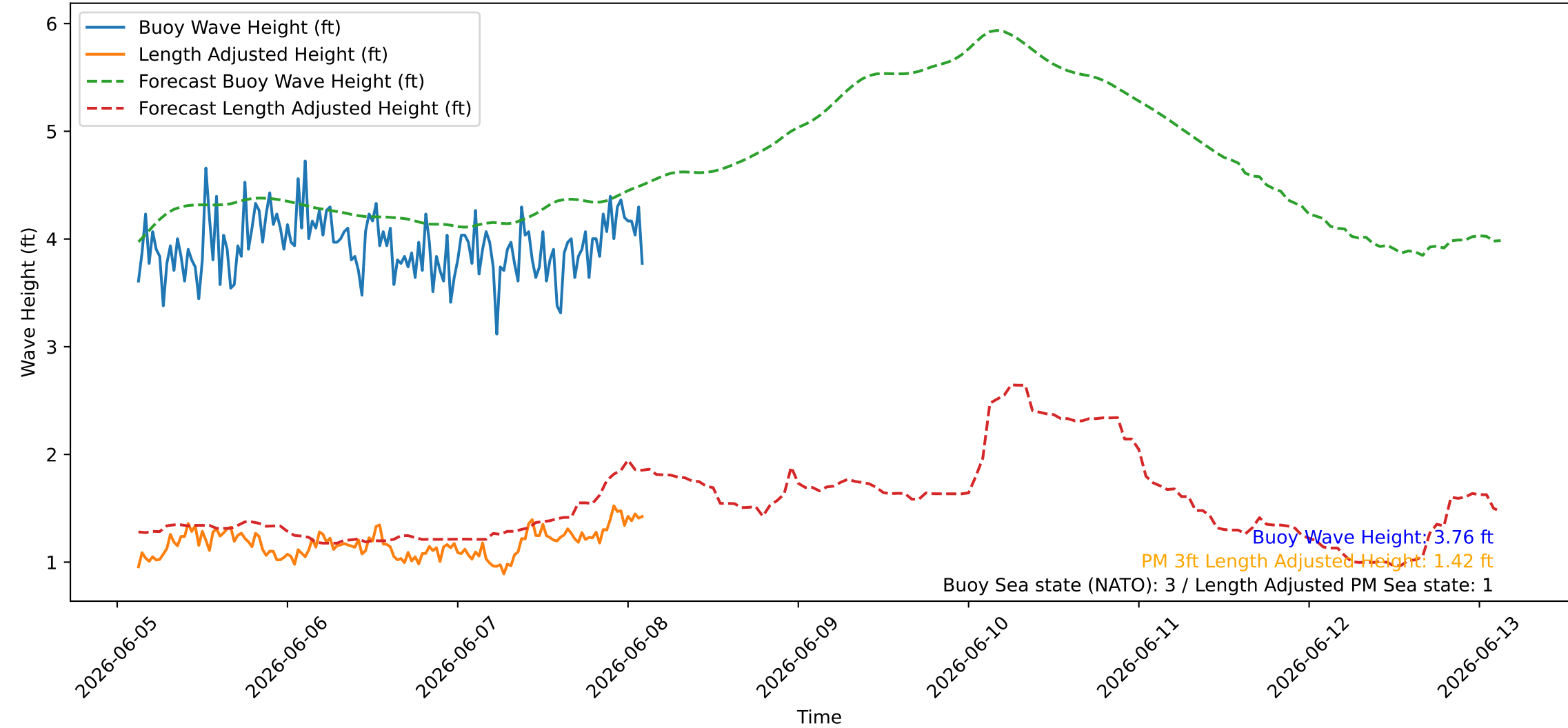
Wave Heights over Time for Green Beach at 2026-06-08 03:01:07
