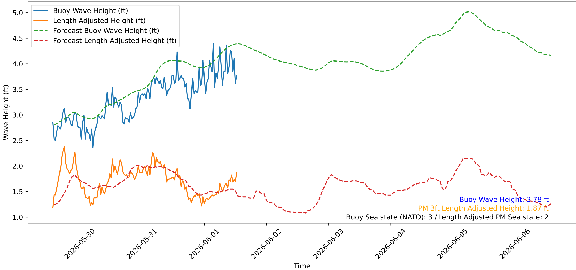
Wave Heights over Time for Oceanside Harbor at 2026-06-01 13:30:26
