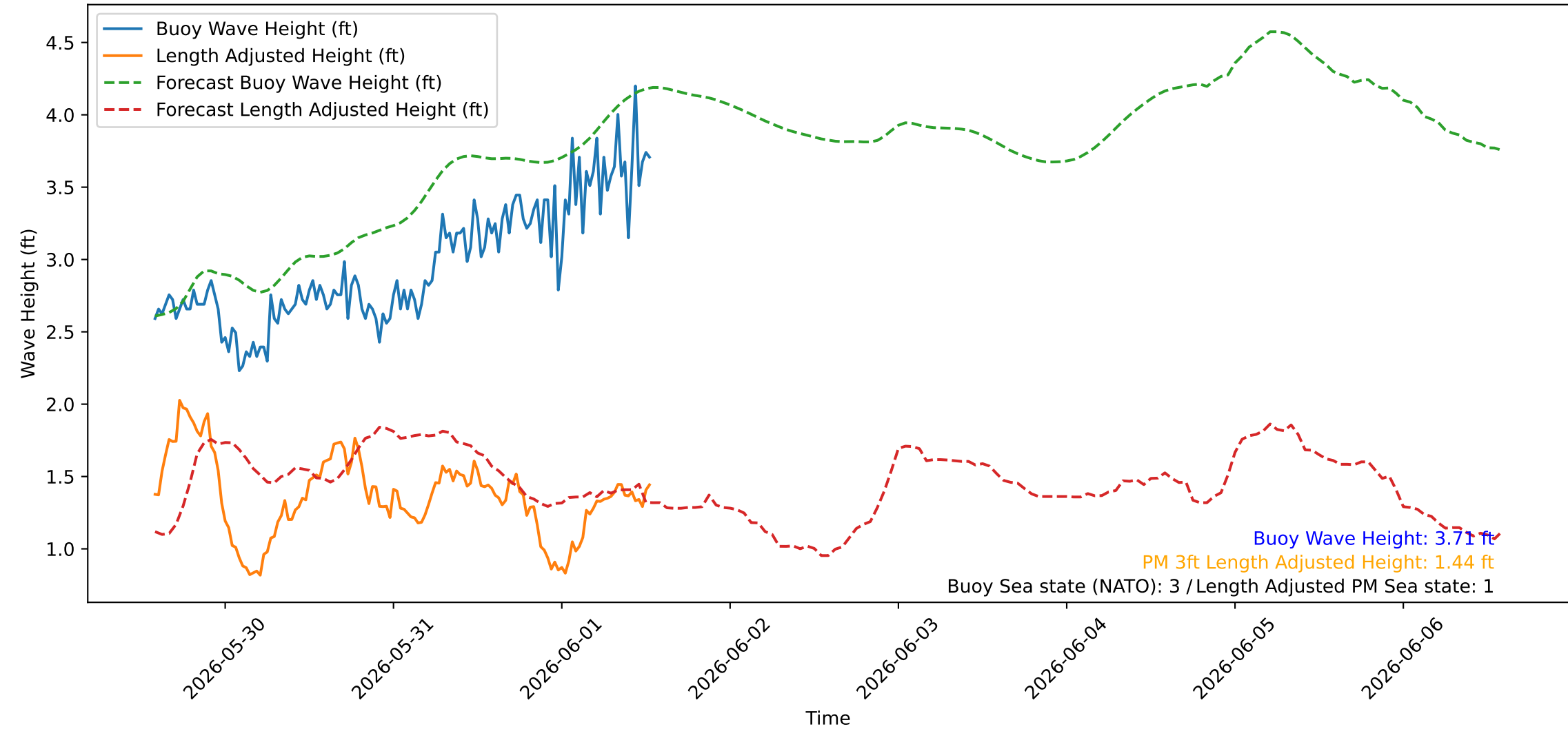
Wave Heights over Time for Red Beach at 2026-06-01 13:30:45
