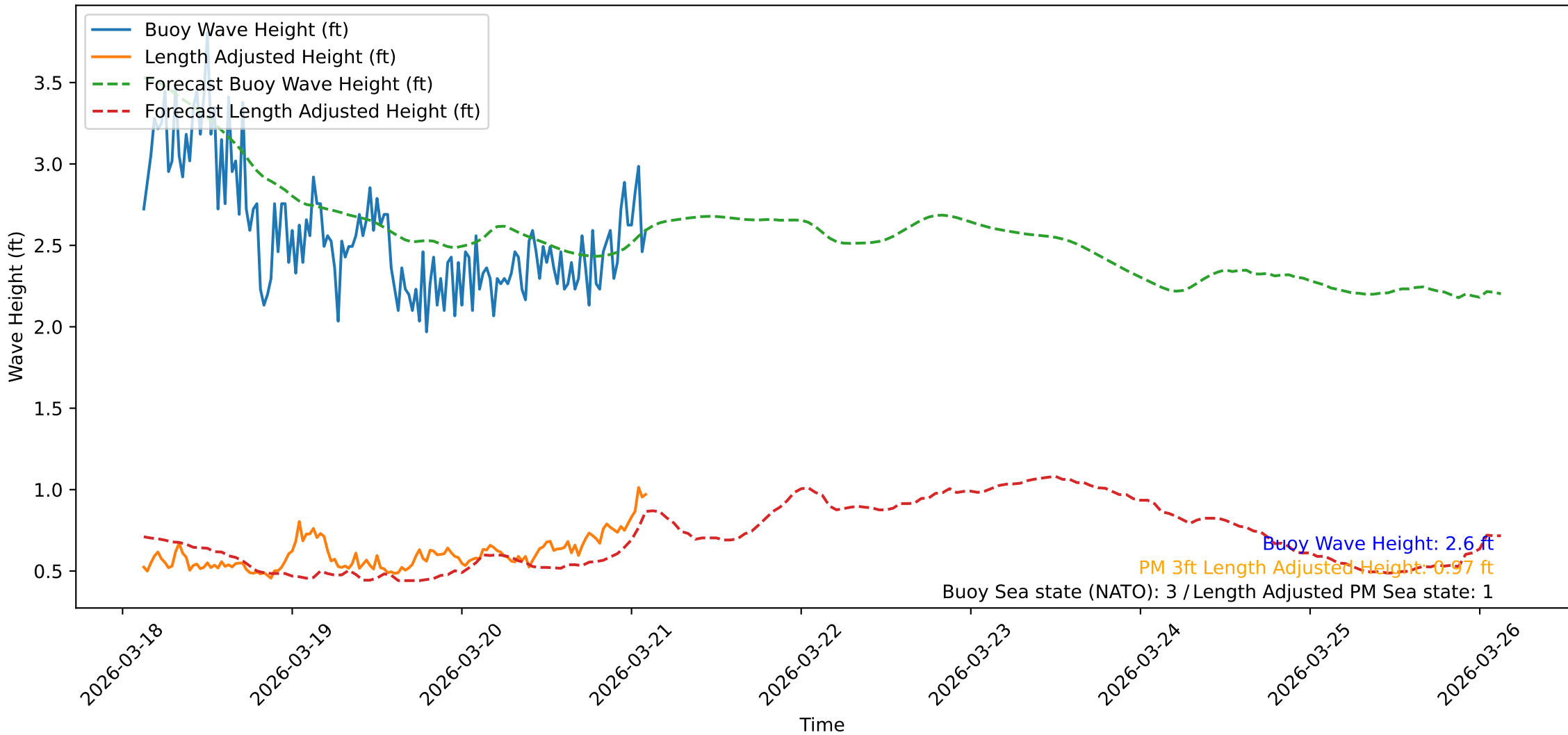
Wave Heights over Time for Oceanside Harbor at 2026-03-21 03:10:32
