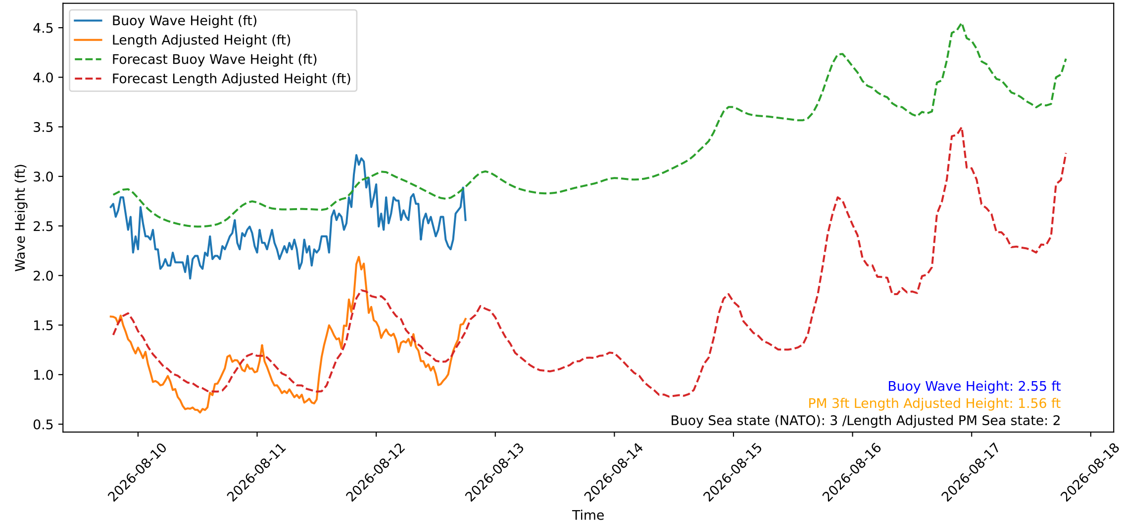
Wave Heights over Time for Green Beach at 2026-08-12 18:41:07
