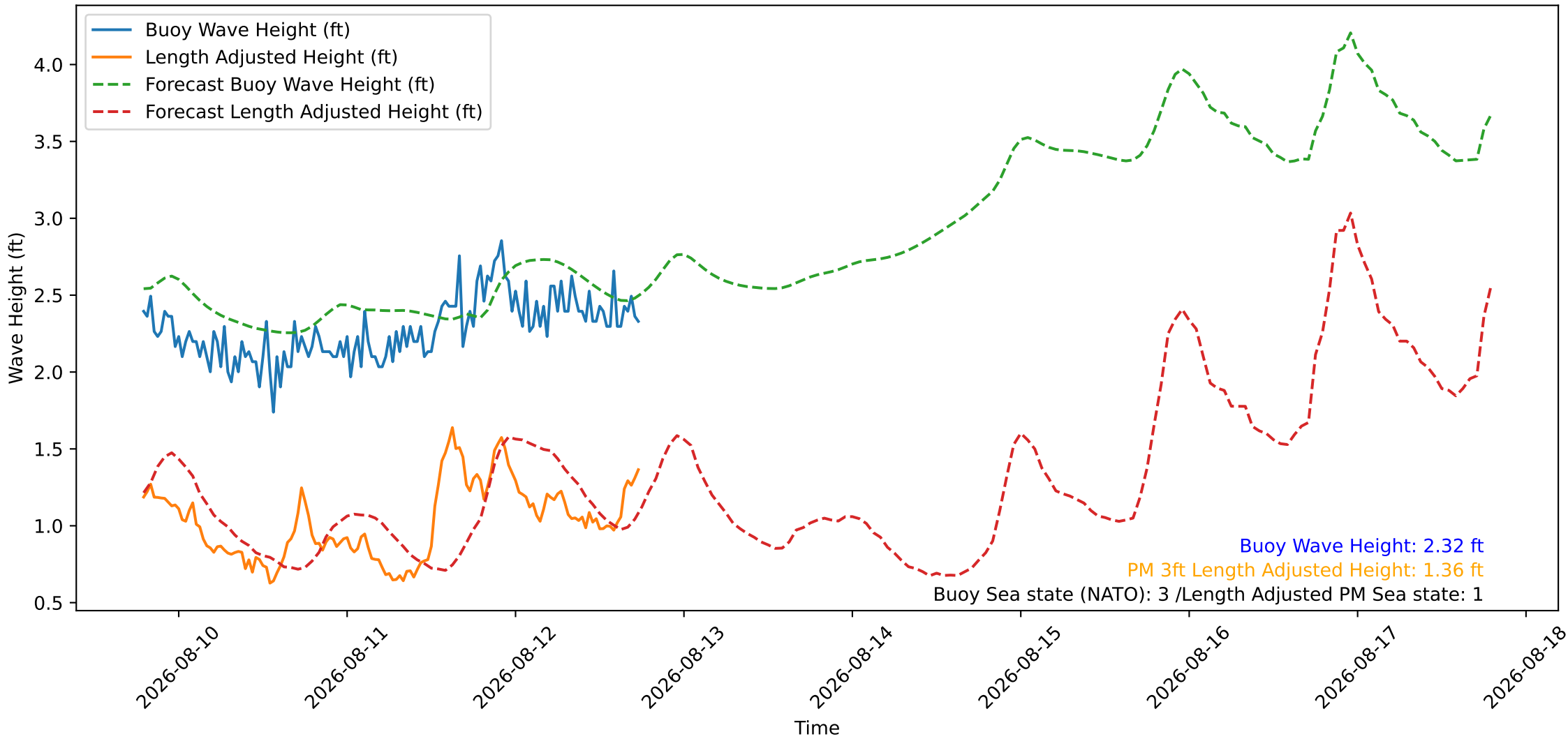
Wave Heights over Time for Red Beach at 2026-08-12 18:40:45
