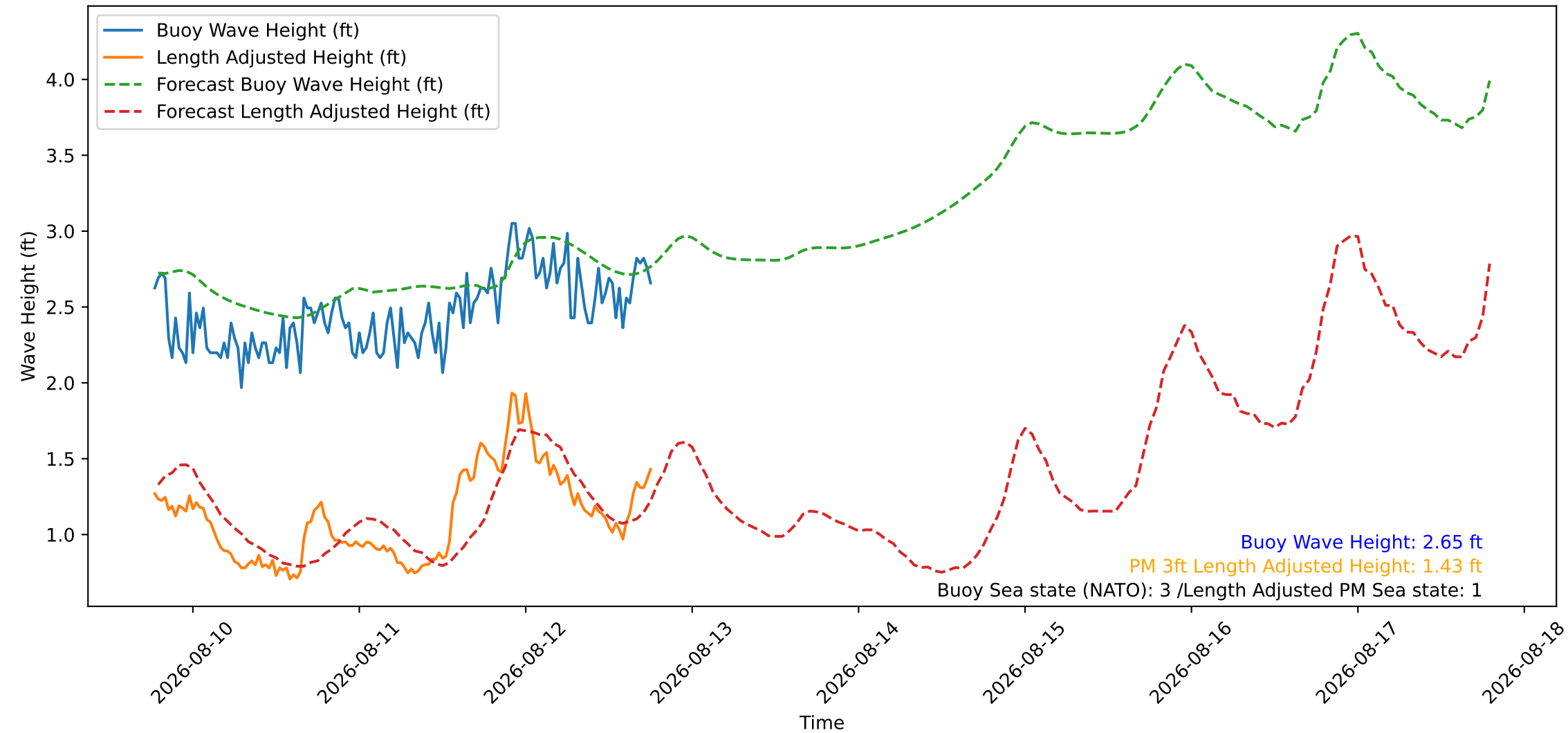
Wave Heights over Time for Oceanside Harbor at 2026-08-12 18:40:26
