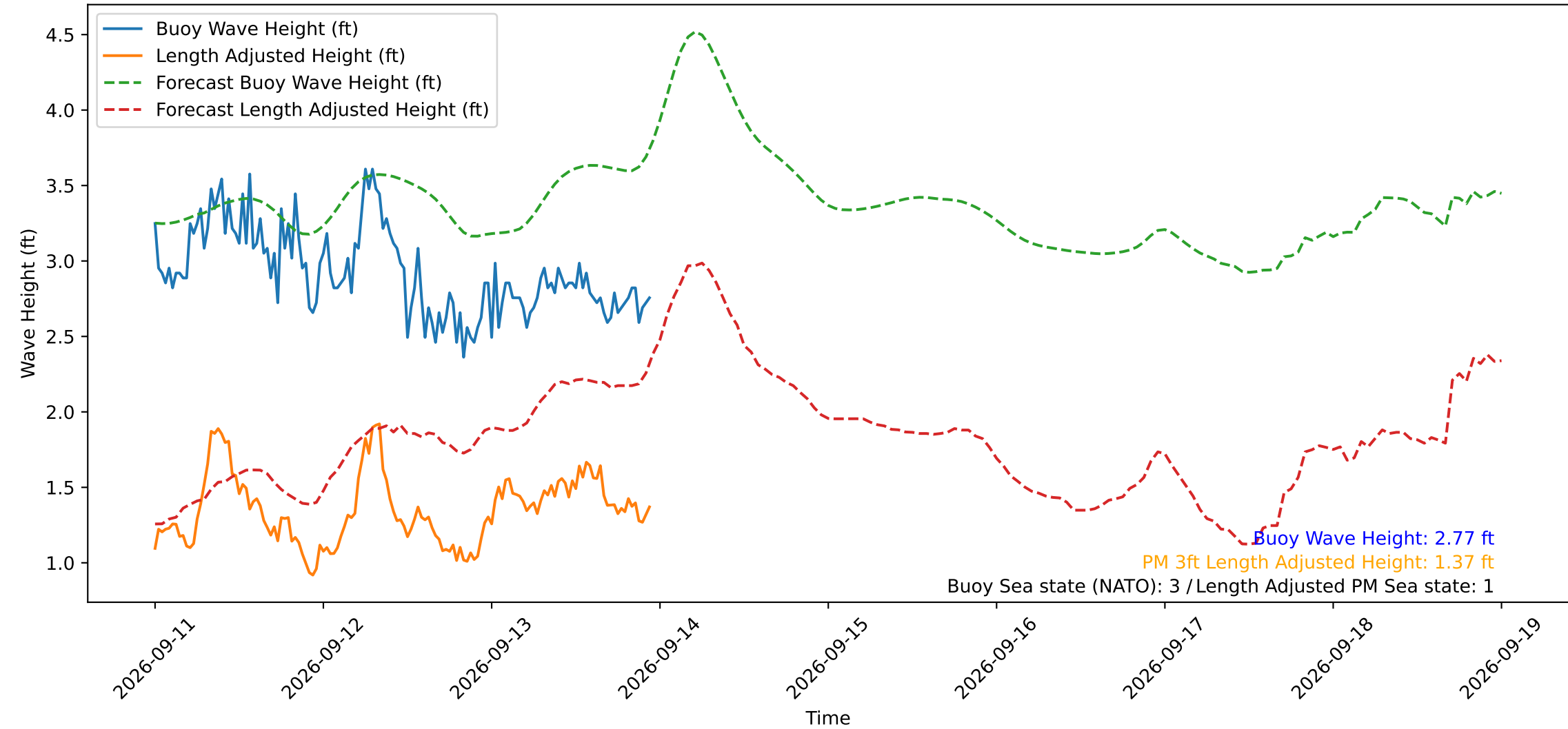
Wave Heights over Time for Green Beach at 2026-09-13 23:31:11
