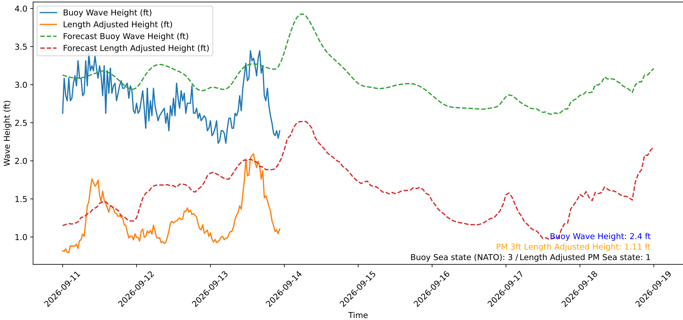
Wave Heights over Time for Red Beach at 2026-09-13 23:30:49
