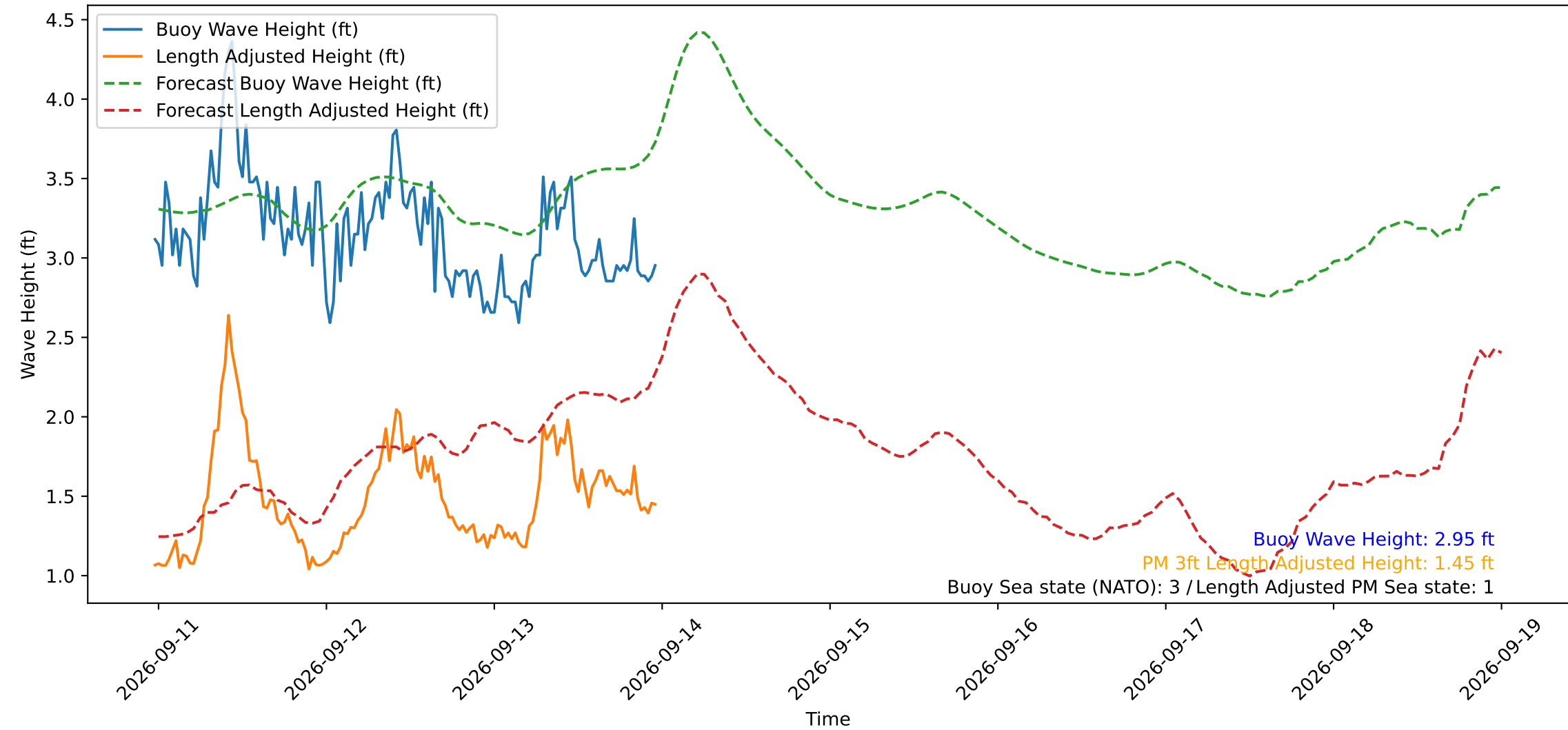
Wave Heights over Time for Oceanside Harbor at 2026-09-13 23:30:30
