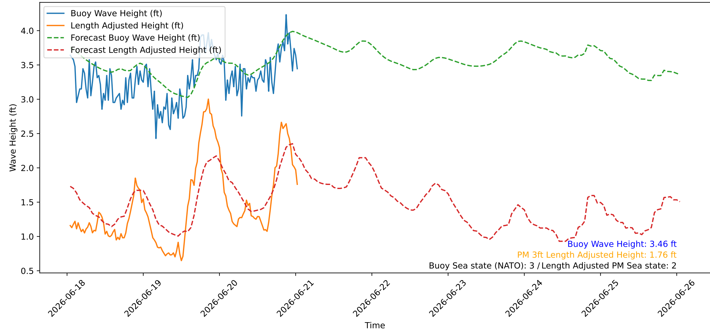
Wave Heights over Time for Green Beach at 2026-06-21 01:11:08
