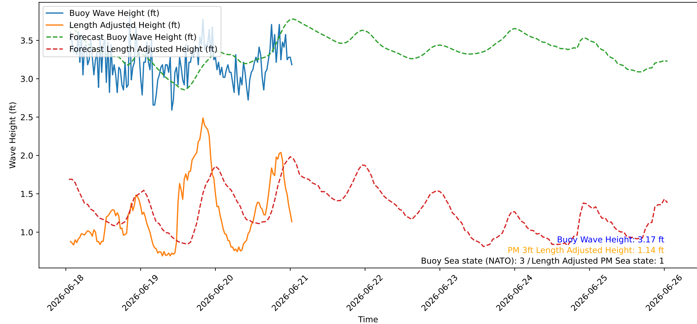
Wave Heights over Time for Red Beach at 2026-06-21 01:10:45
