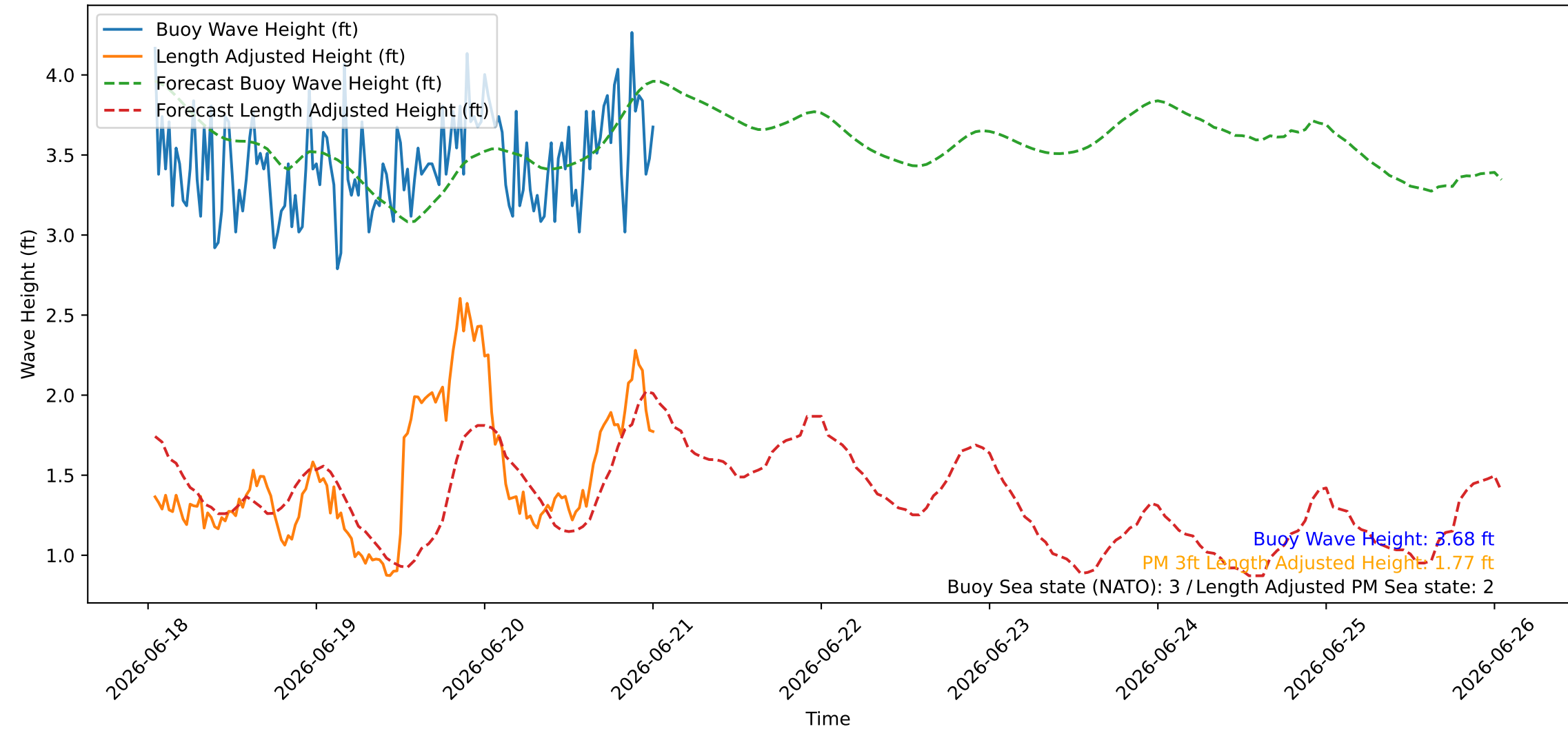
Wave Heights over Time for Oceanside Harbor at 2026-06-21 01:10:26
