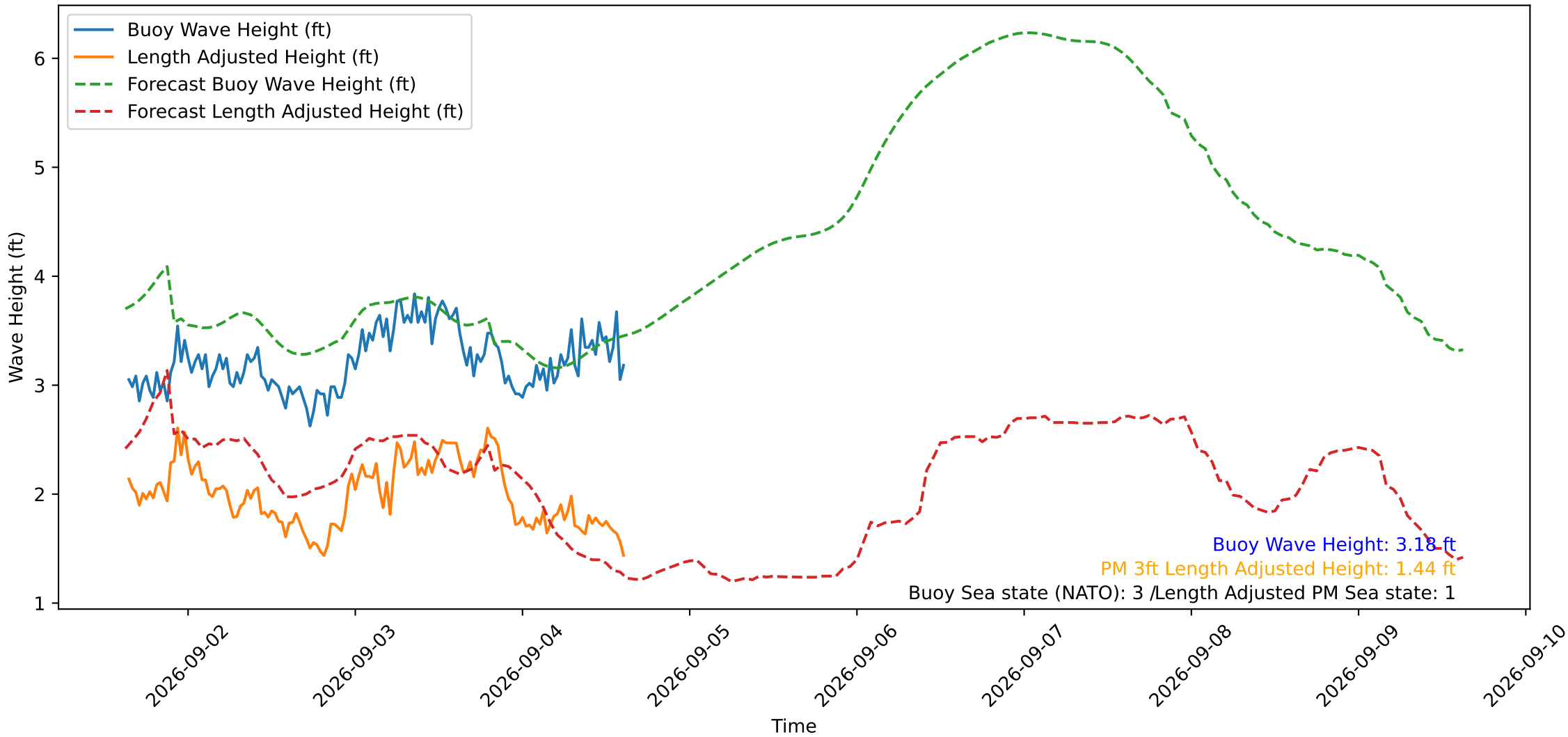
Wave Heights over Time for Oceanside Harbor at 2026-09-04 15:20:30
