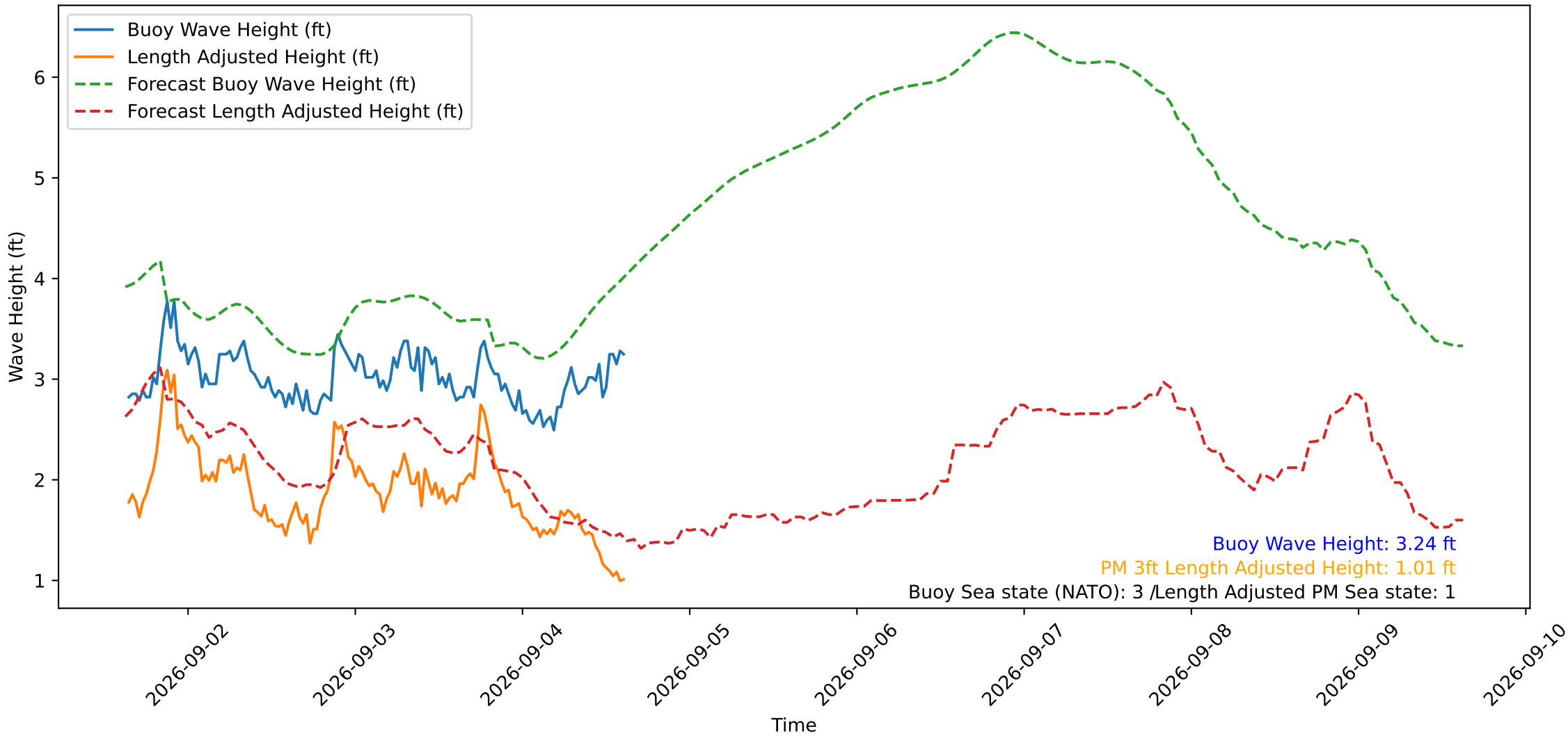
Wave Heights over Time for Green Beach at 2026-09-04 15:21:15
