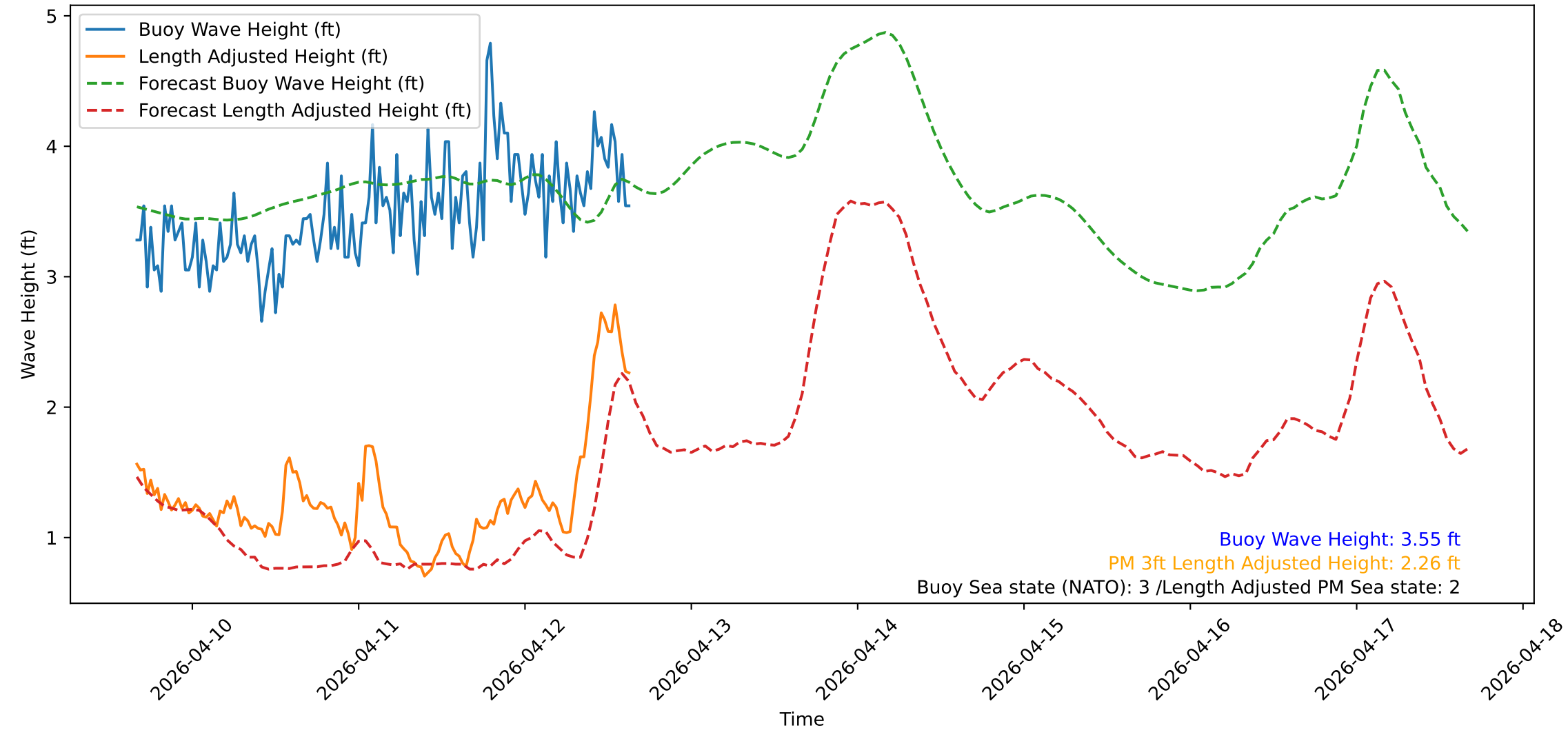
Wave Heights over Time for Oceanside Harbor at 2026-04-12 15:50:31
