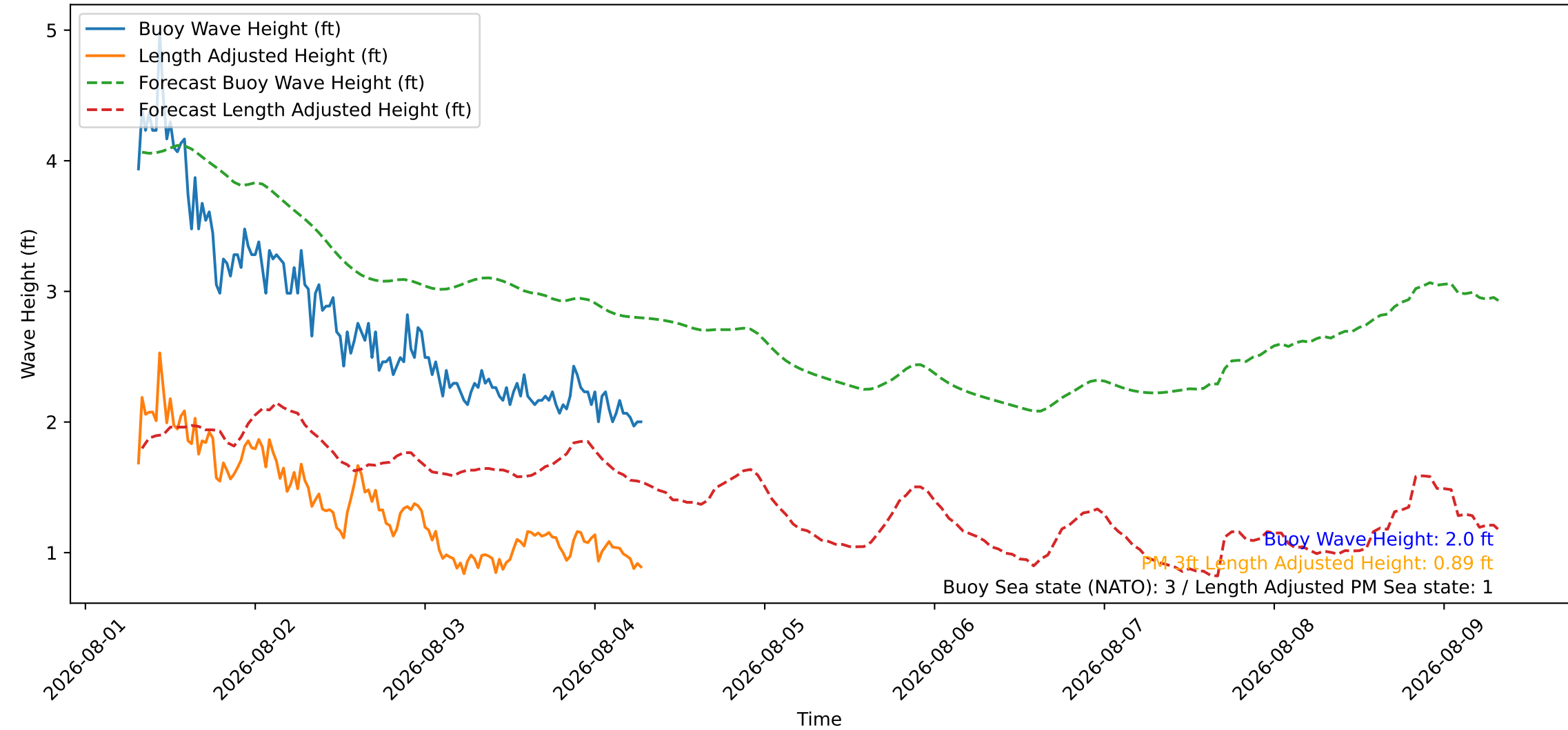
Wave Heights over Time for Green Beach at 2026-08-04 07:31:09
