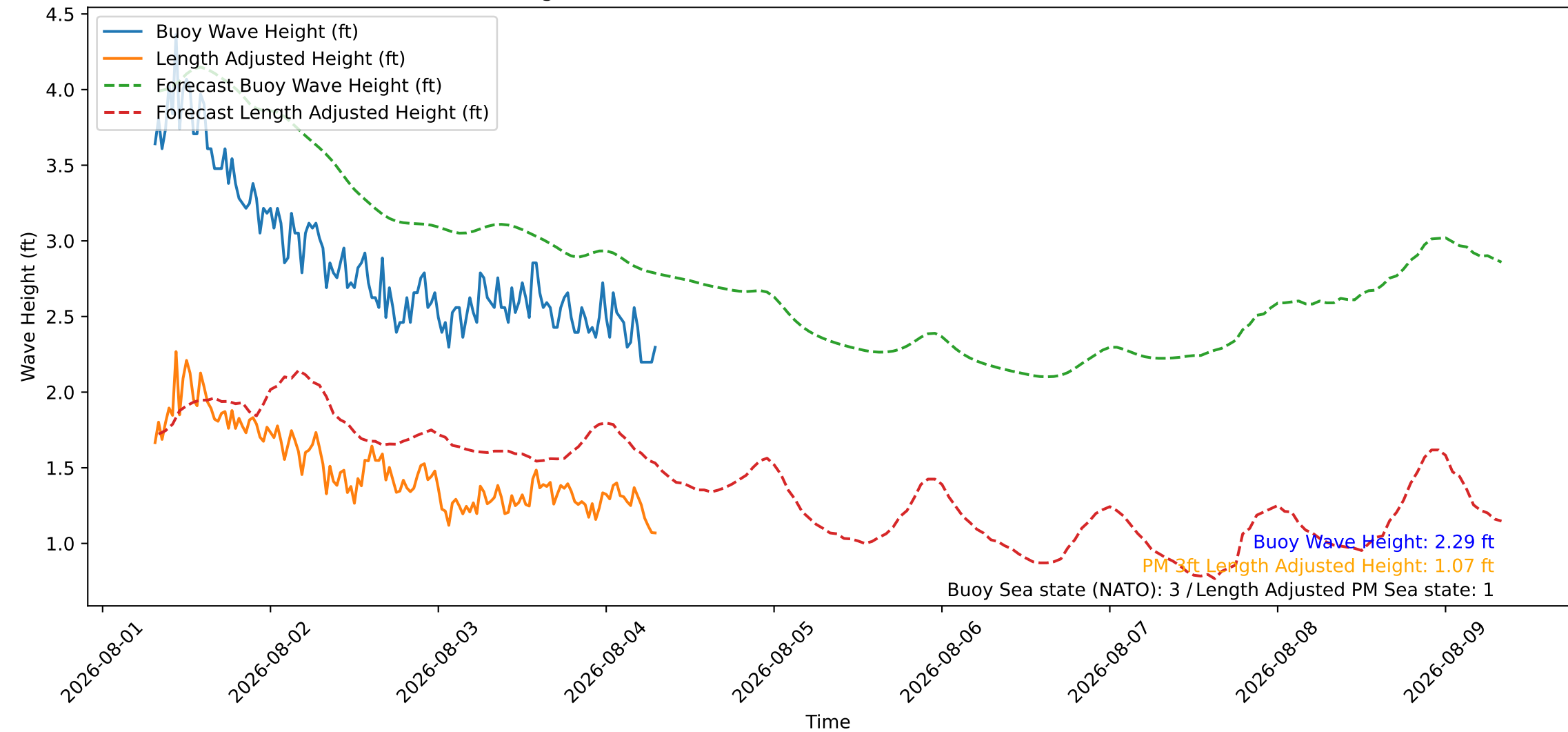
Wave Heights over Time for Oceanside Harbor at 2026-08-04 07:30:27
