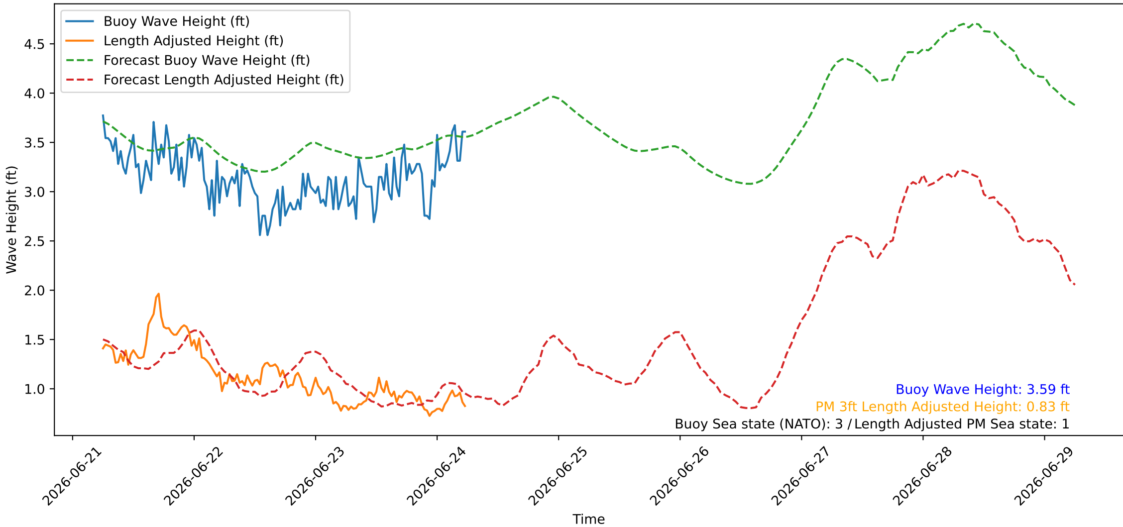
Wave Heights over Time for Oceanside Harbor at 2026-06-24 06:10:26
