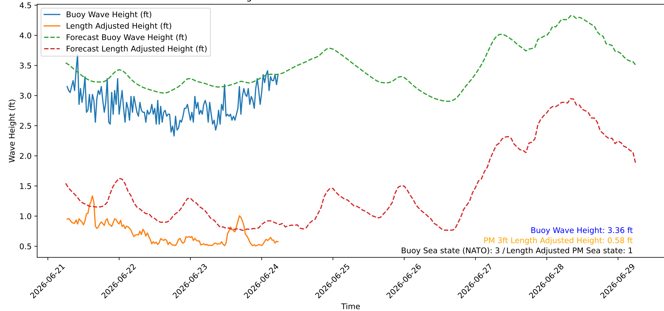
Wave Heights over Time for Red Beach at 2026-06-24 06:10:45
