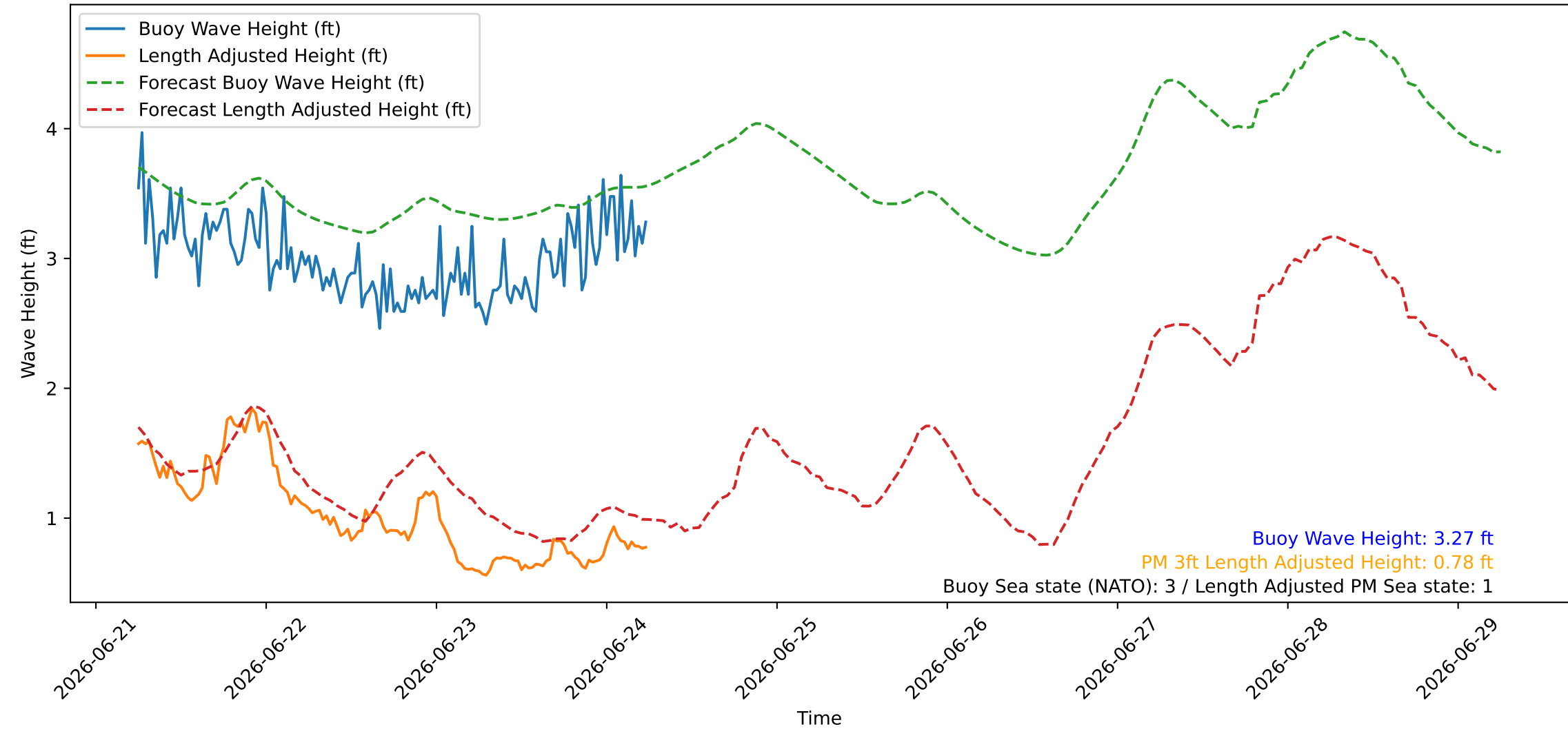
Wave Heights over Time for Green Beach at 2026-06-24 06:11:08
