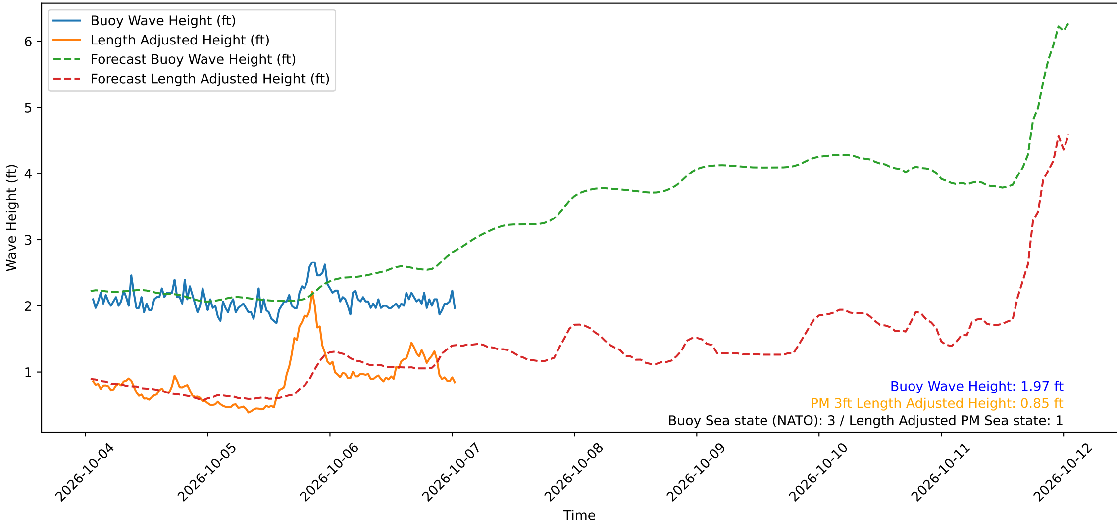
Wave Heights over Time for Red Beach at 2026-10-07 01:20:50
