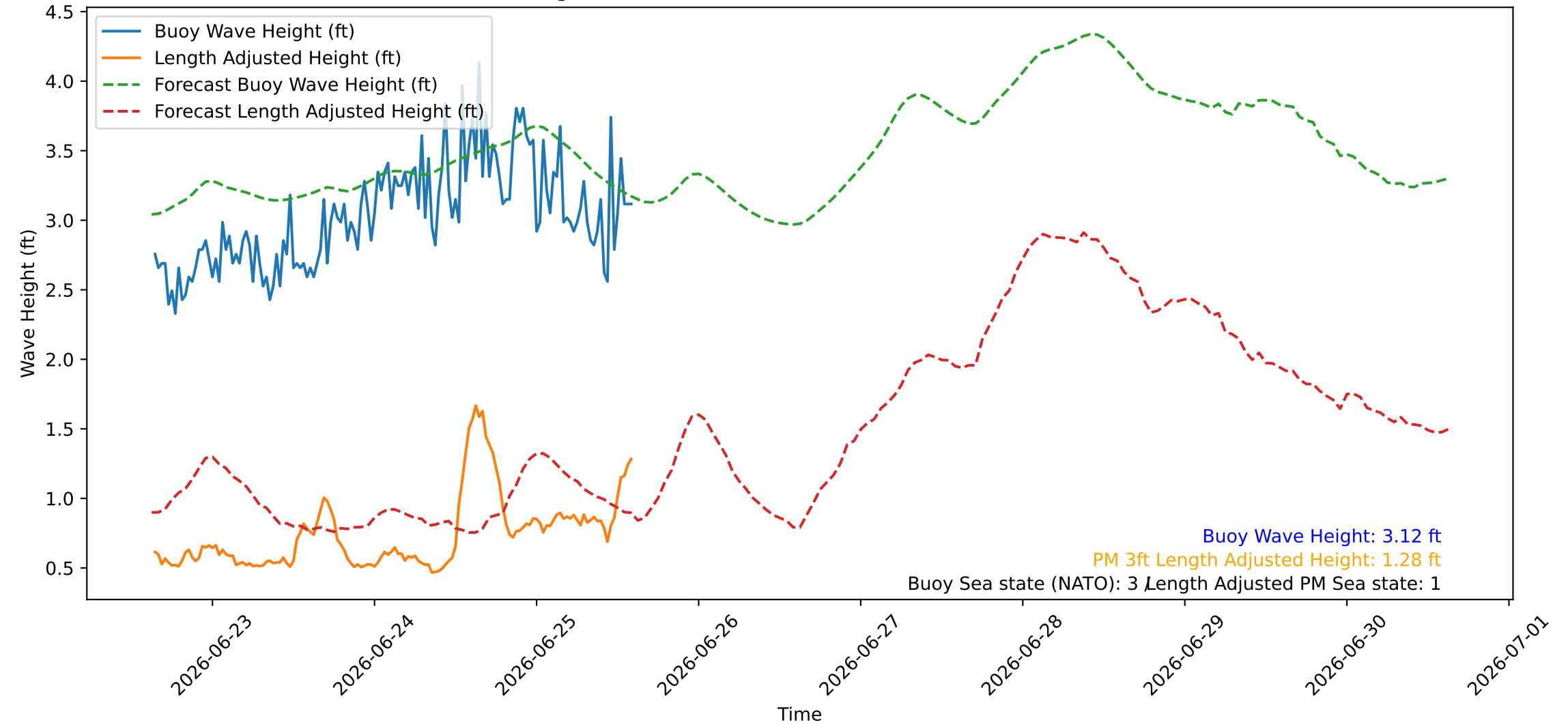
Wave Heights over Time for Red Beach at 2026-06-25 15:00:45
