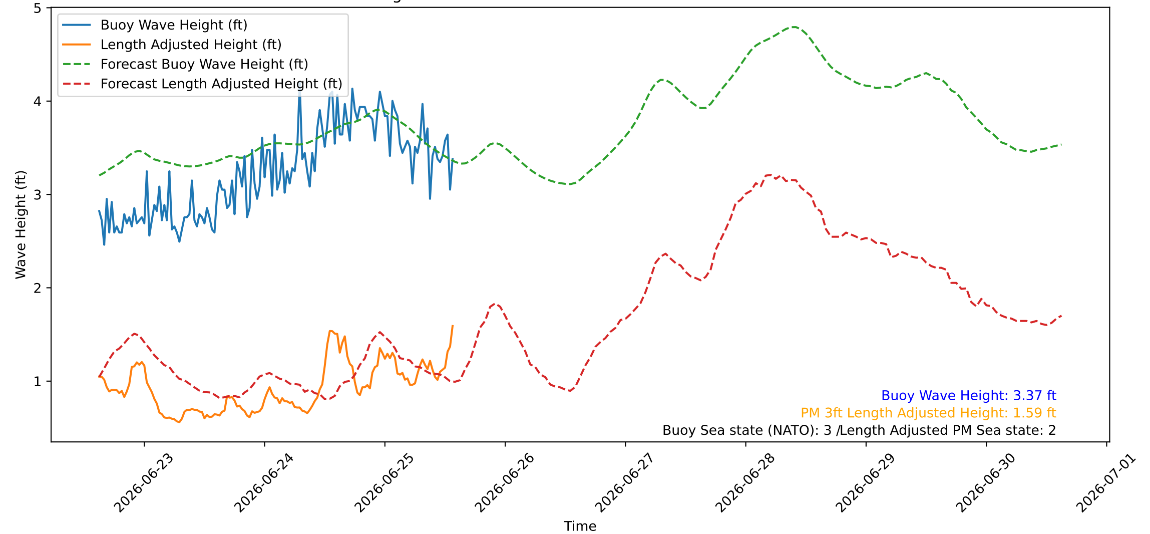
Wave Heights over Time for Green Beach at 2026-06-25 15:01:08
