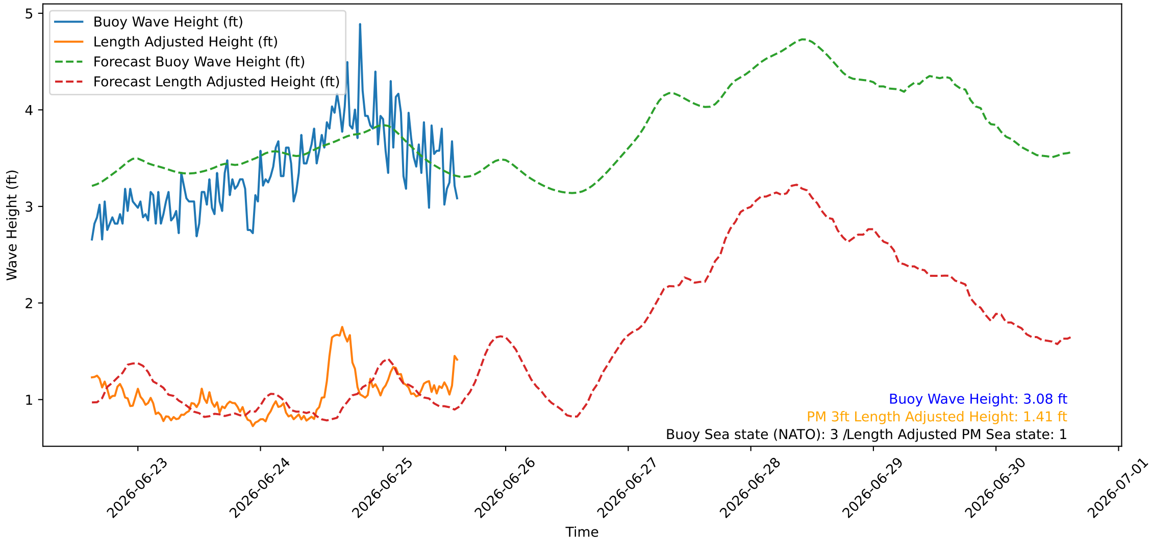
Wave Heights over Time for Oceanside Harbor at 2026-06-25 15:00:26
