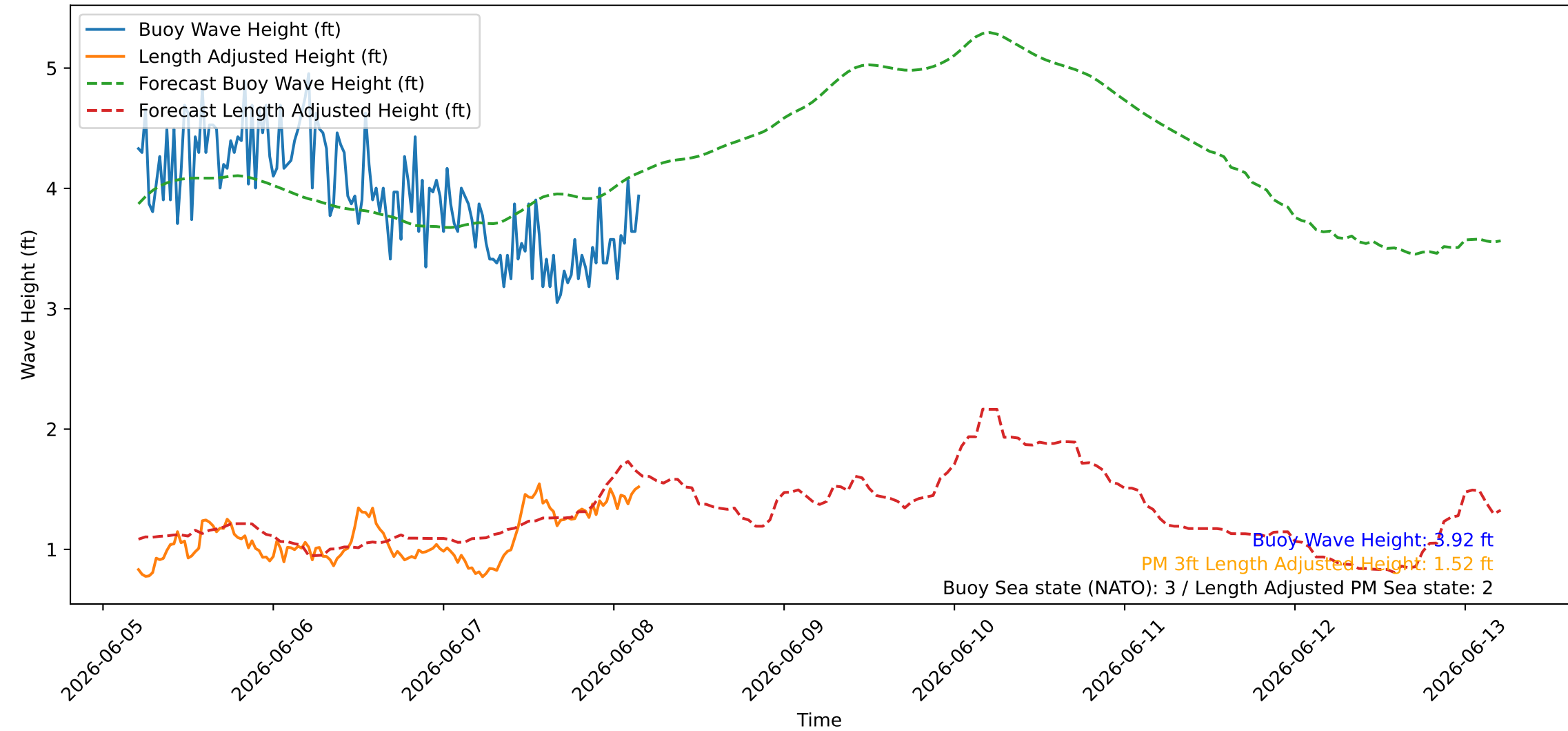
Wave Heights over Time for Red Beach at 2026-06-08 04:30:46
