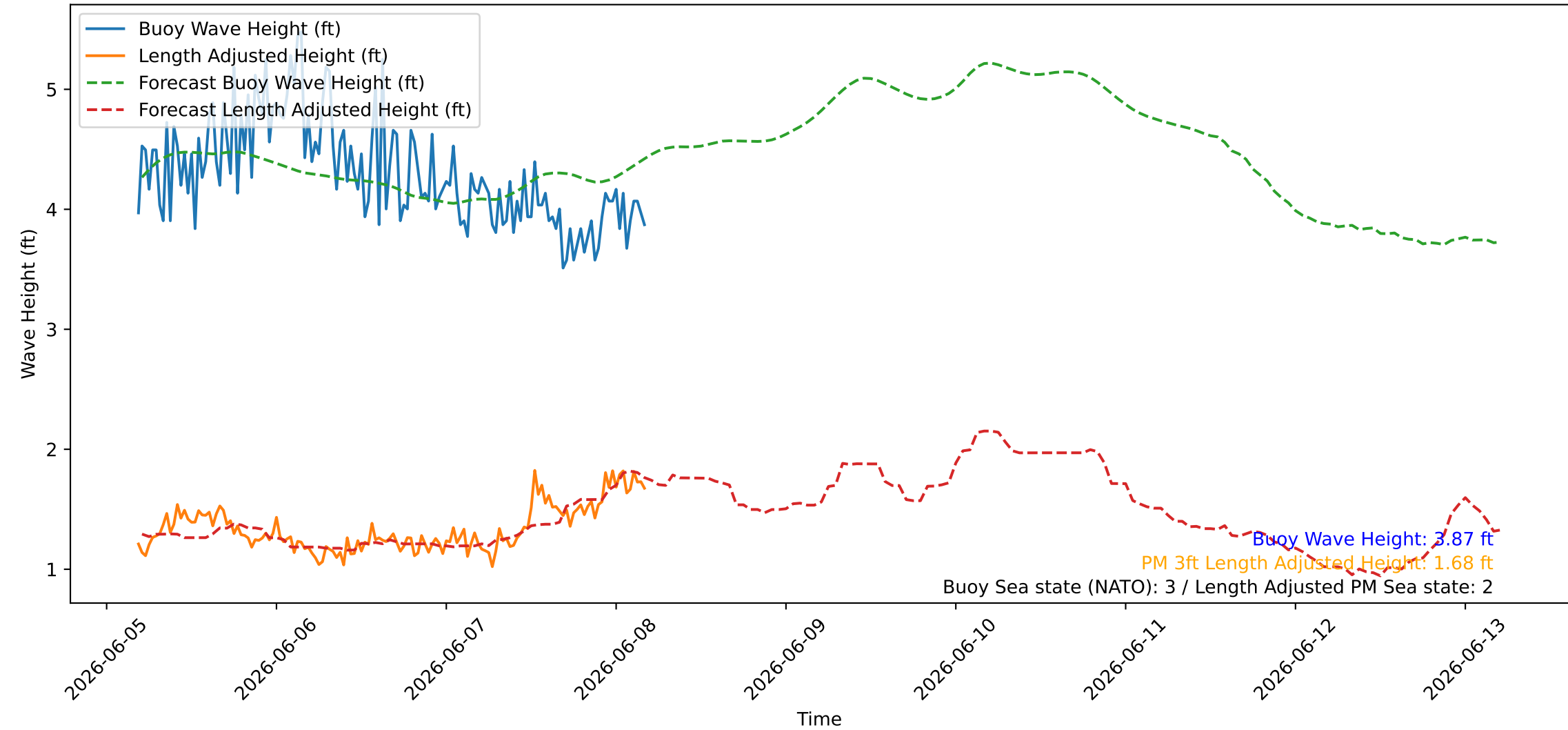
Wave Heights over Time for Oceanside Harbor at 2026-06-08 04:30:27
