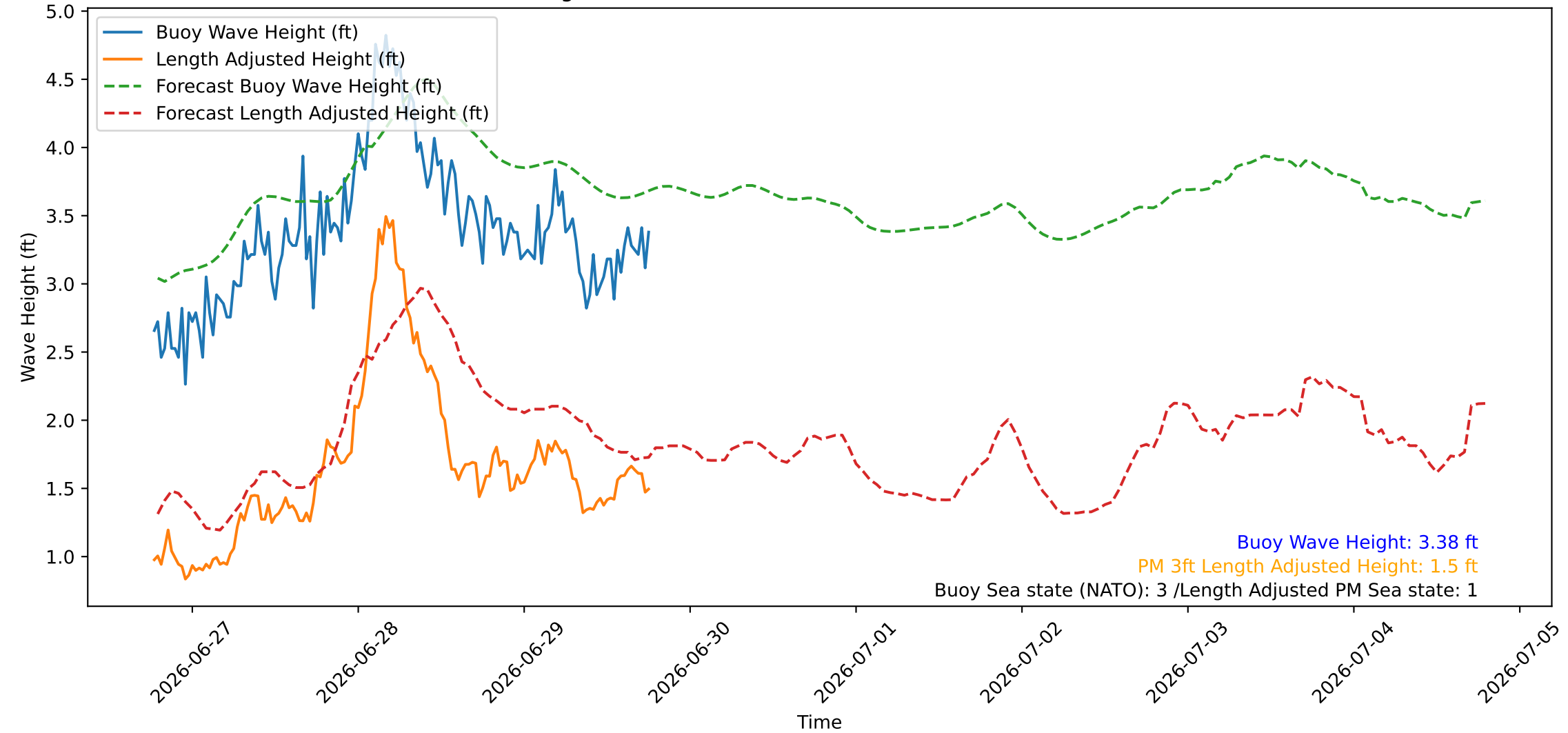
Wave Heights over Time for Green Beach at 2026-06-29 18:41:08
