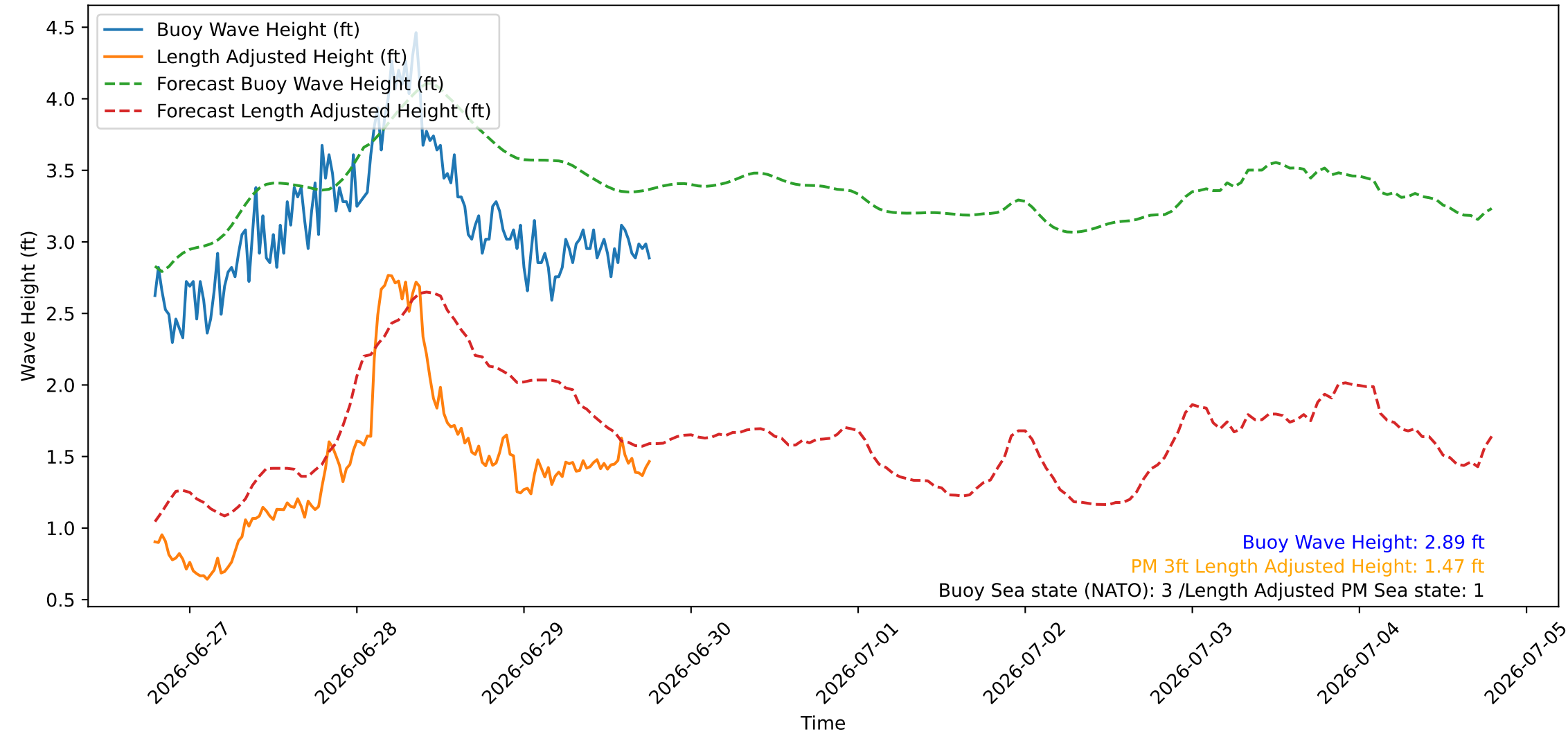
Wave Heights over Time for Red Beach at 2026-06-29 18:40:46
