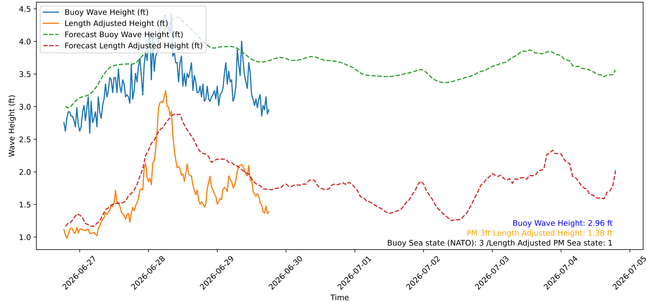
Wave Heights over Time for Oceanside Harbor at 2026-06-29 18:40:26
