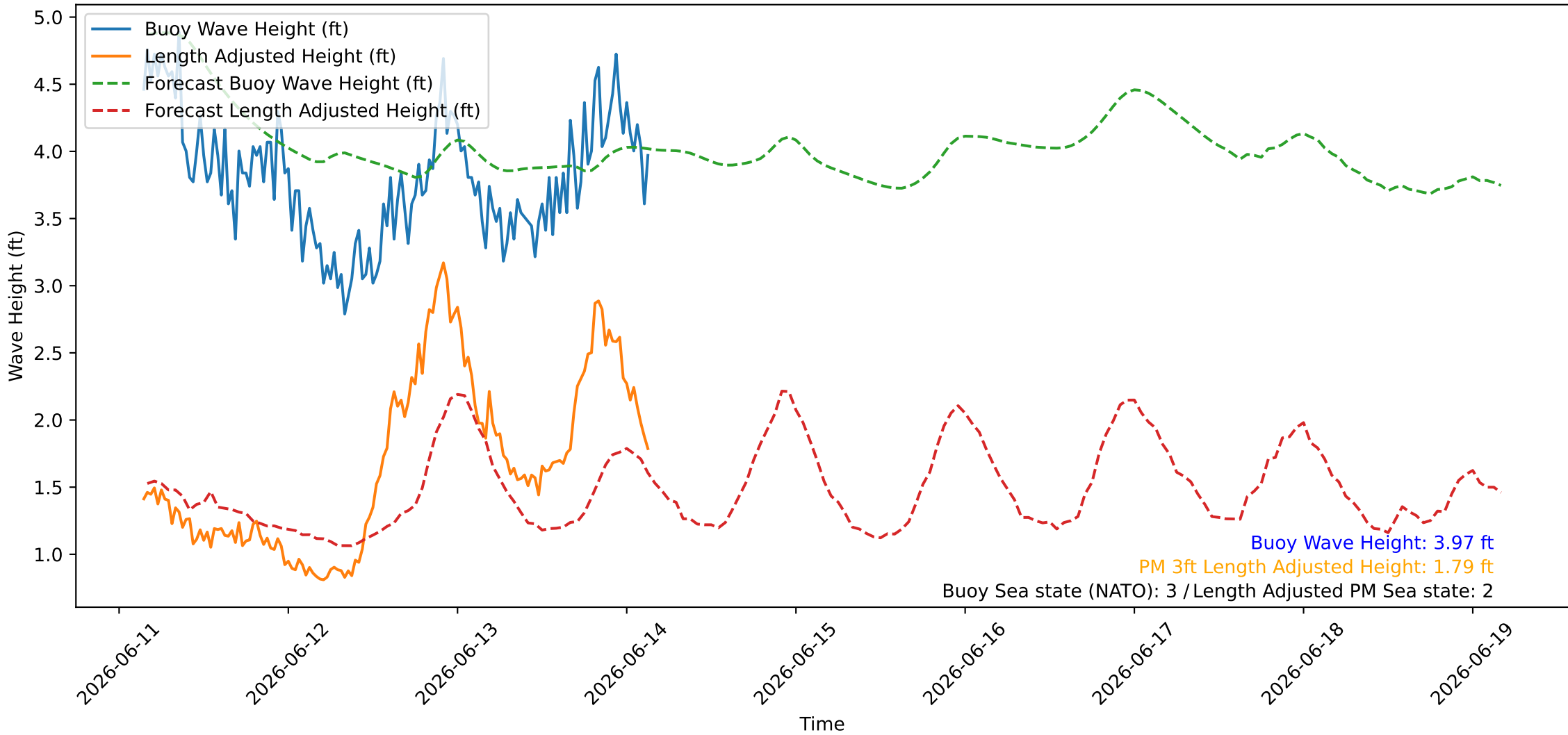
Wave Heights over Time for Oceanside Harbor at 2026-06-14 03:40:26
