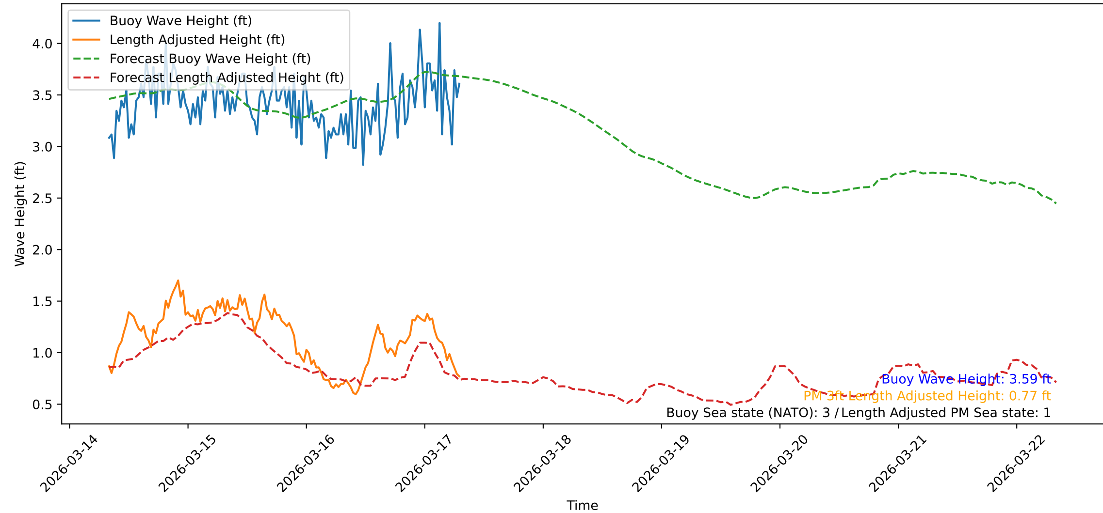
Wave Heights over Time for Green Beach at 2026-03-17 07:51:51
