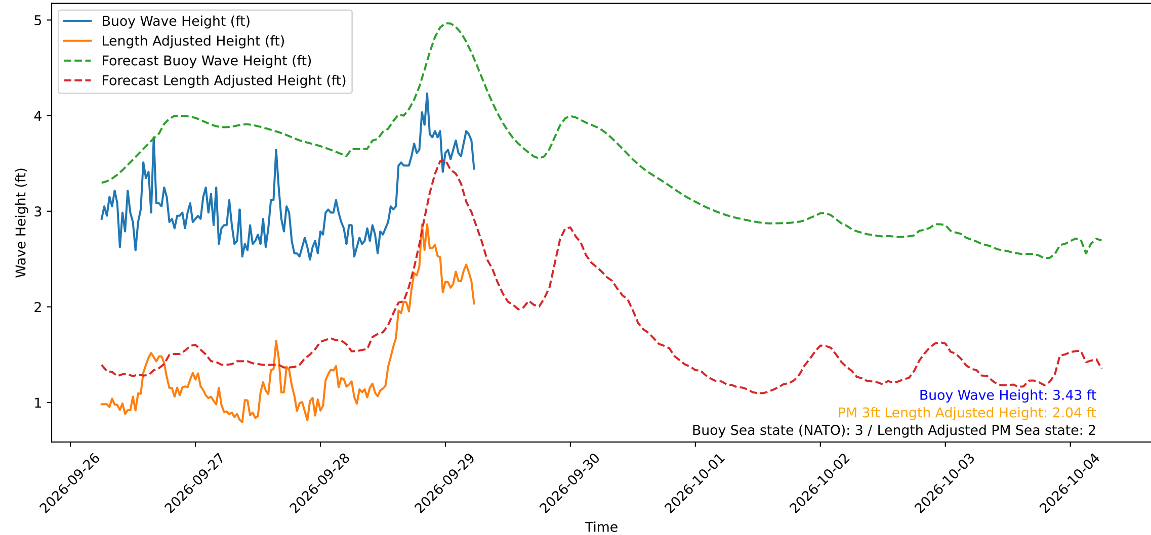
Wave Heights over Time for Oceanside Harbor at 2026-09-29 06:10:30
