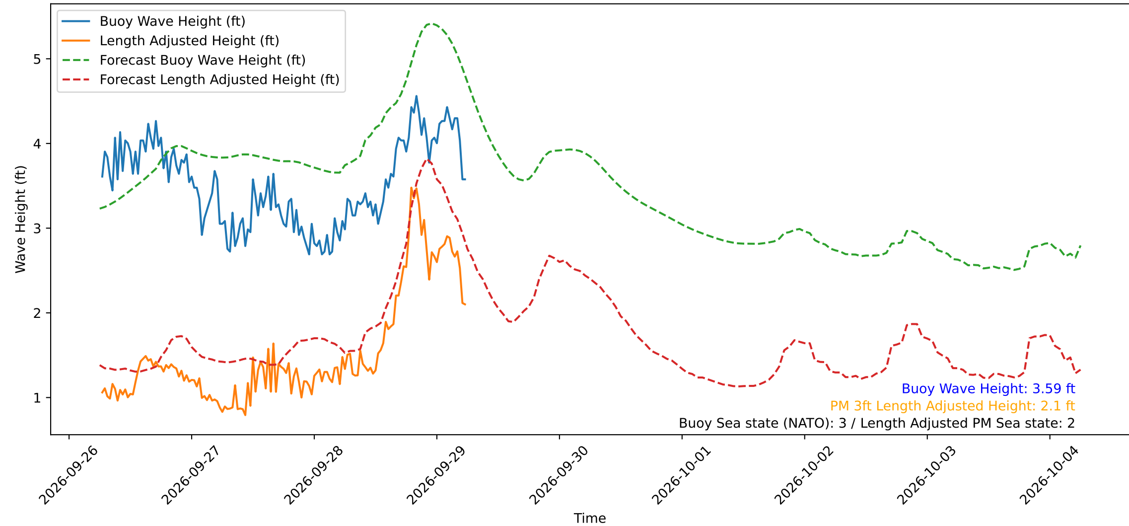
Wave Heights over Time for Green Beach at 2026-09-29 06:11:12
