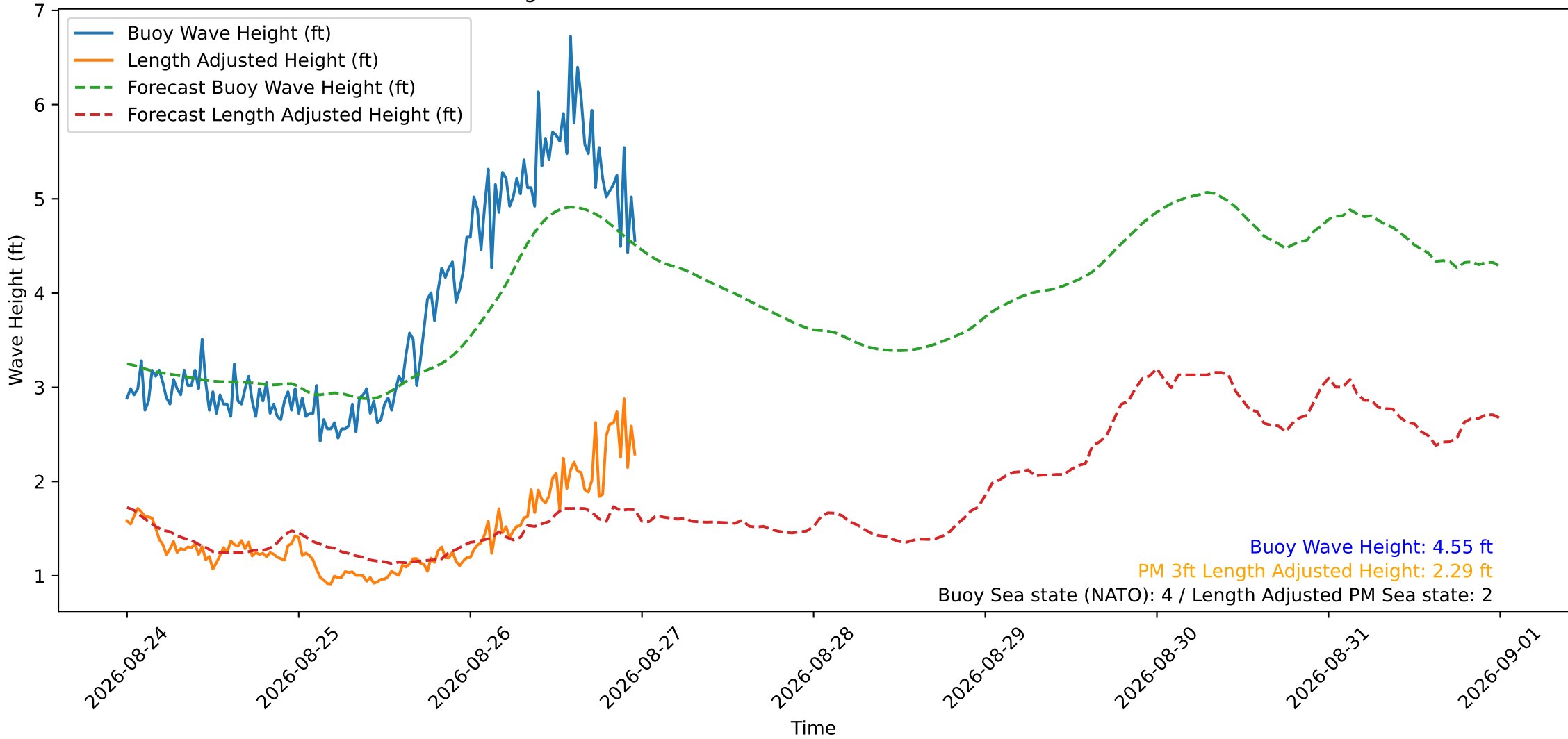
Wave Heights over Time for Oceanside Harbor at 2026-08-26 23:50:29
