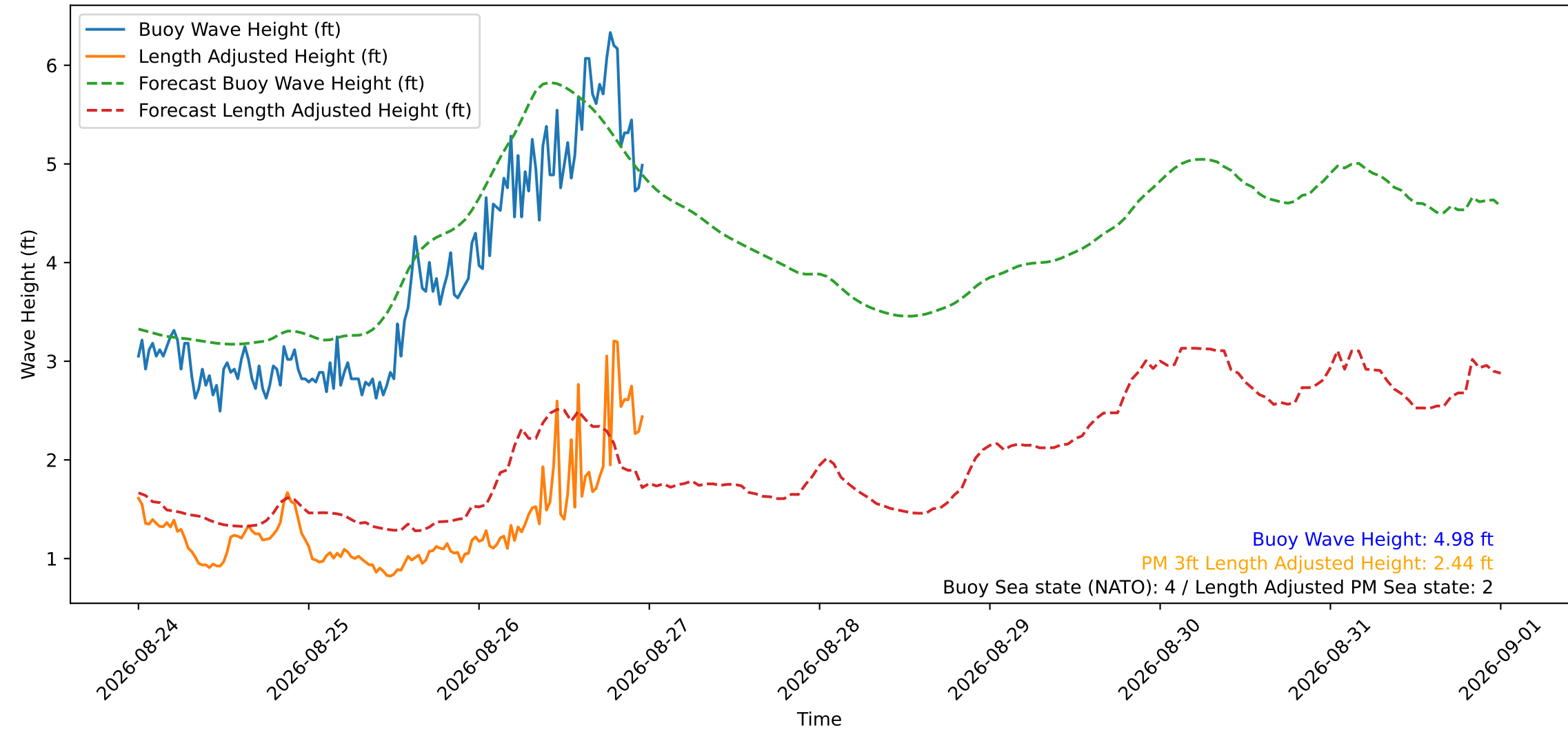
Wave Heights over Time for Green Beach at 2026-08-26 23:51:15
