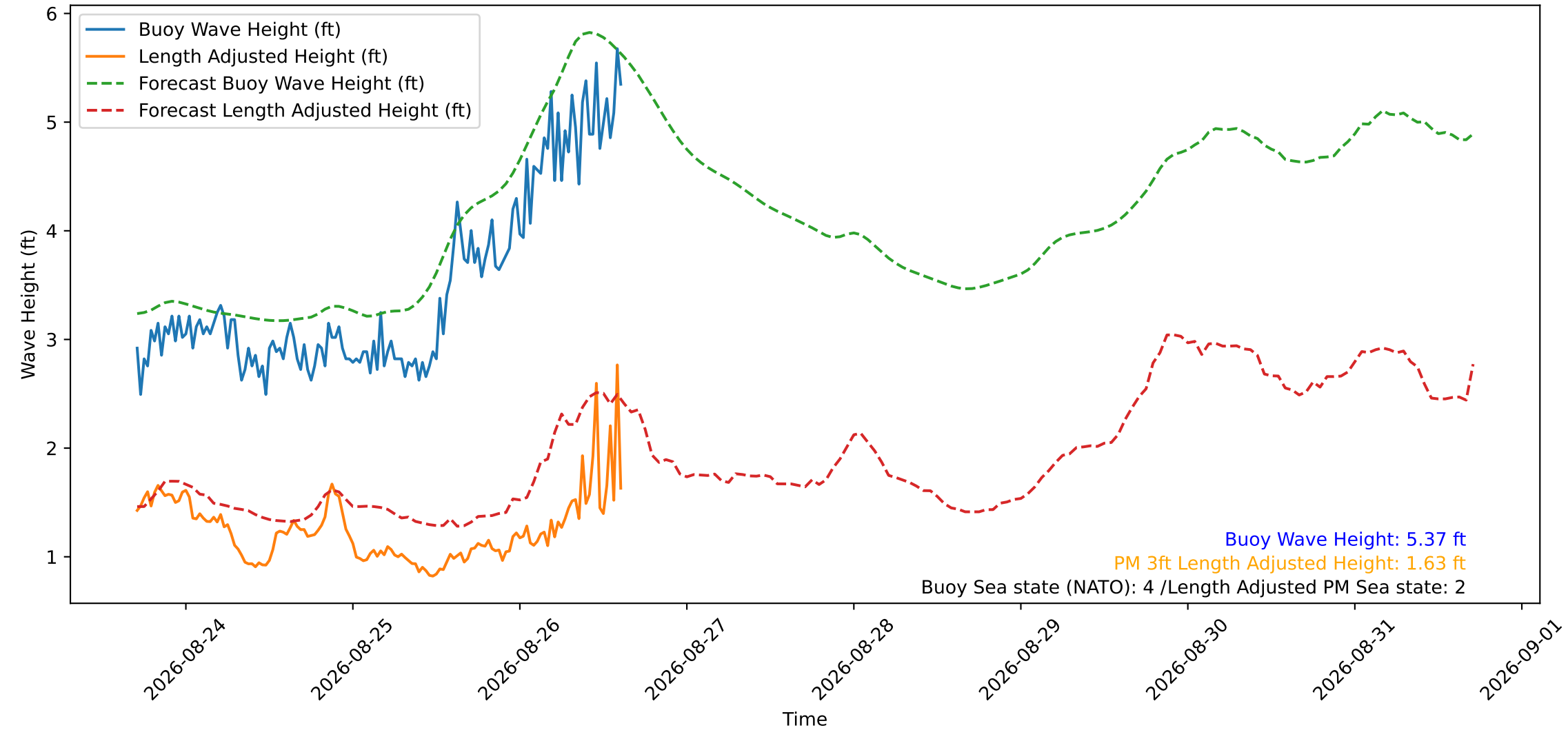
Wave Heights over Time for Green Beach at 2026-08-26 16:51:15
