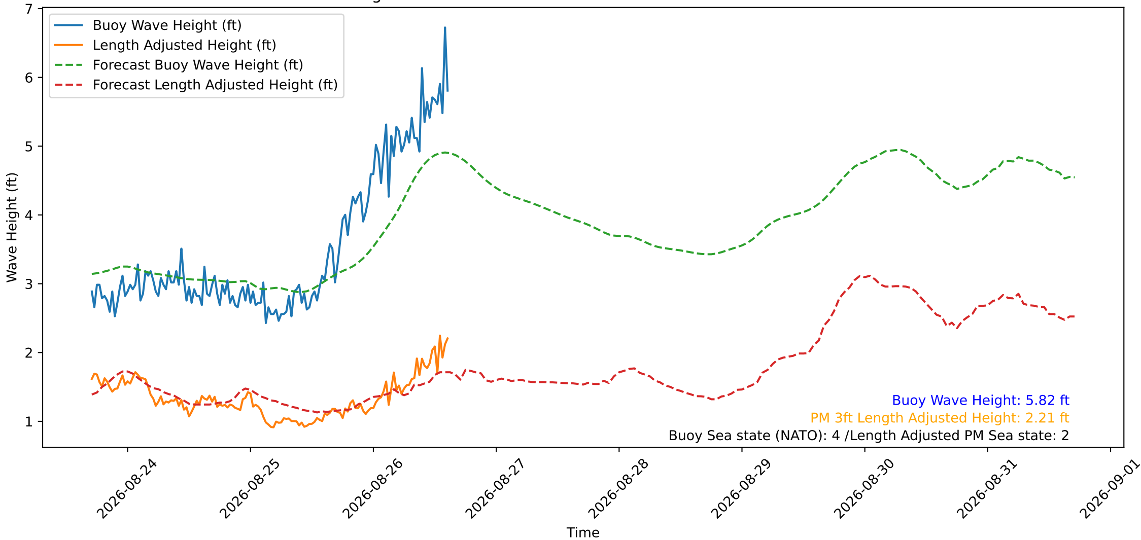
Wave Heights over Time for Oceanside Harbor at 2026-08-26 16:50:30
