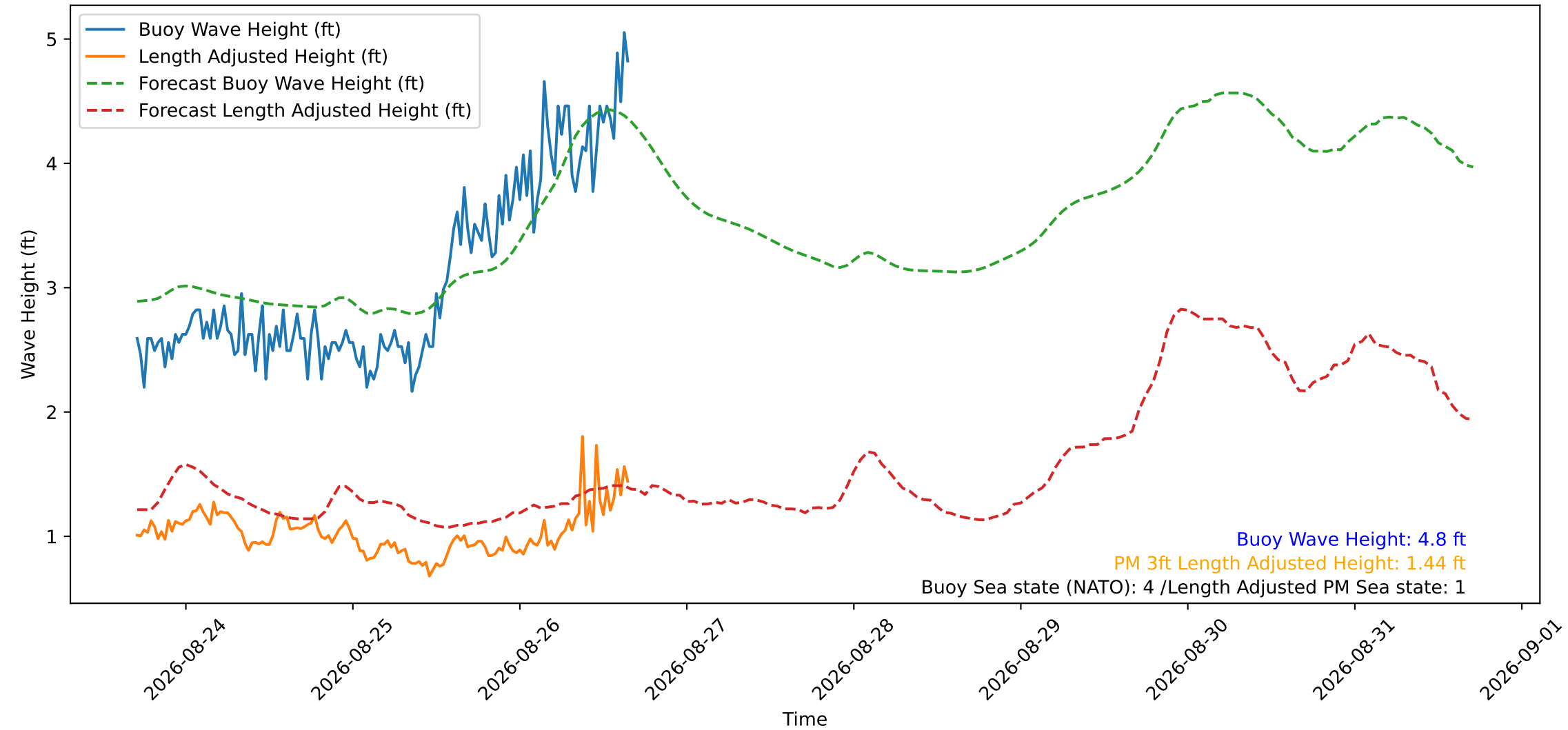
Wave Heights over Time for Red Beach at 2026-08-26 16:50:50
