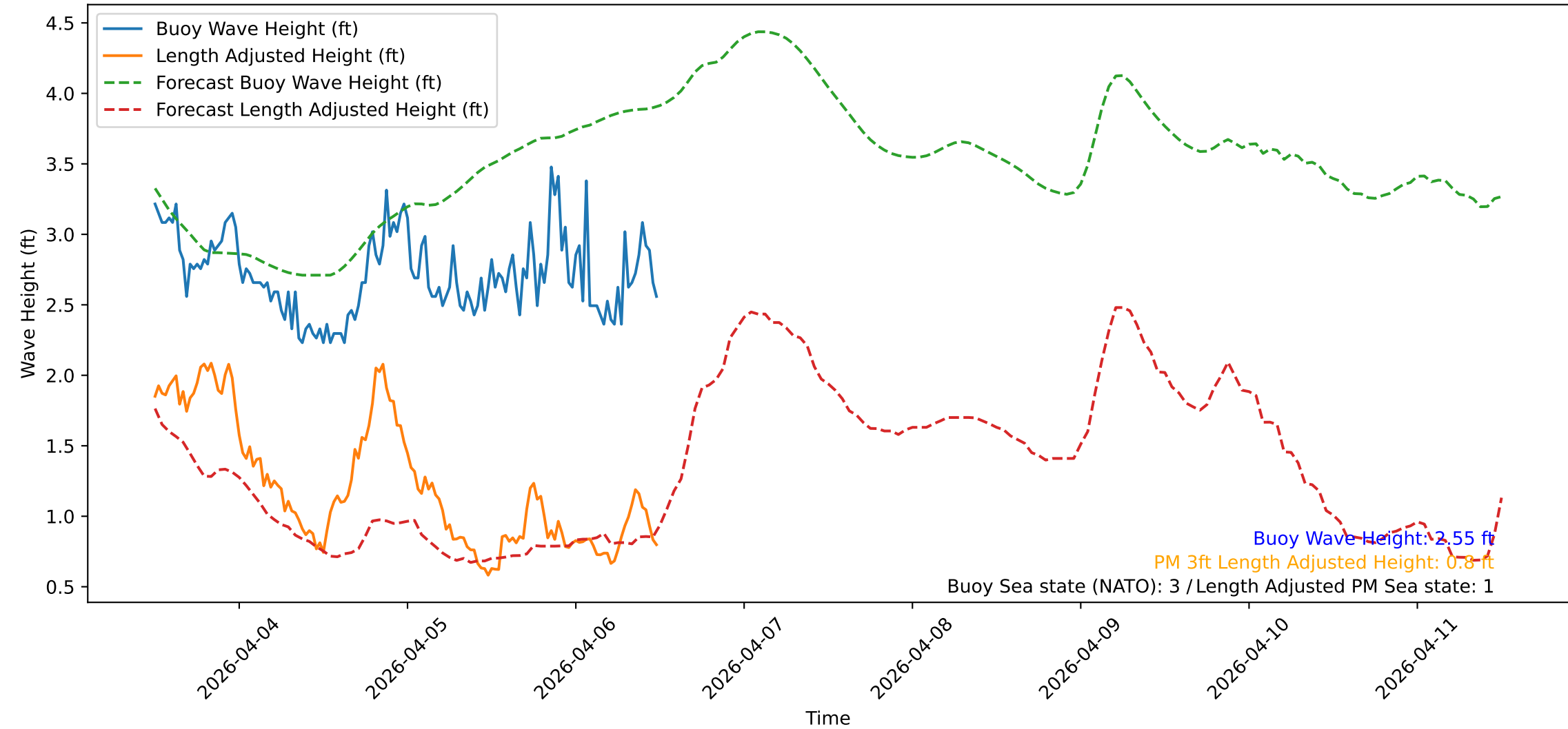
Wave Heights over Time for Green Beach at 2026-04-06 12:11:11
