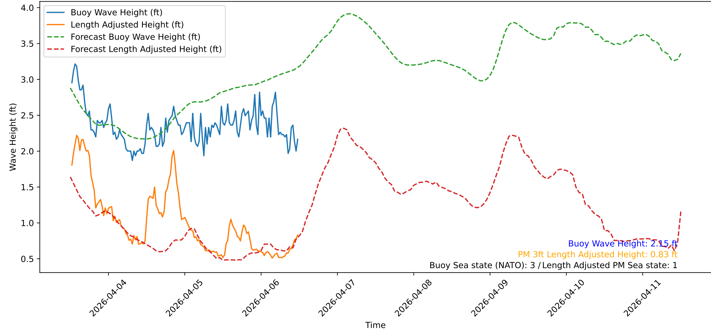
Wave Heights over Time for Red Beach at 2026-04-06 12:10:48
