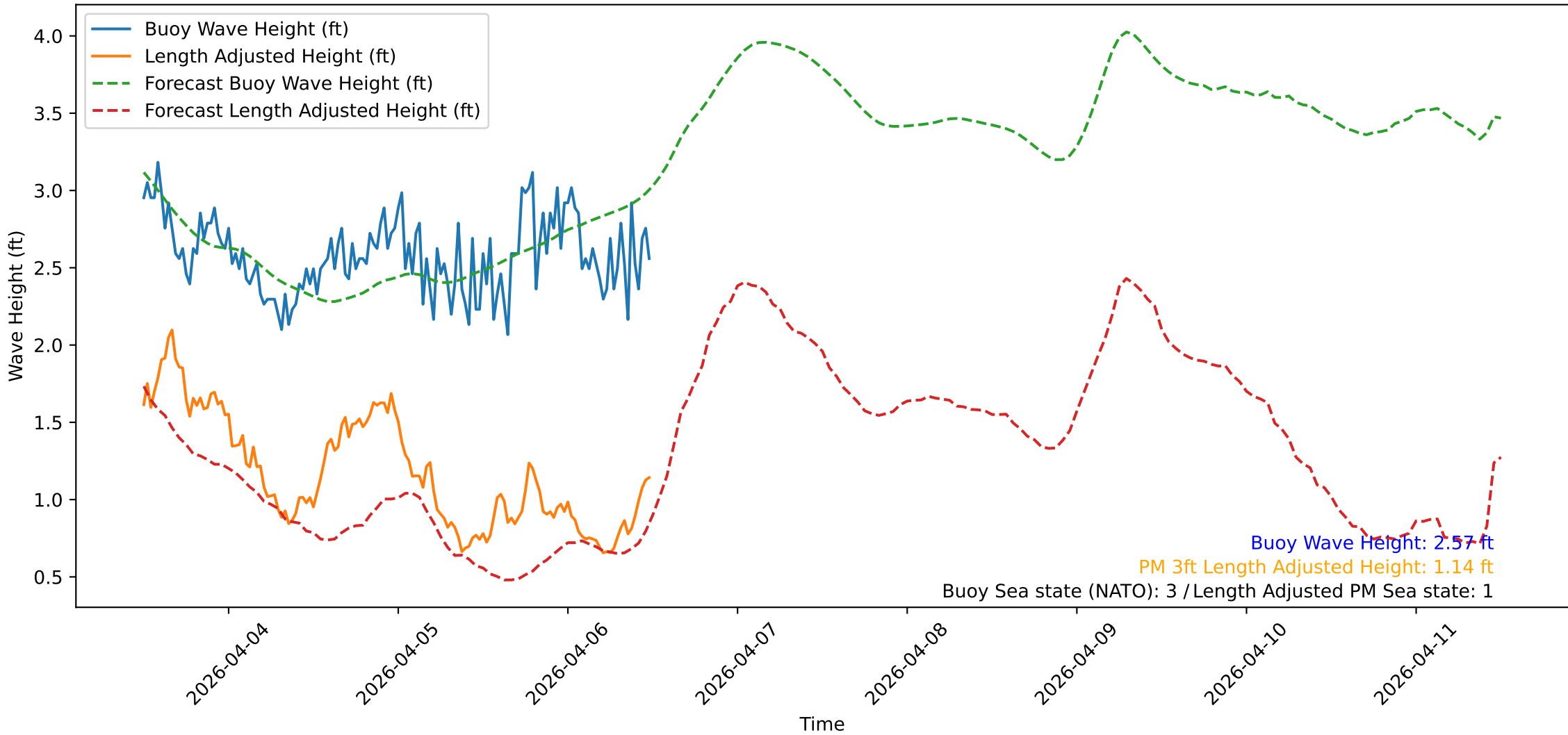
Wave Heights over Time for Oceanside Harbor at 2026-04-06 12:10:32
