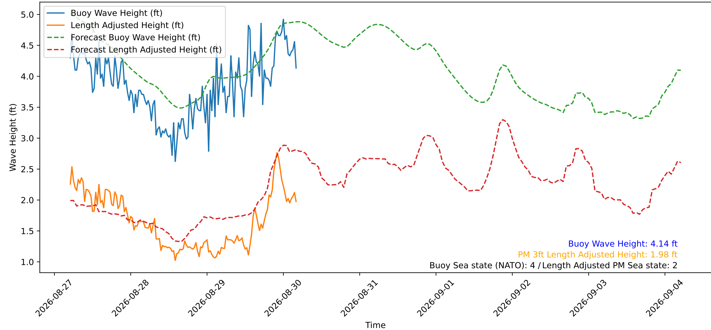
Wave Heights over Time for Green Beach at 2026-08-30 04:51:15
