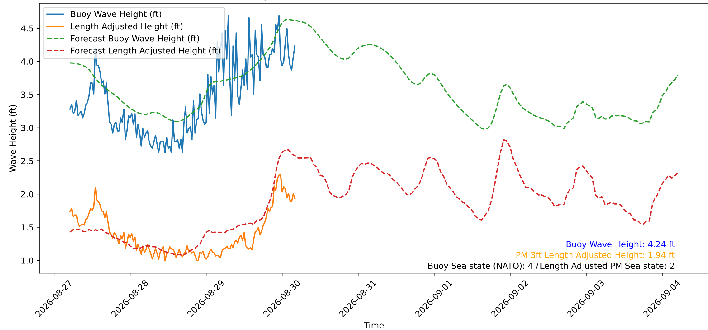
Wave Heights over Time for Red Beach at 2026-08-30 04:50:51
