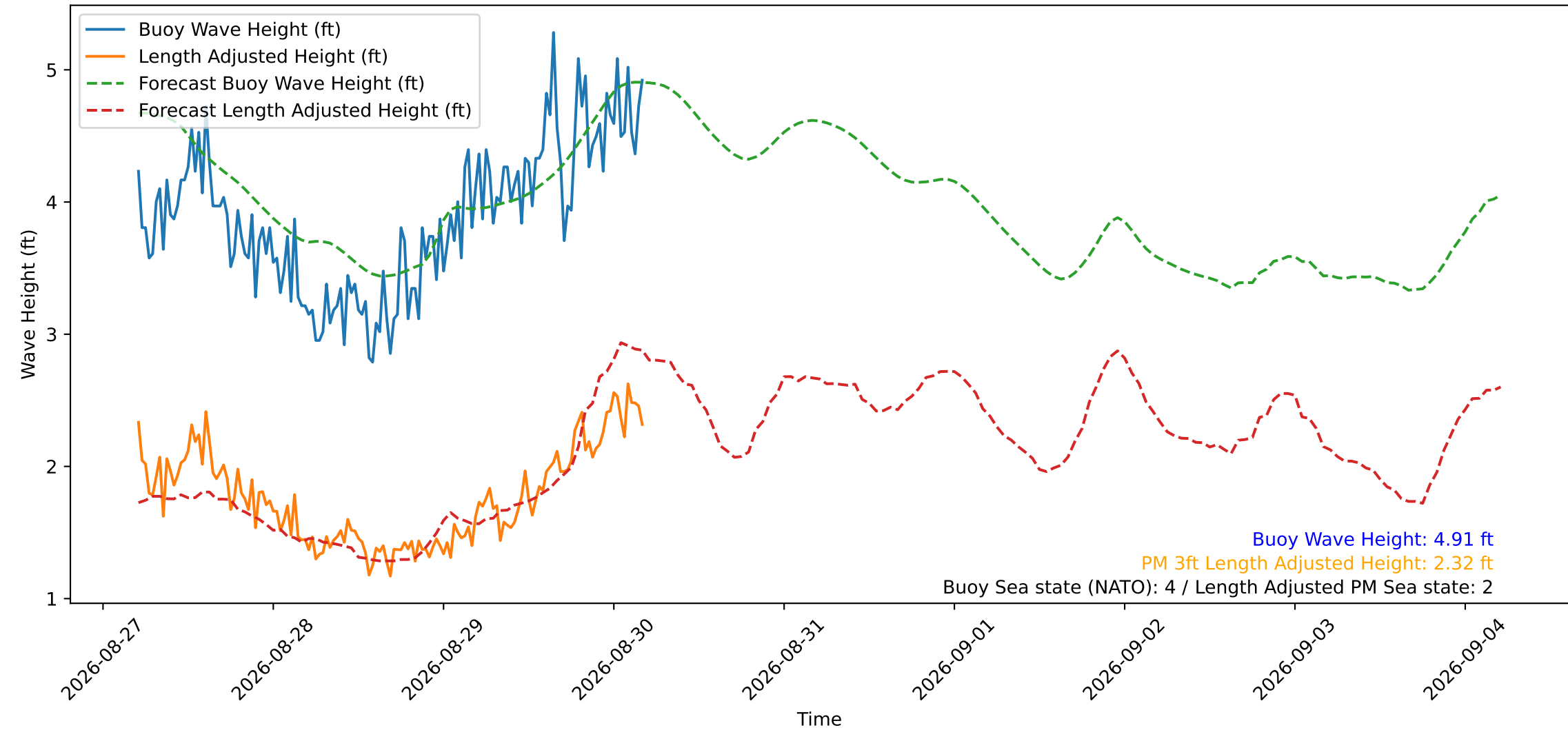
Wave Heights over Time for Oceanside Harbor at 2026-08-30 04:50:30
