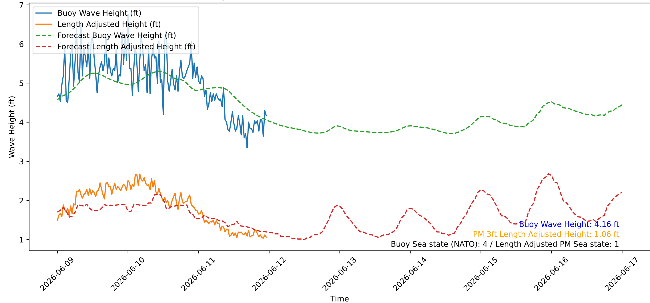
Wave Heights over Time for Oceanside Harbor at 2026-06-12 00:00:26
