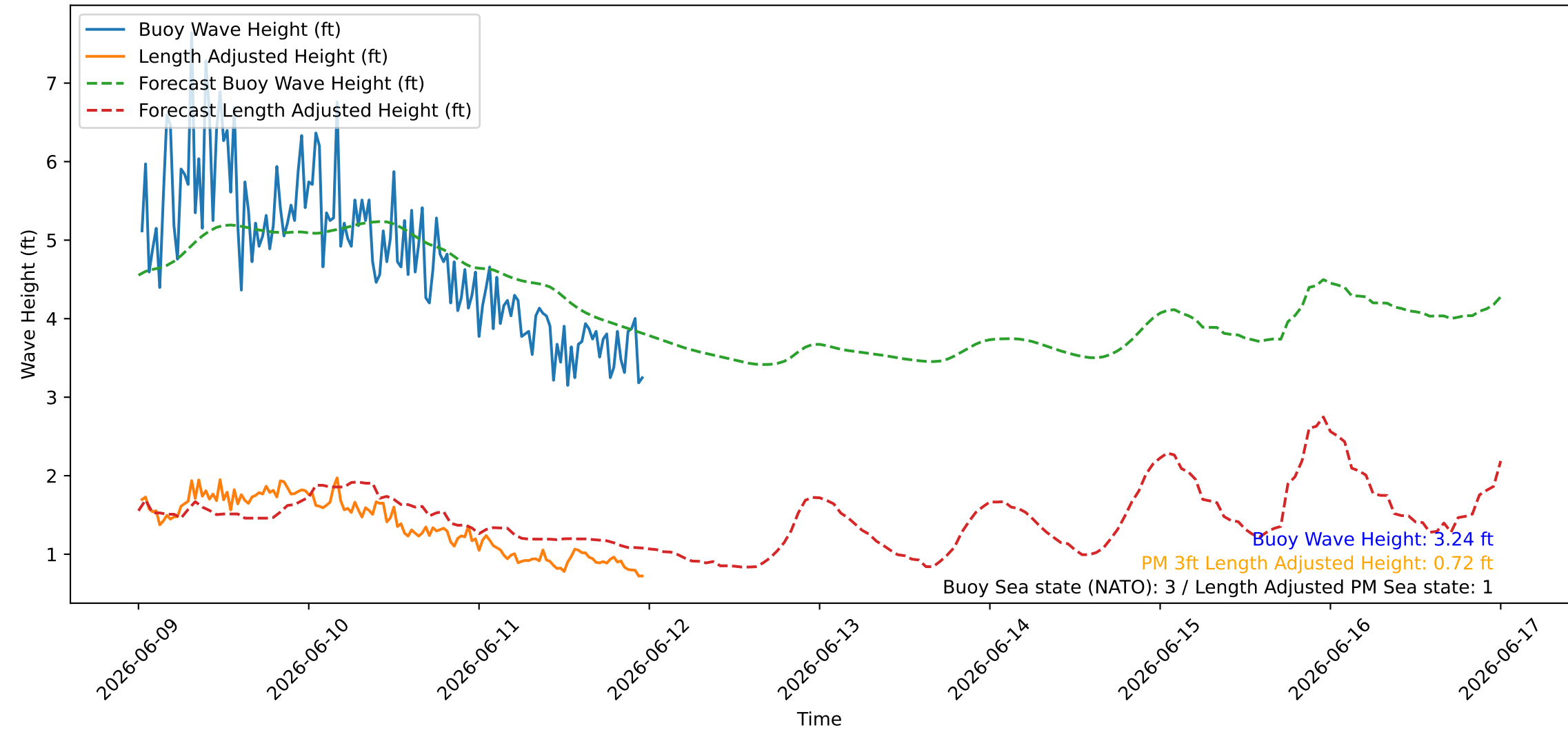
Wave Heights over Time for Red Beach at 2026-06-12 00:00:45
