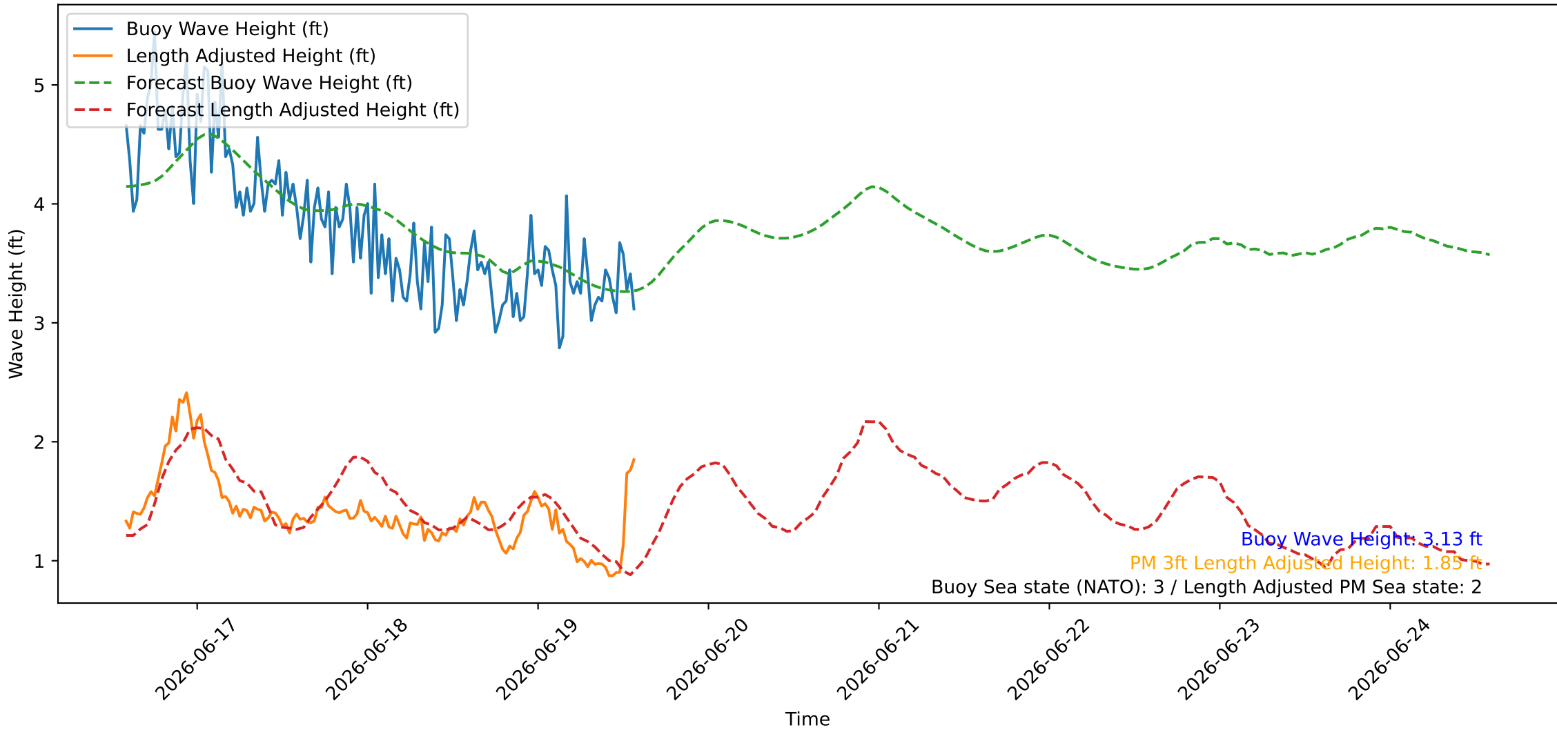
Wave Heights over Time for Oceanside Harbor at 2026-06-19 14:00:26
