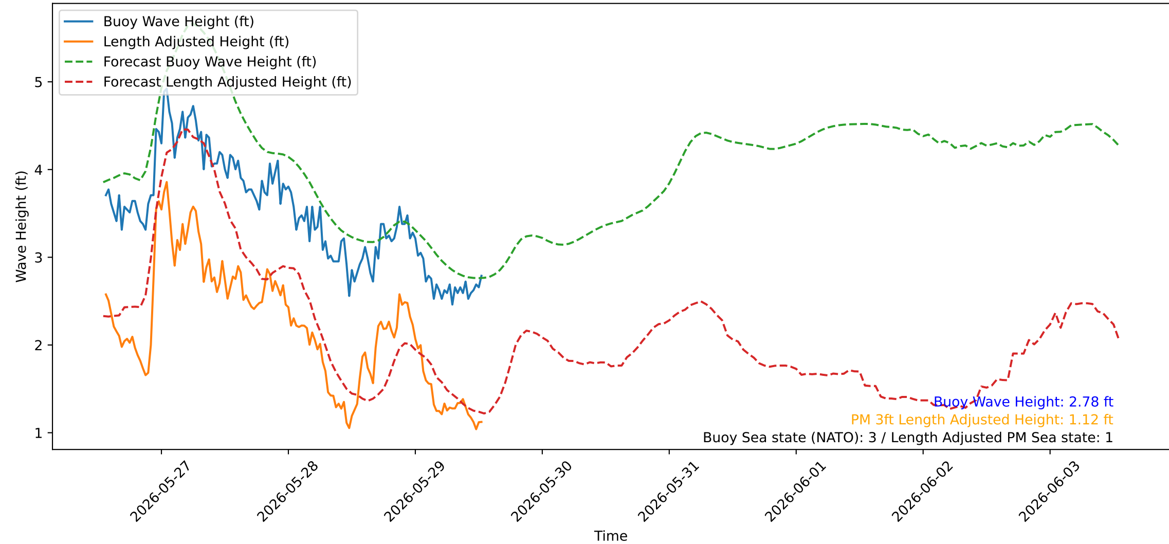
Wave Heights over Time for Green Beach at 2026-05-29 13:21:05
