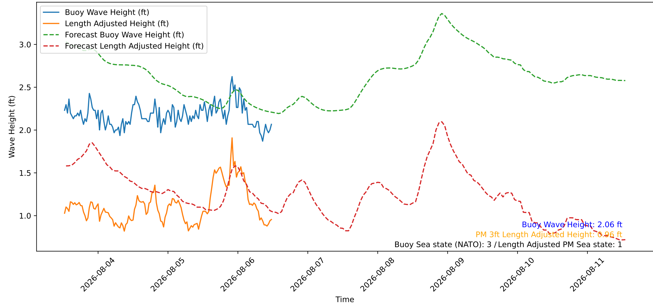
Wave Heights over Time for Green Beach at 2026-08-06 12:31:07
