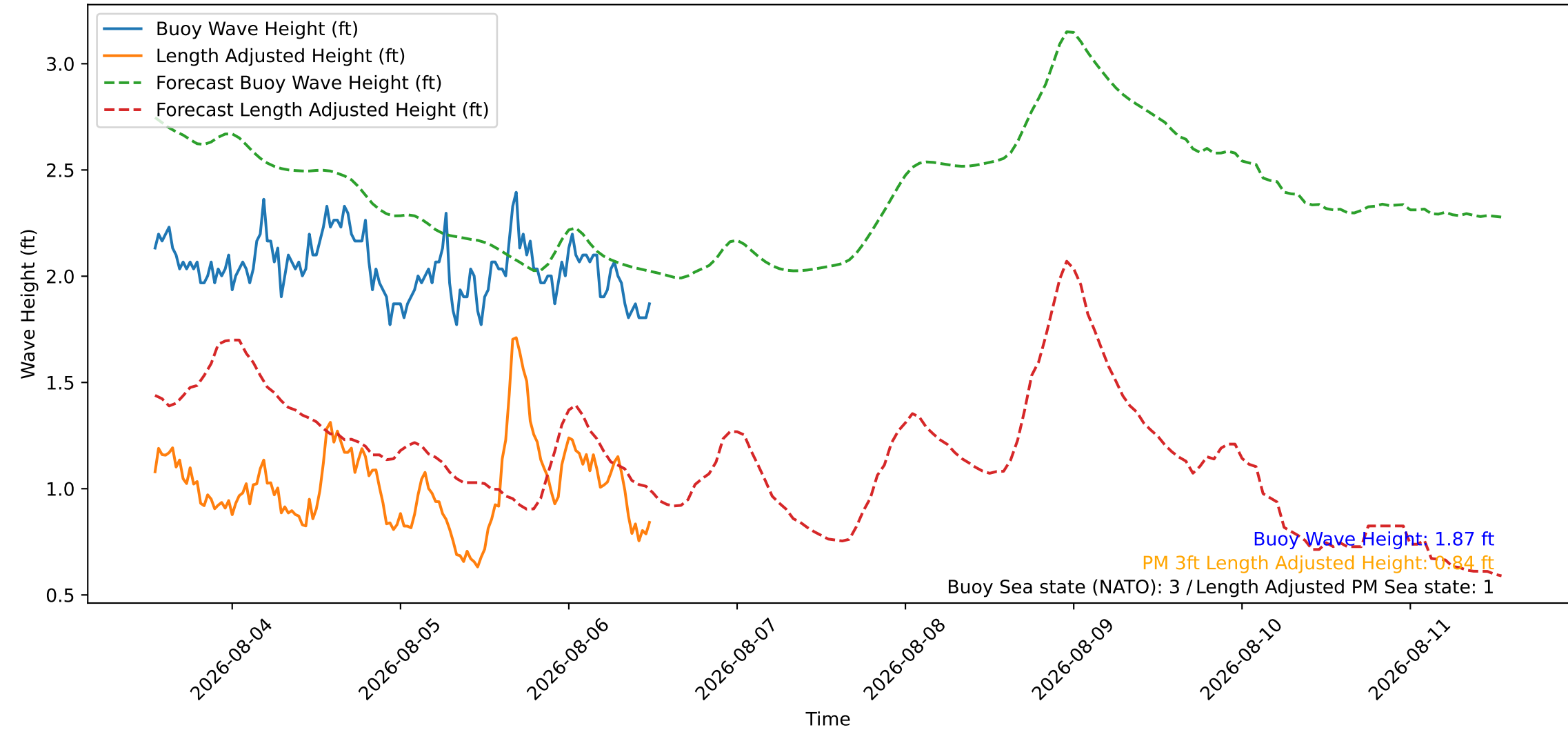
Wave Heights over Time for Red Beach at 2026-08-06 12:30:45
