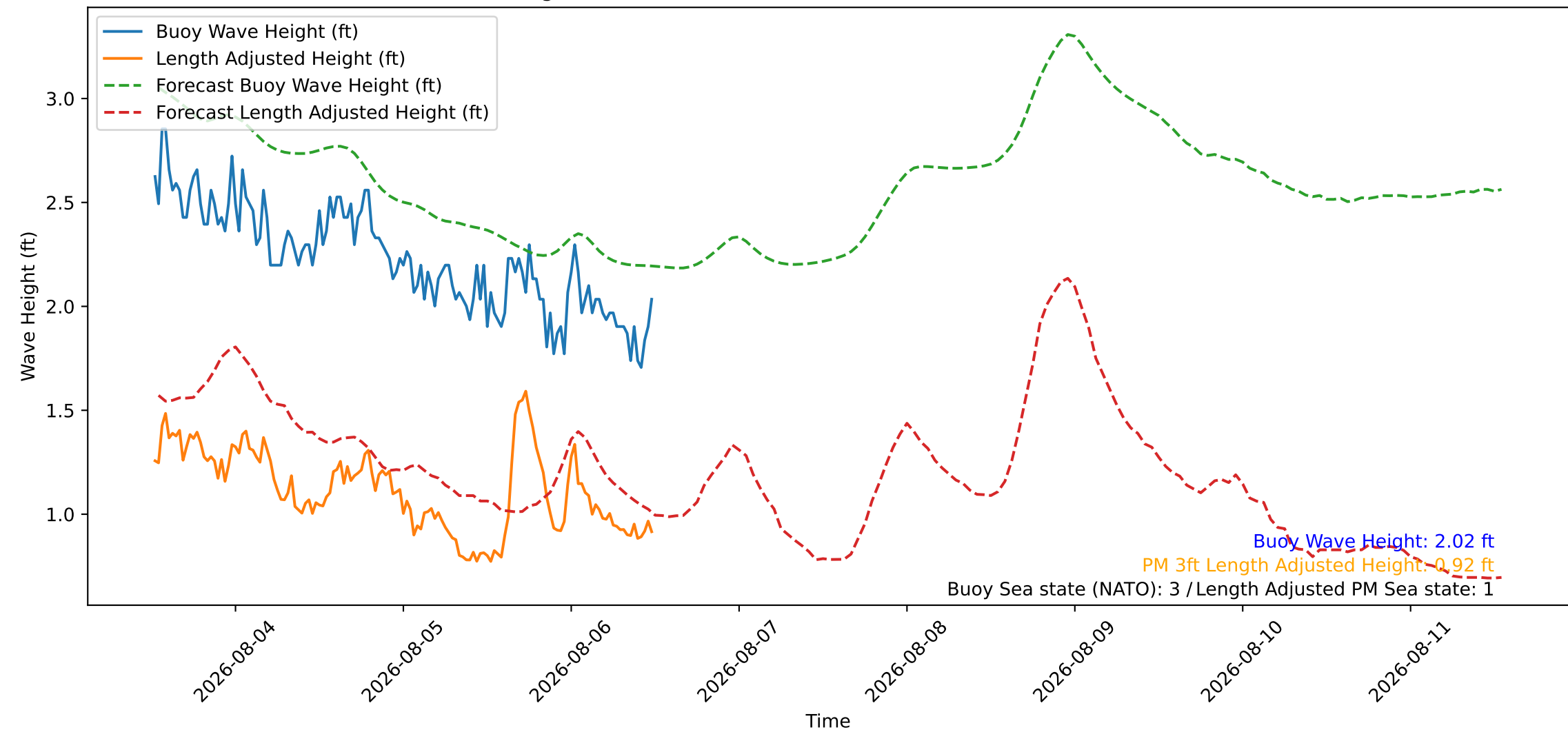
Wave Heights over Time for Oceanside Harbor at 2026-08-06 12:30:26
