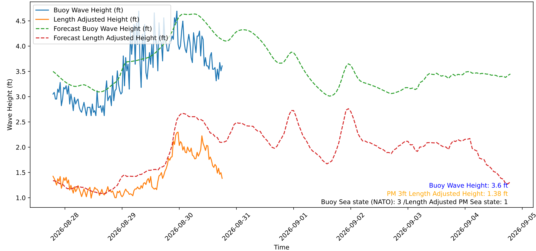
Wave Heights over Time for Red Beach at 2026-08-30 18:40:49
