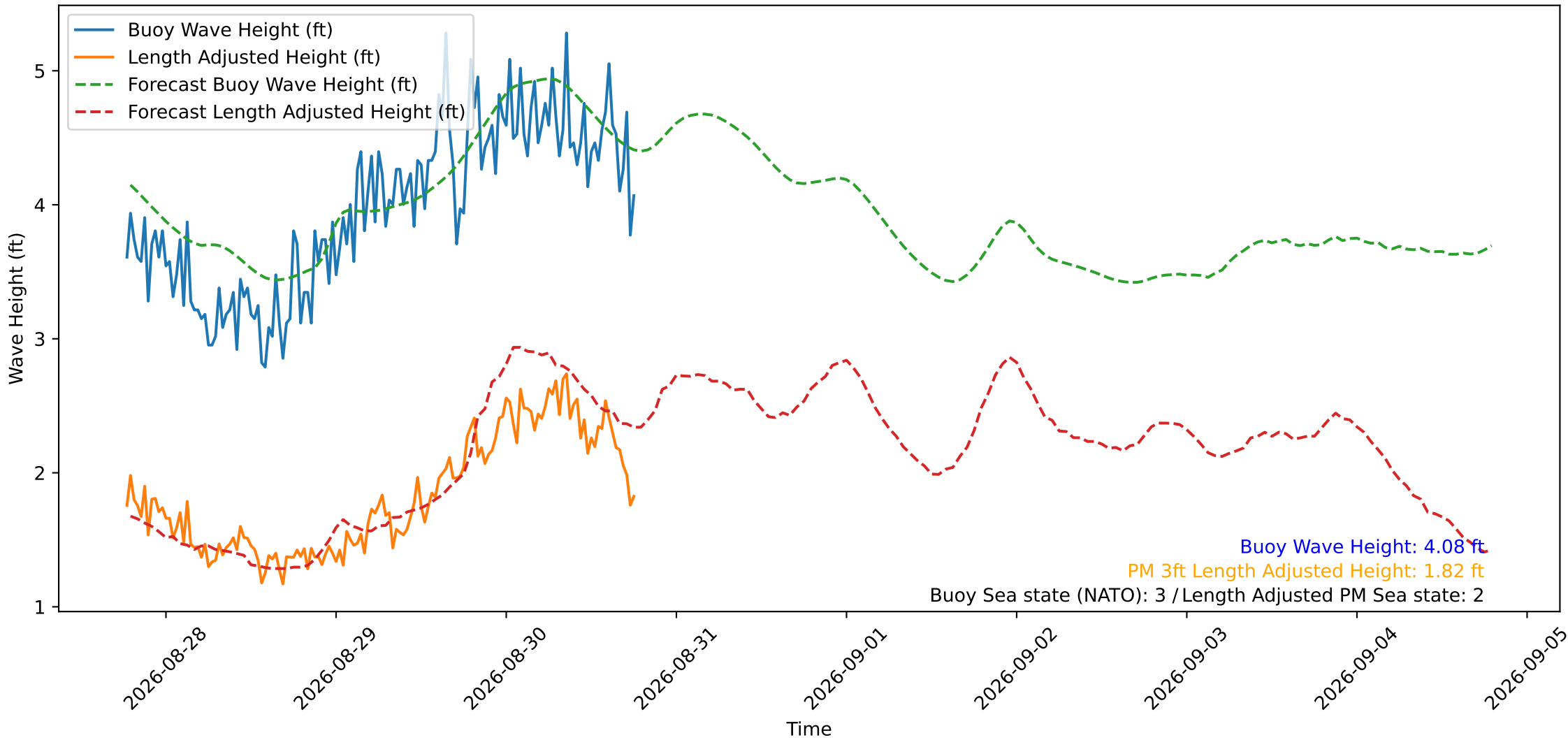
Wave Heights over Time for Oceanside Harbor at 2026-08-30 18:40:29
