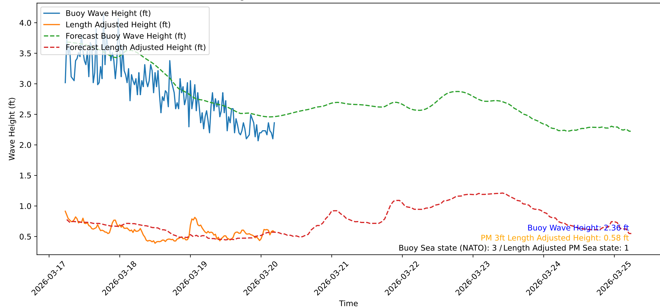
Wave Heights over Time for Green Beach at 2026-03-20 05:31:11
