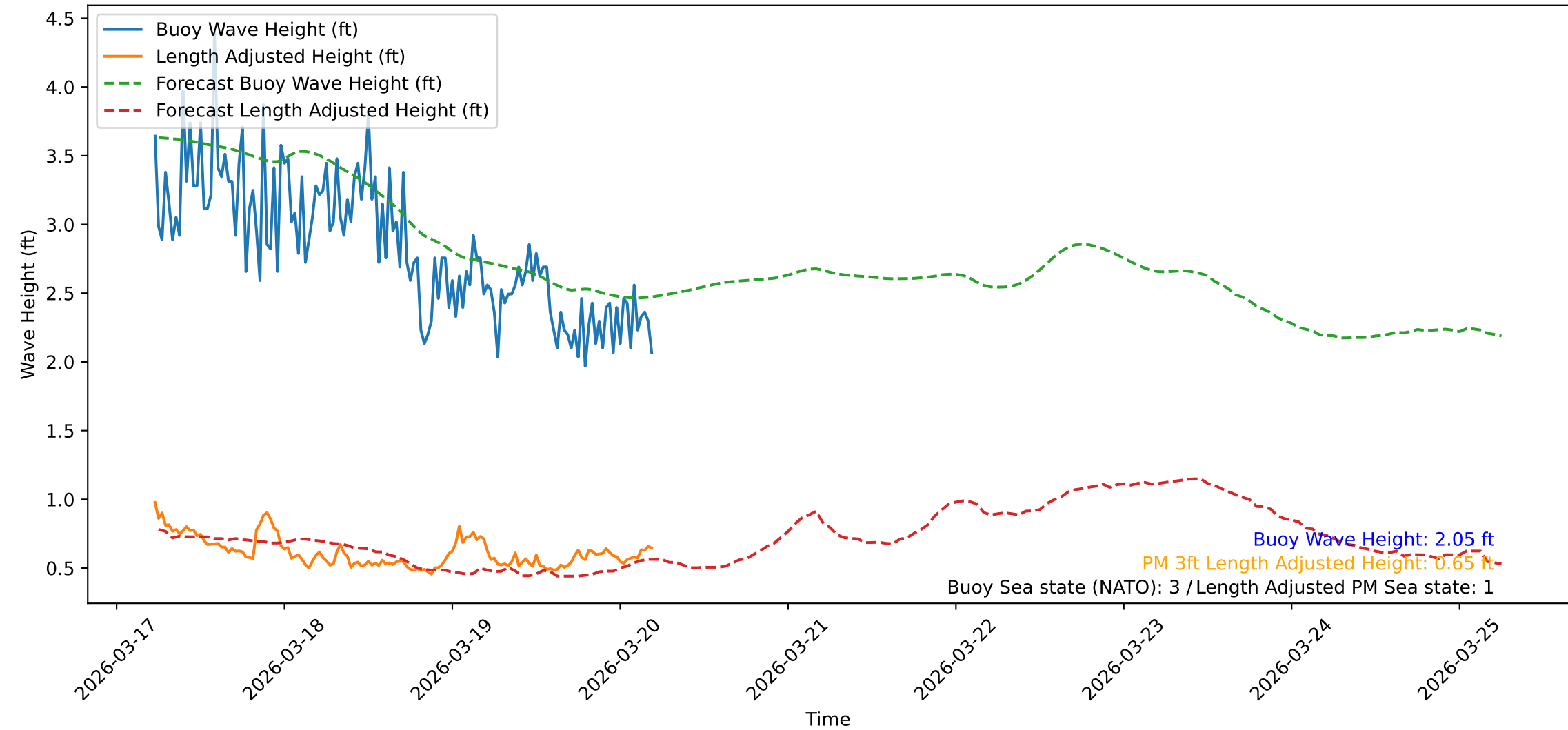
Wave Heights over Time for Oceanside Harbor at 2026-03-20 05:30:32
