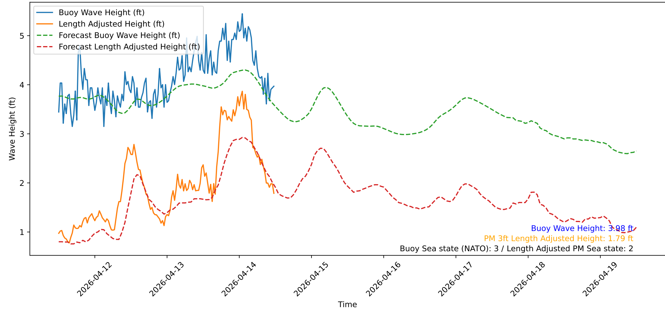
Wave Heights over Time for Oceanside Harbor at 2026-04-14 12:10:30
