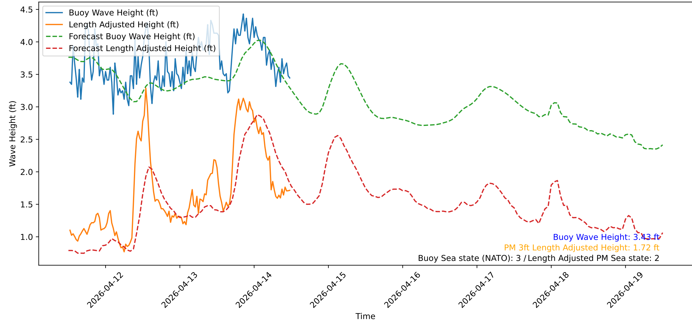
Wave Heights over Time for Red Beach at 2026-04-14 12:10:50
