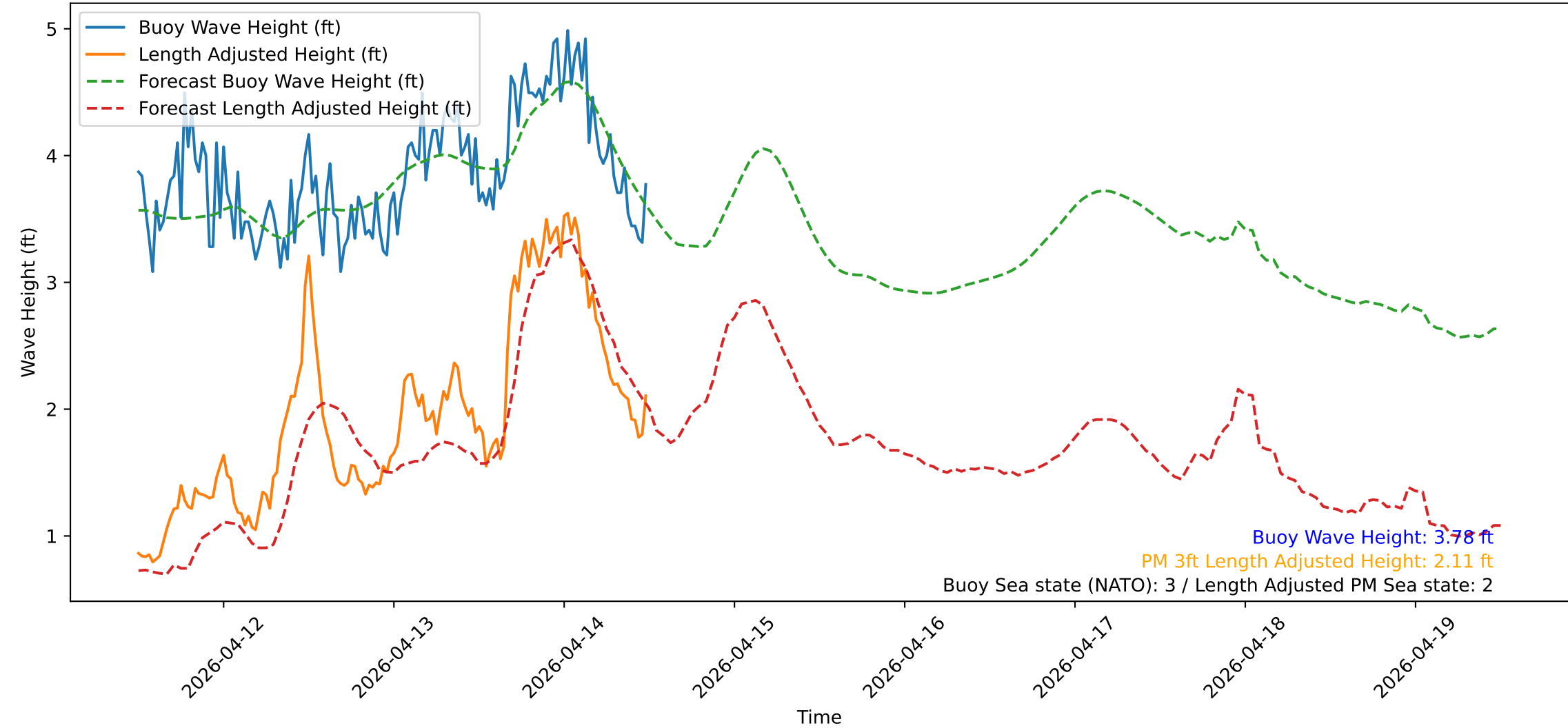
Wave Heights over Time for Green Beach at 2026-04-14 12:11:12
