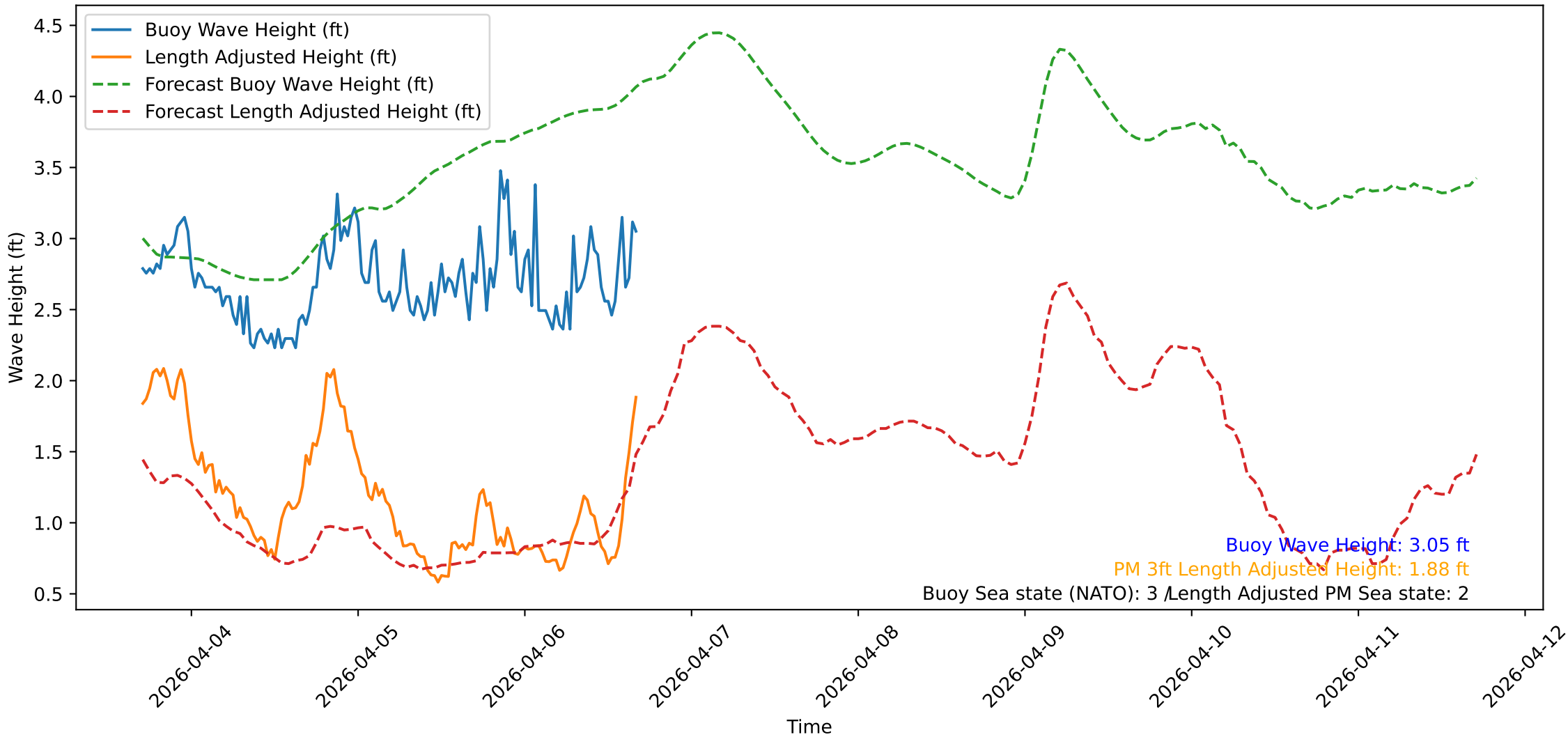
Wave Heights over Time for Green Beach at 2026-04-06 17:01:11
