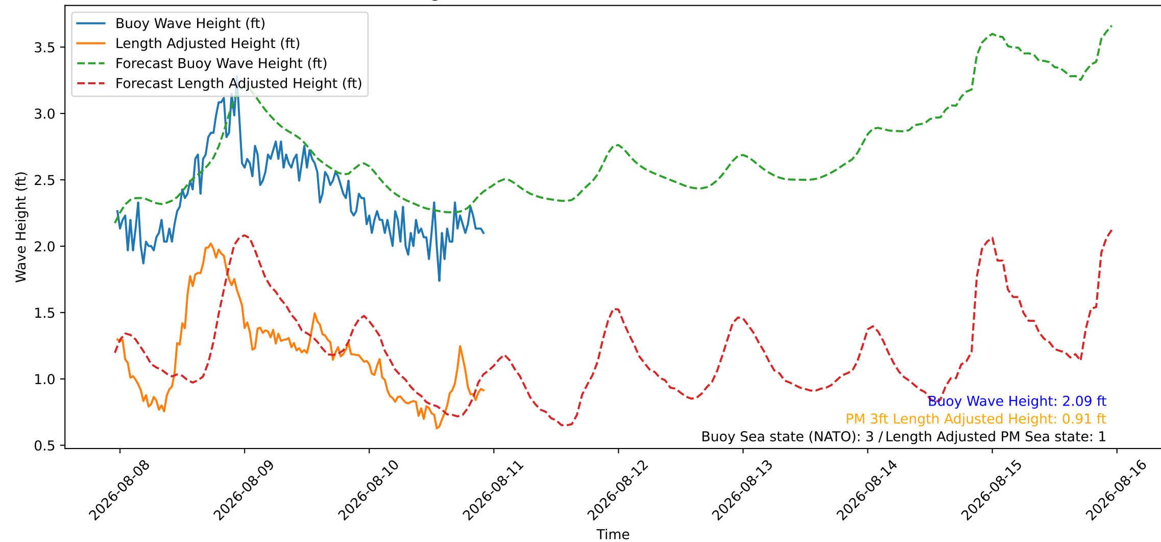
Wave Heights over Time for Red Beach at 2026-08-10 23:00:46
