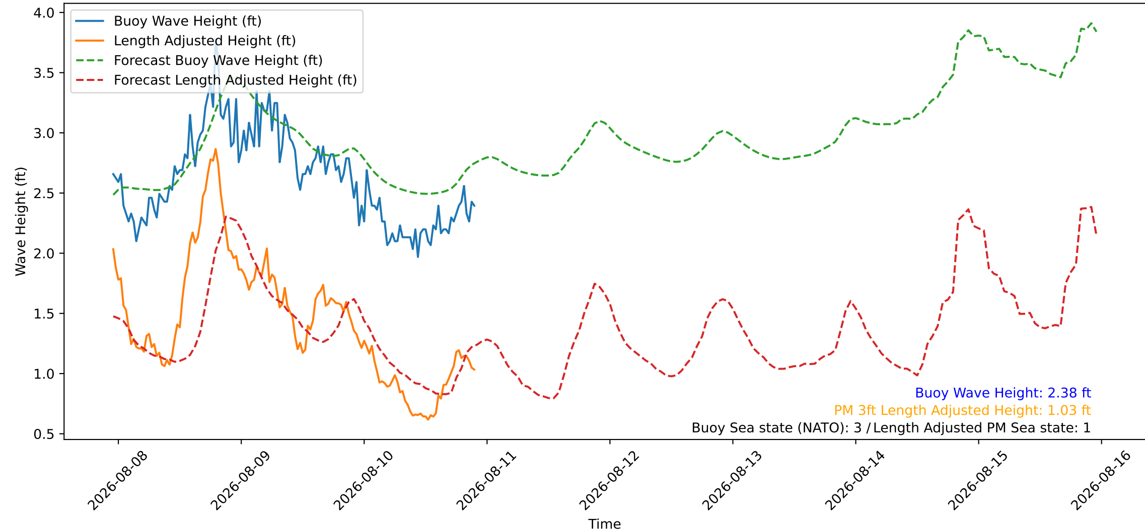
Wave Heights over Time for Green Beach at 2026-08-10 23:01:09
