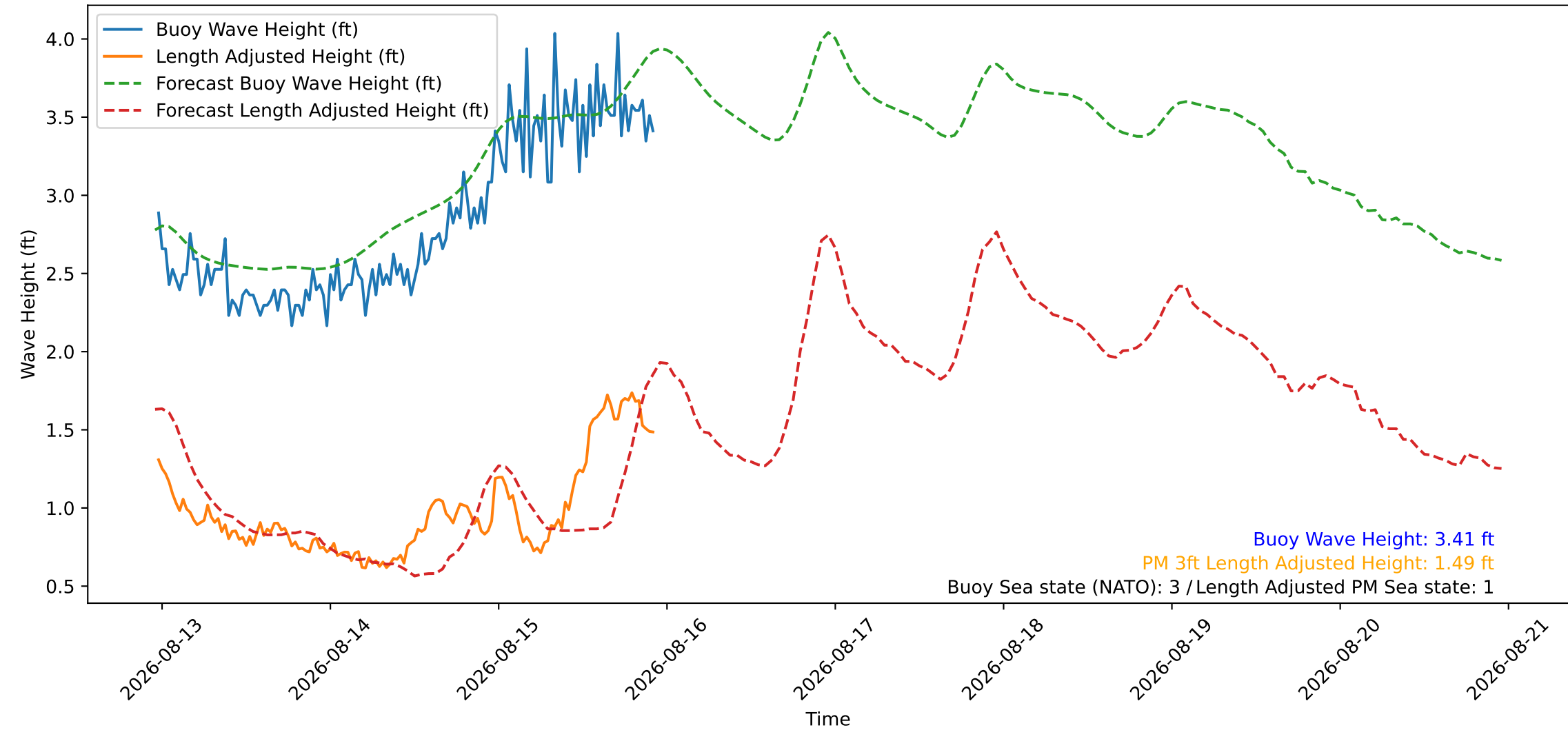
Wave Heights over Time for Red Beach at 2026-08-15 23:00:47
