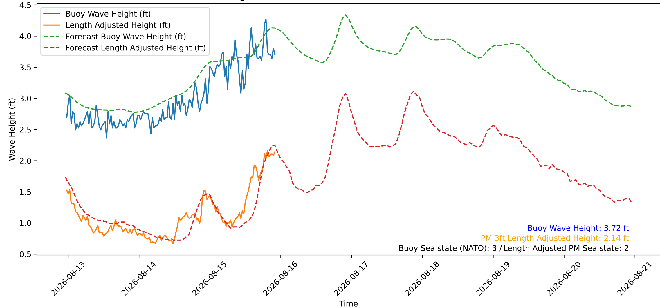
Wave Heights over Time for Green Beach at 2026-08-15 23:01:09
