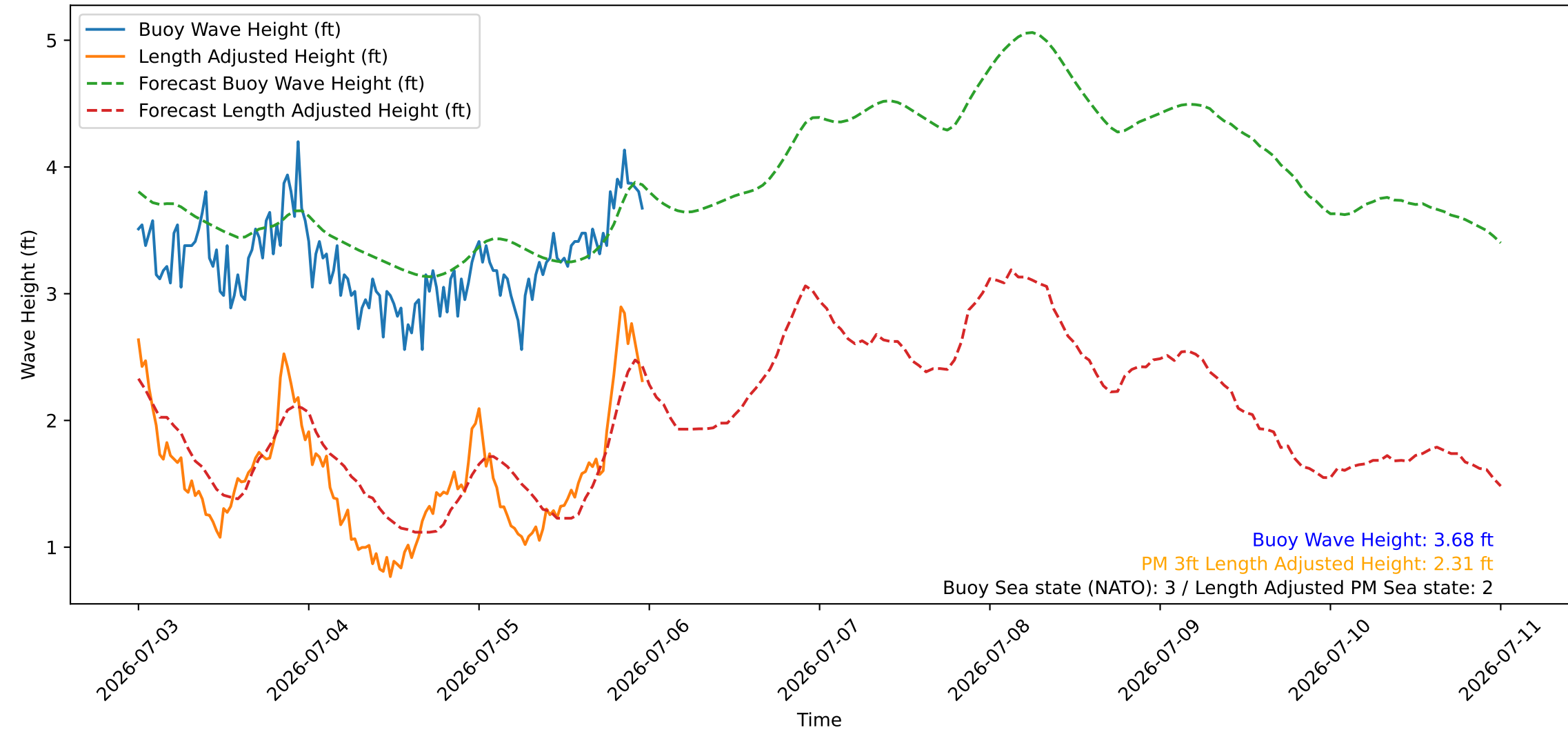
Wave Heights over Time for Green Beach at 2026-07-05 23:51:10
