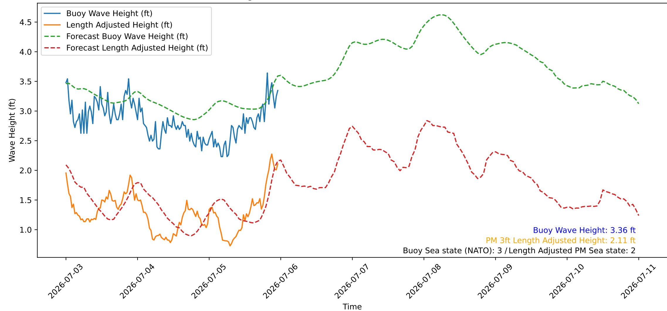
Wave Heights over Time for Red Beach at 2026-07-05 23:50:47
