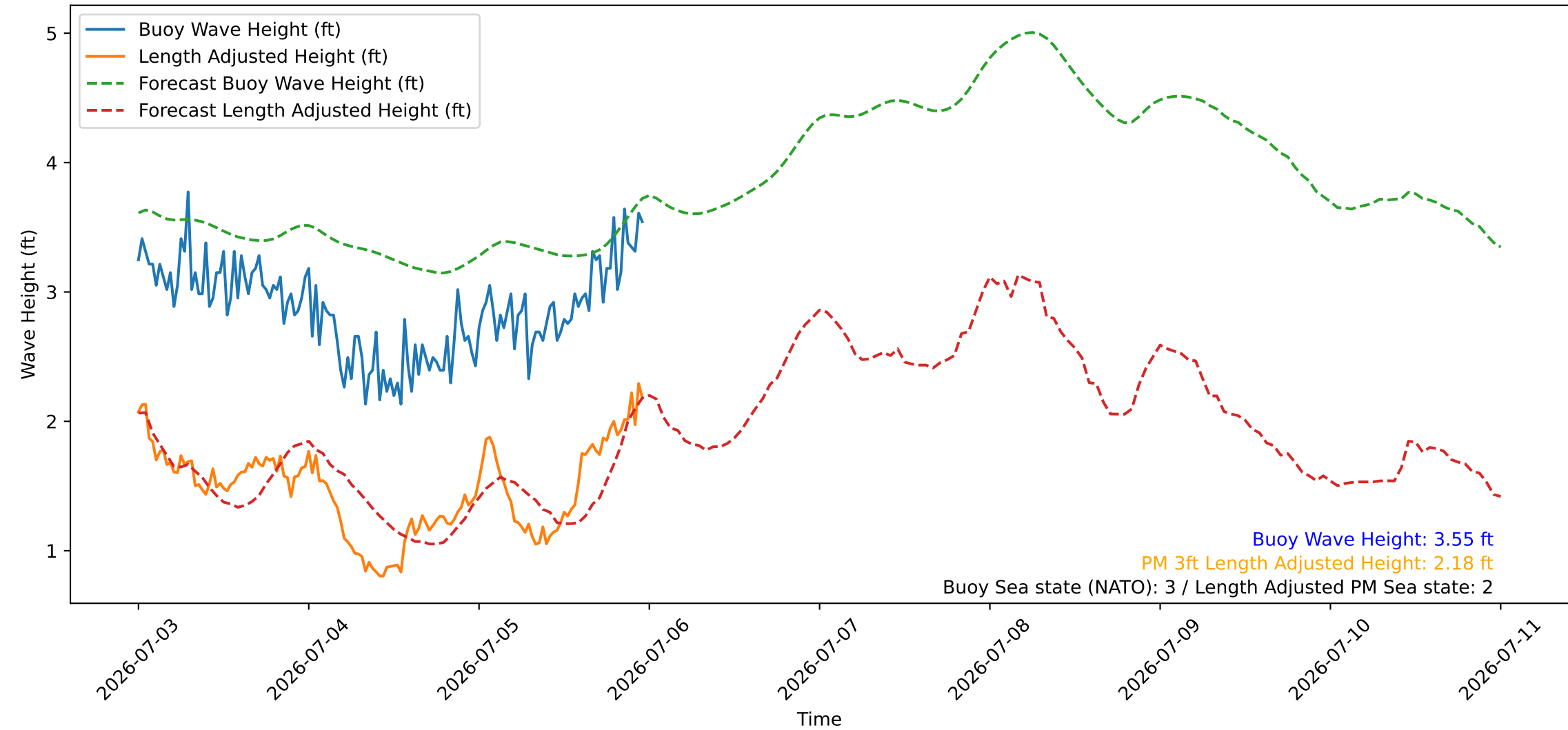
Wave Heights over Time for Oceanside Harbor at 2026-07-05 23:50:27
