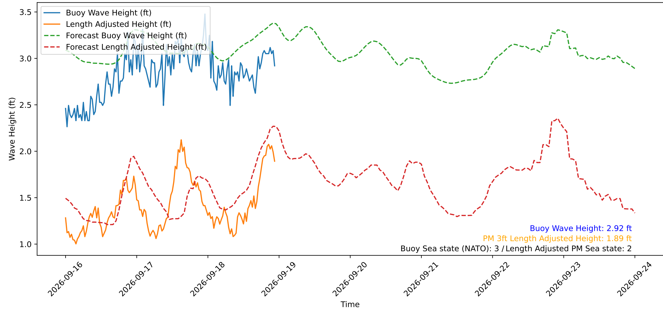
Wave Heights over Time for Green Beach at 2026-09-18 23:31:11
