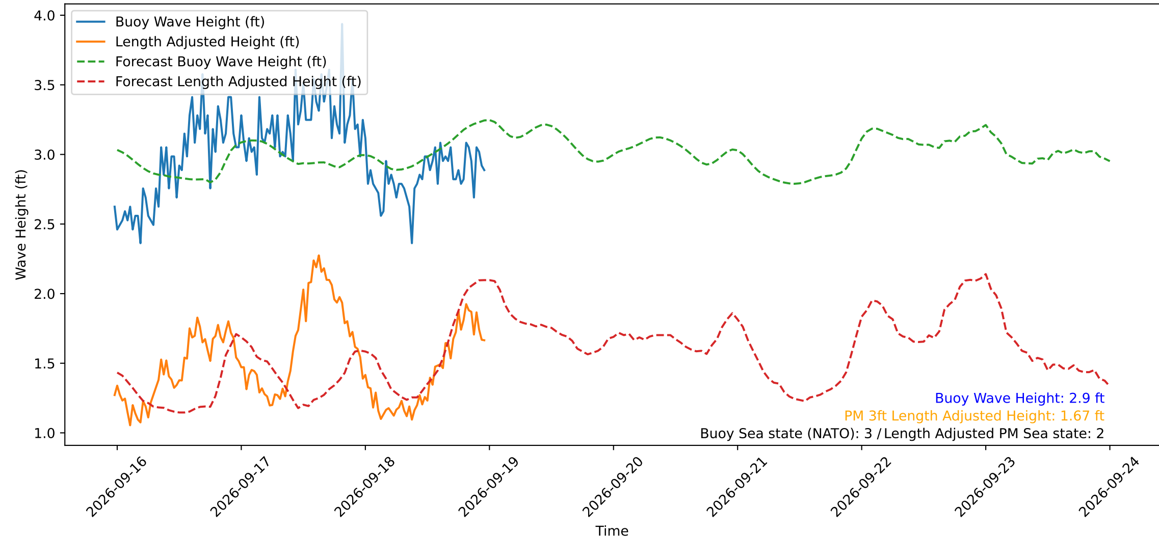
Wave Heights over Time for Oceanside Harbor at 2026-09-18 23:30:30
