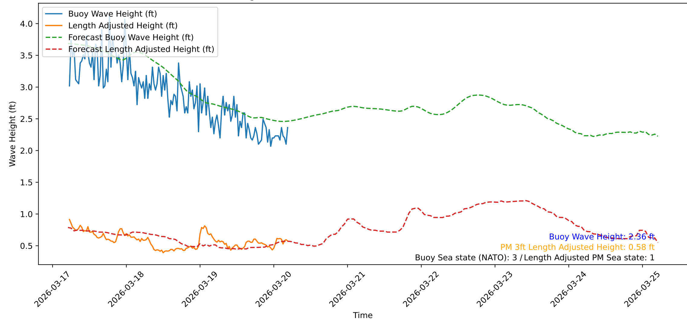
Wave Heights over Time for Green Beach at 2026-03-20 05:21:11
