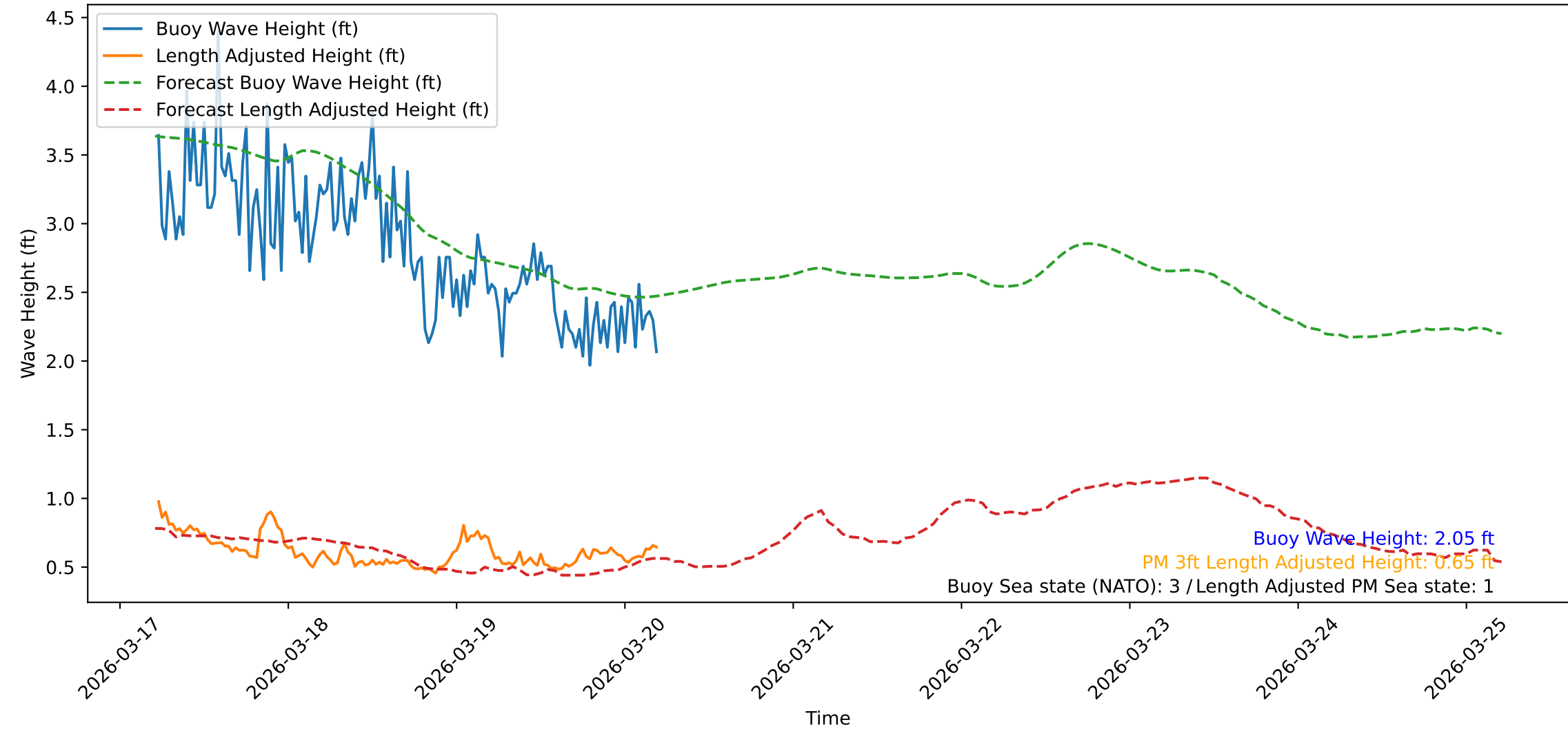
Wave Heights over Time for Oceanside Harbor at 2026-03-20 05:20:32
